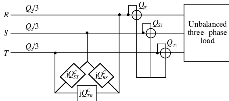
Fig. 3.- This compensator, formed by reactances, balances the system. Three wattmeters measure Q_{R1} , Q_{S1} and Q_{T1} , and allow to obtain which power values the compensator's reactances must absorb.
