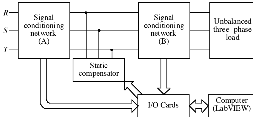
Fig. 8.- Block diagram of the experimental device.
