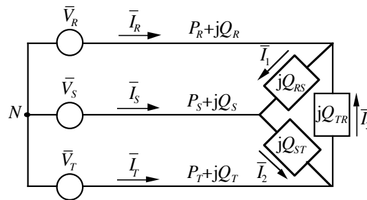
Fig. 2.- By choosing the appropriate value for Q_{RS} , Q_{ST} , and Q_{TR} , the reactive powers delivered by each phase, Q_R , Q_S , and Q_T , might be fixed at any desired value.
