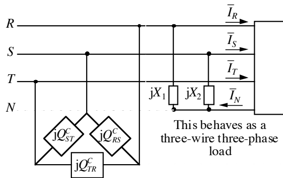
Fig. 6.- Static VAr compensator for a four-wire three-phase load.
