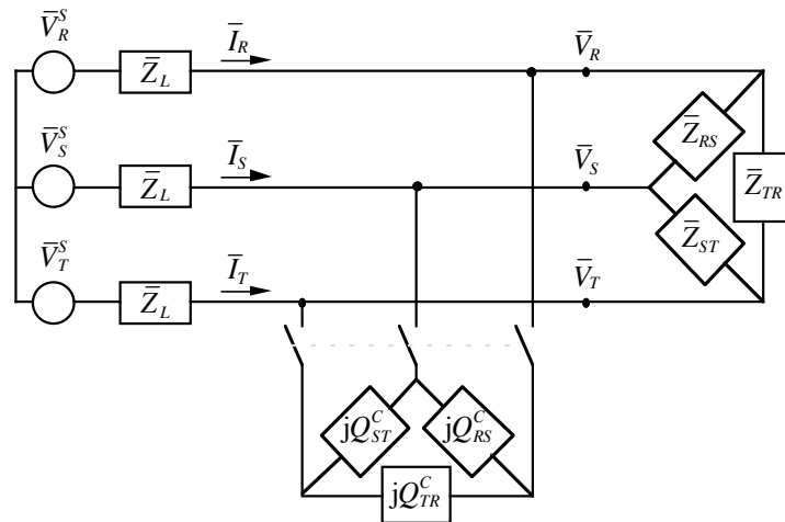
Fig. 7.- Simulation network.
