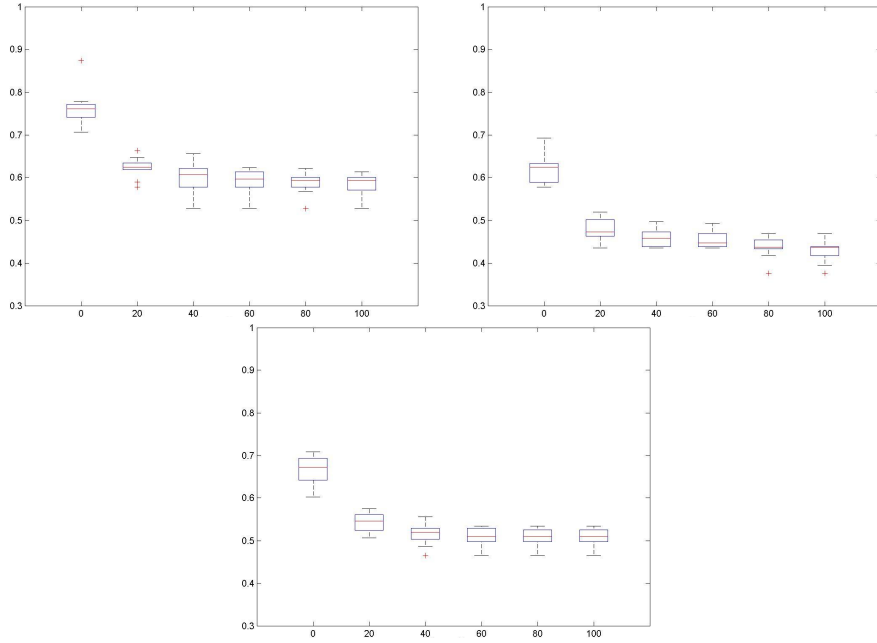
Fig. 5: Evolution of the MSE with the generations for the CC data set and the different CV methods. The top-left, top-right and bottom boxplots correspond with the 10-fold, 5x2 and LOO CV methods results.
