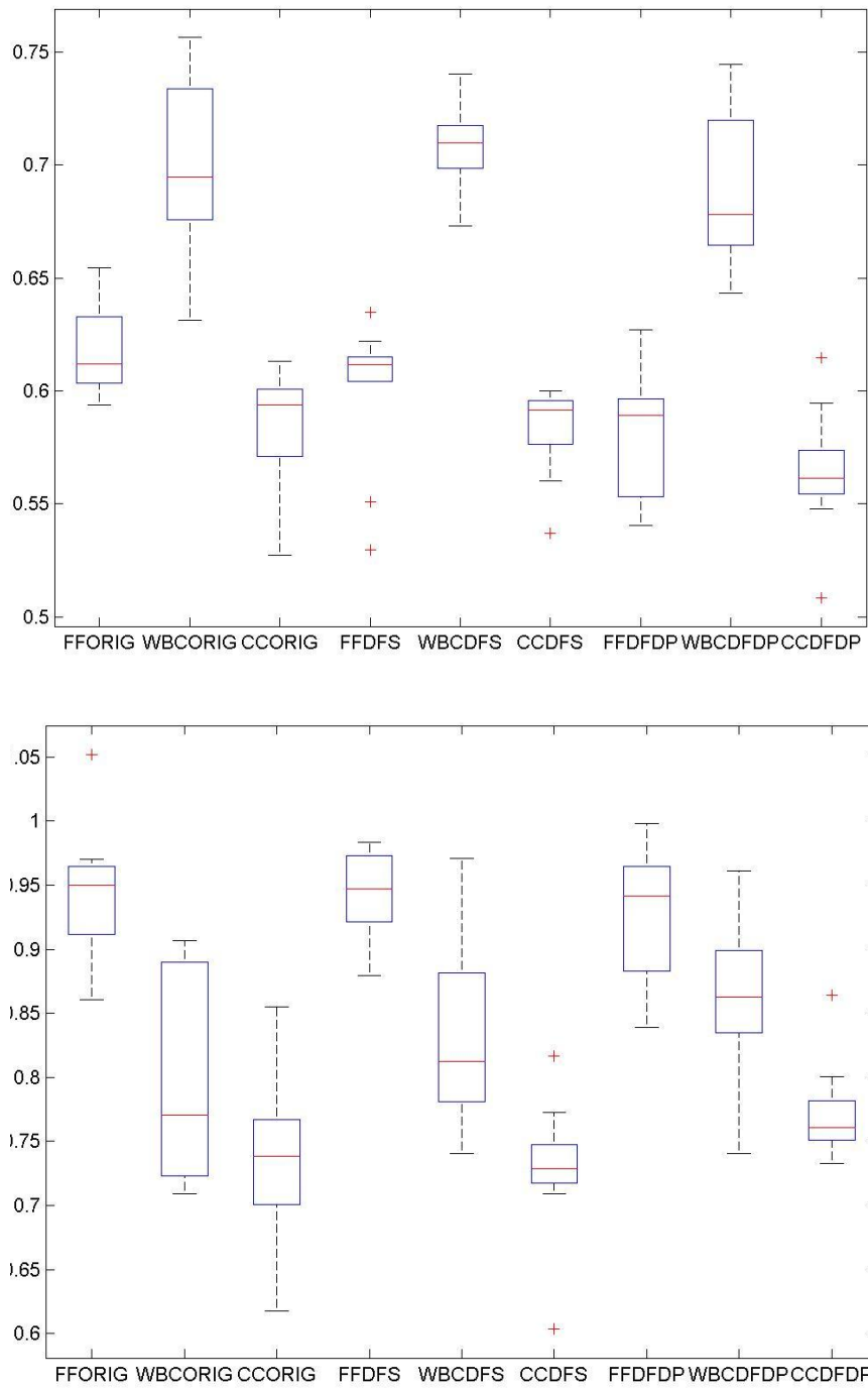
Fig. 6: Boxplot for the MSE values of the best individuals found for each data set and parameter combination -ORI, DFS and DF. On top, the box plot with the test subsets; on bottom, the box plots with the whole data set (both train and test sets).
