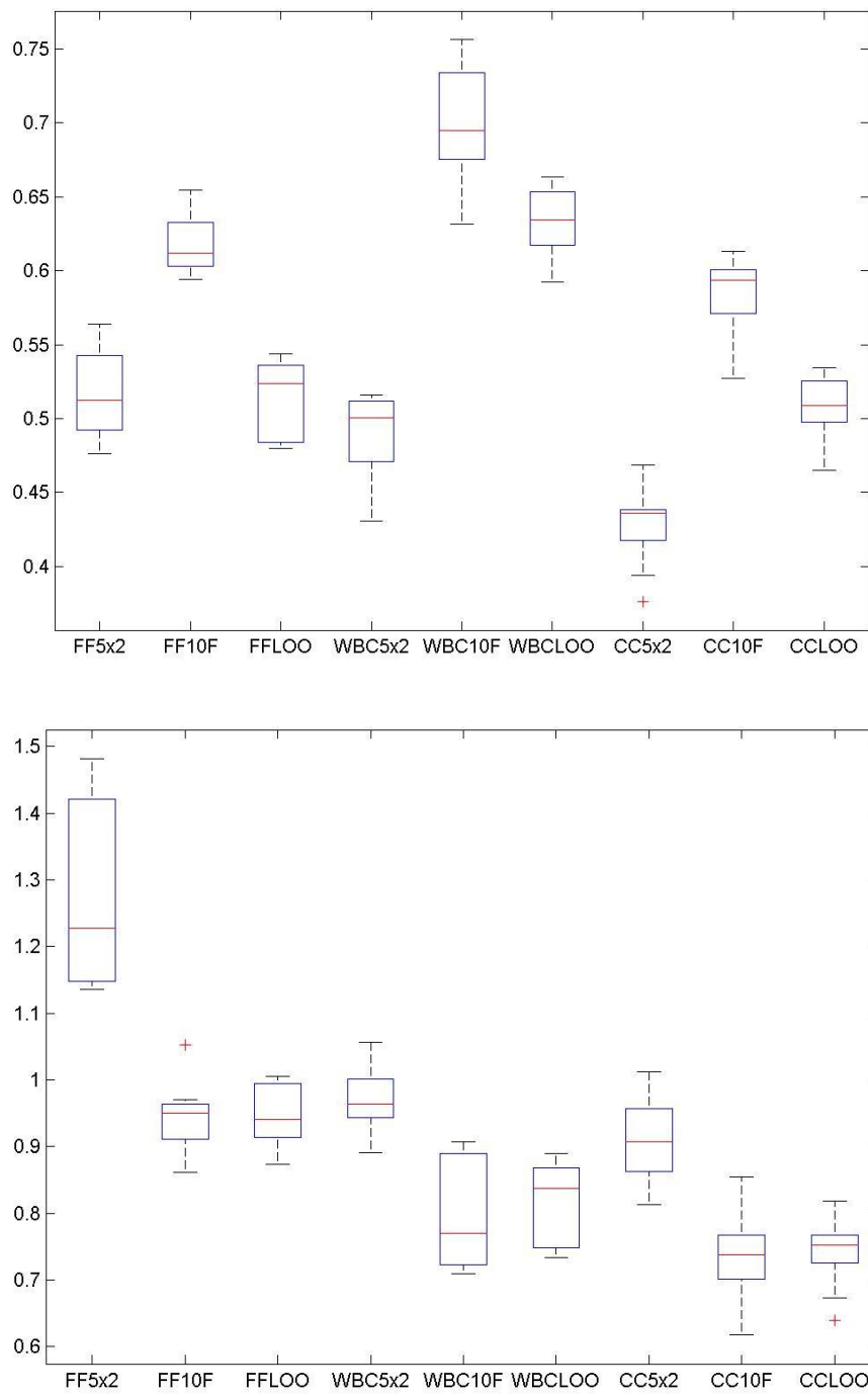
Fig. 2: Boxplot for the MSE values of the best individuals found for each data set. On top, the box plot with the test subsets; on bottom, the box plots with the whole data set (both train and test sets).
