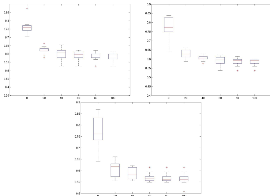
Fig. 9: Evolution of the MSE with the generations for the CC data set and the different options of parameter evolution. The top-left, top-right and bottom boxplots correspond with the ORI, the DFS and the DFDP options results.
