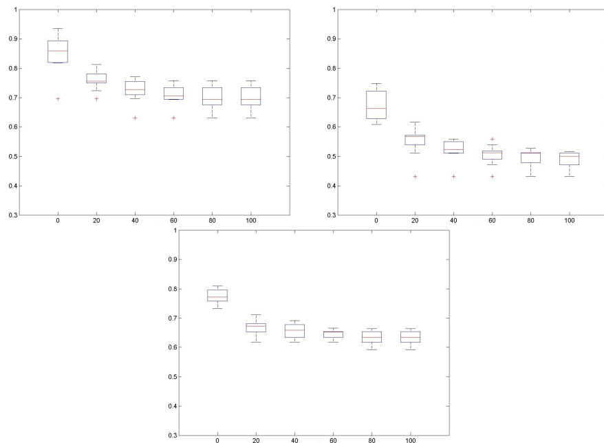
Fig. 4: Evolution of the MSE with the generations for the WBC data set and the different CV methods. The top-left, top-right and bottom boxplots correspond with the 10-fold, 5x2 and LOO CV methods results.
