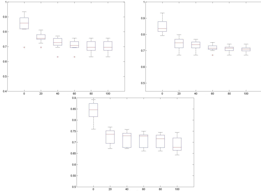
Fig. 8: Evolution of the MSE with the generations for the WBC data set and the different options of parameter evolution. The top-left, top-right and bottom boxplots correspond with the ORI, the DFS and the DFDP options results.
