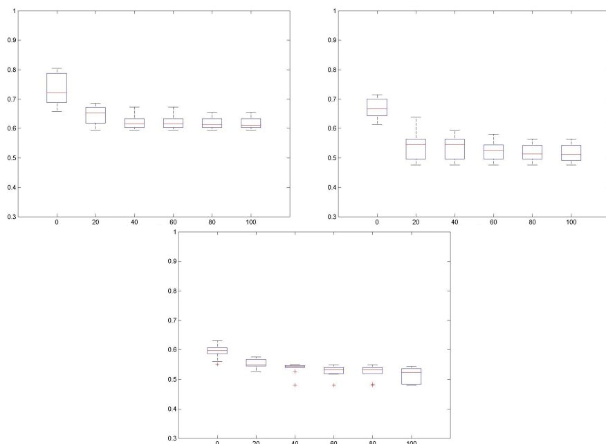
Fig. 3: Evolution of the MSE with the generations for the FF data set and the different CV methods. The top-left, top-right and bottom boxplots correspond with the 10-fold, 5x2 and LOO CV methods results.
