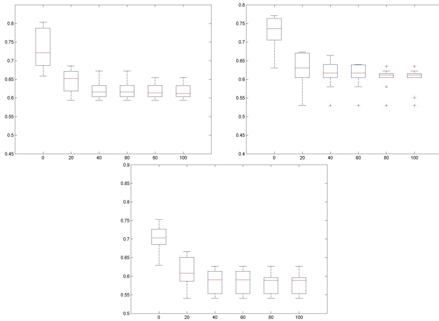
Fig. 7: Evolution of the MSE with the generations for the FF data set and the different options of parameter evolution. The top-left, top-right and bottom boxplots correspond with the ORI, the DFS and the DFDP options results.
