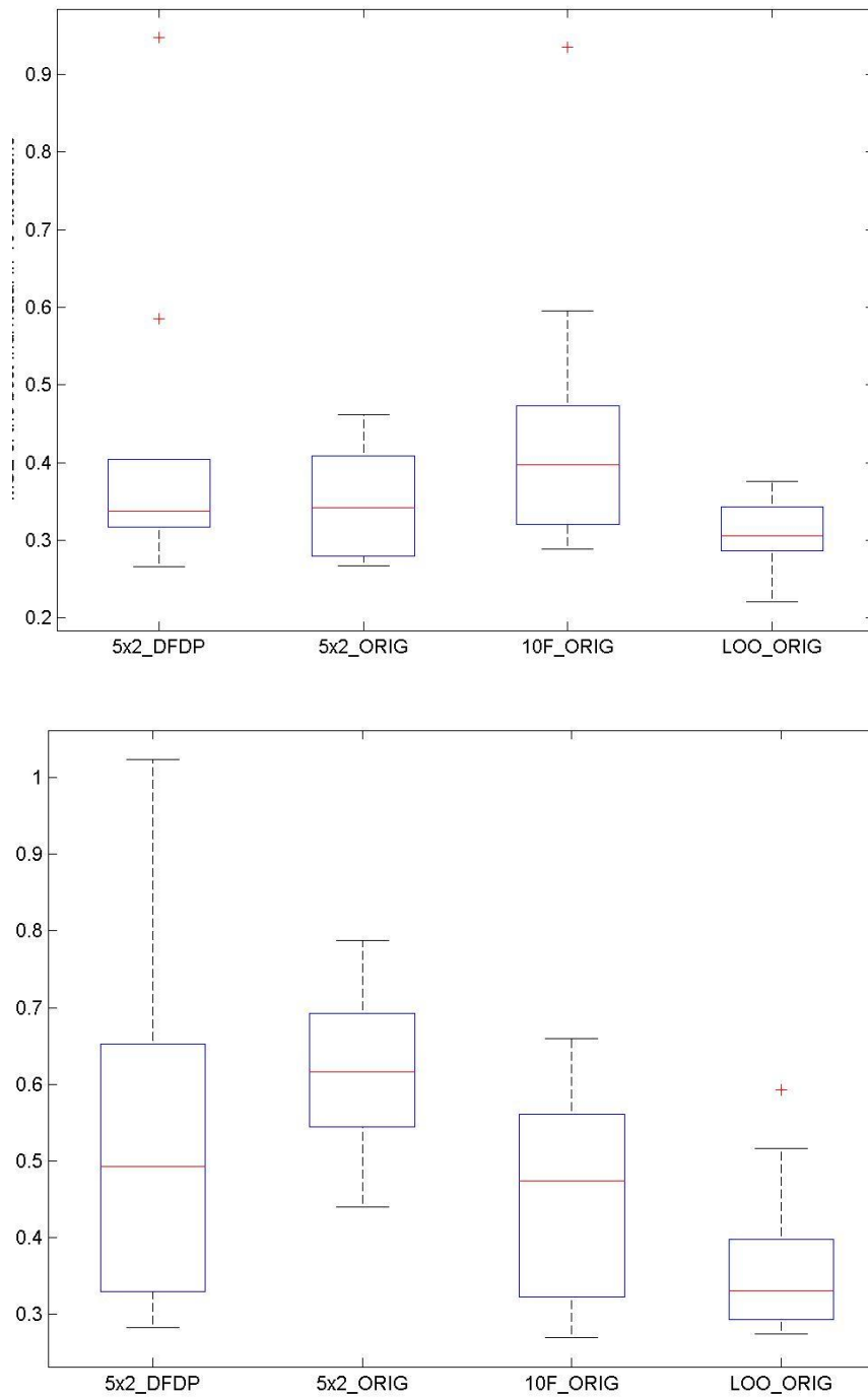
Fig. 10: Regression problem and NNs. Boxplot for the MSE values of the best individuals found for 5x2 DFDP, the 5x2, 10Fold and LOO CV for the original method. On top, the box plot with the test subsets; on bottom, the box plots with the whole data set (both train and test sets).
