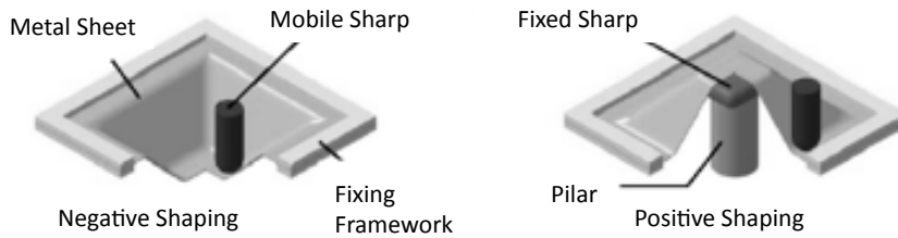
Fig. 1: The incremental cold shaping process of a steel sheet. A sharpening tool is iteratively applied onto the metal sheet at a different depth. In the negative shaping only the sharp tool is moved, while in the positive shaping both the metal sheet and the sharp tool are moved.
