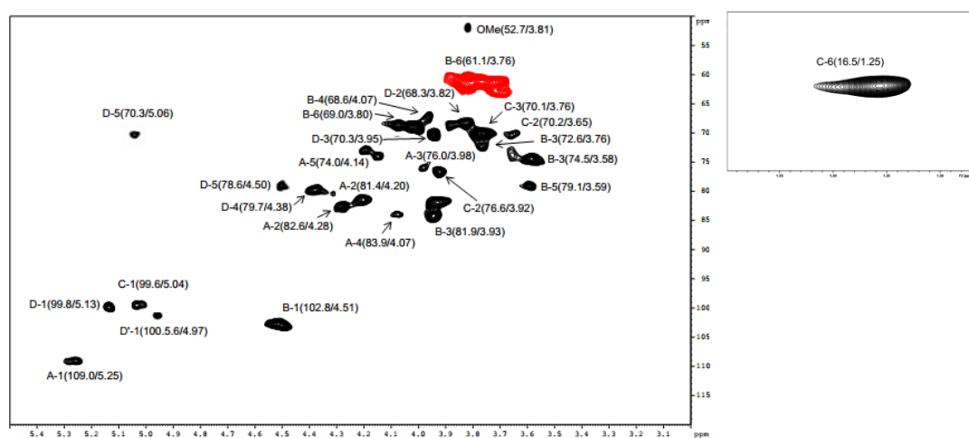
Fig. 4: ^1\text{H}/^{13}\text{C} HSQC NMR spectrum of FCF. Solvent \text{D}_2\text{O} at 30 ^\circ\text{C} ; numerical values are in \delta ppm. A ( \alpha -L-Araf); B ( \beta -D-Galp); C ( \alpha -L-Rhap); D ( \alpha -D-GalpA); D' (6-OMe- \alpha -D-GalpA). The letters are followed by the carbon number of the monosaccharide unit. Chemical shifts were determined by HSQCed, COSY, TOCSY and HMBC experiments.
