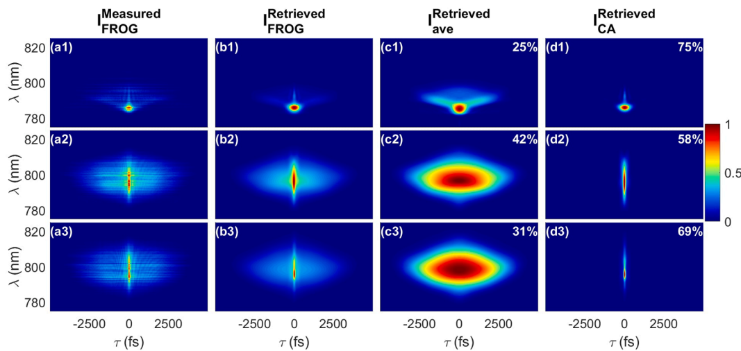
Fig. 6. FROG reconstruction measured in the same configuration but with different I_p from top to bottom: 250 mA, 500 mA and 750 mA. Experimental (column a), reconstructed (column b), average pulse (column c), and CA (column d) FROG traces for each pumping intensity. Note that all traces are individually normalized to maximum unity.
