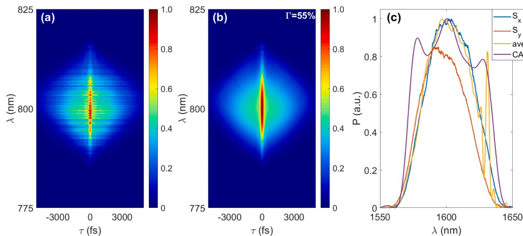
Fig. 8. Complete measurement of I_p = 550 mA. (a) Experimental FROG trace. (b) Reconstructed FROG trace with \Gamma = 55\% . (c) Spectral comparison of the horizontal ( S_x ) and vertical ( S_y ) projections of the vector pulse measured with the OSA and the spectra retrieved for the average (ave) and coherent artifact pulses (CA).
