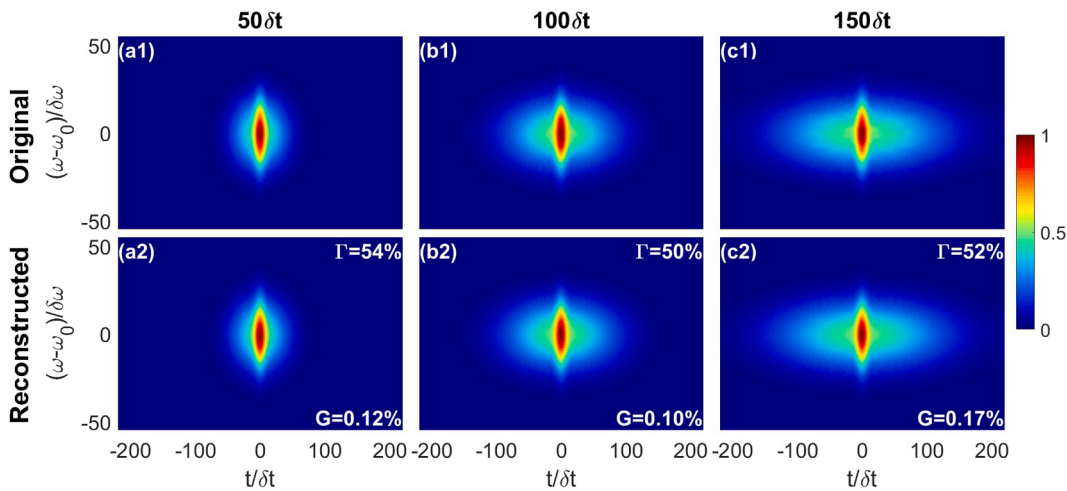
Fig. 4. Numerical test of the modified PCGPA algorithm for a seed of 10\delta t (FWHM) with different values of the FWHM temporal width of the temporal gaussian envelope: (a) 50\delta t ; (b) 100\delta t ; (c) 150\delta t . First row represents the original FROG trace calculated from the unstable train. Second row shows the reconstructed FROG traces using the modified PCGPA for each case.
