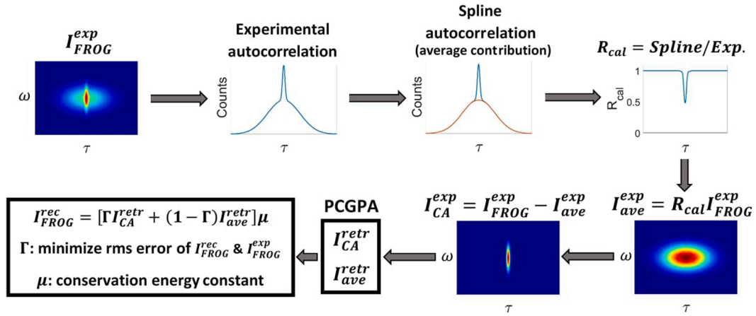
Fig. 3. Diagram of the modified PCGPA algorithm for the reconstruction of double structured FROG traces.
