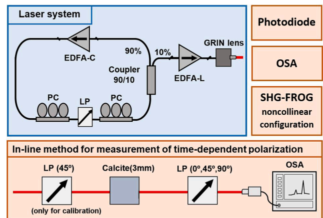
Fig. 1. Scheme of the experimental set-up: laser source (blue background) and characterization systems (orange background). The characterization systems are: photodiode for the direct observation of the pulse train, Optical Spectrum Analyser (OSA) for the spectra measurement, noncollinear SHG-FROG for temporal characterization and the in-line method for measurement of time-dependent polarization of ultrashort pulses.
