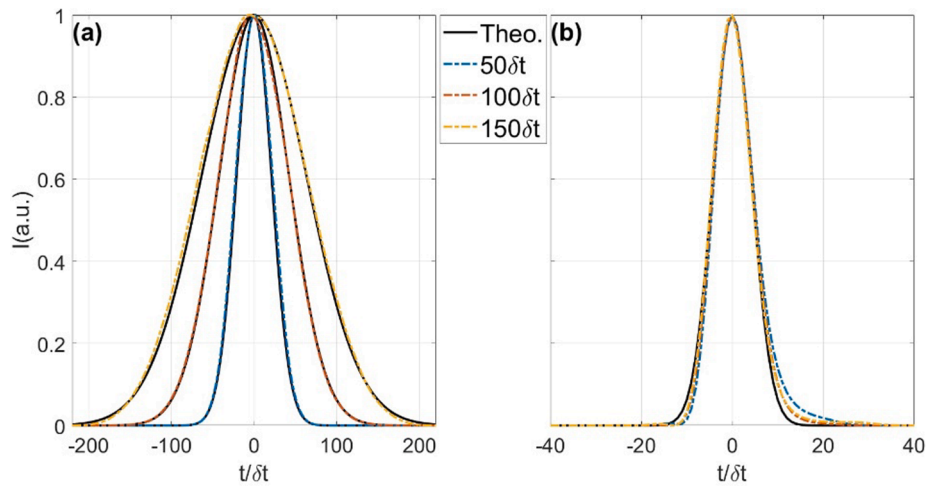
Fig. 5. Numerical comparison of the temporal evolution. (a) Average reconstruction compared with the wide gaussian envelope (Theo.) for each case. (b) CA reconstruction compared with the seed (Theo.) used to create the unstable pulse train.
