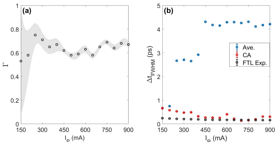
Fig. 7. Evolution of parameters as a function of the pumping intensity of the amplification stage, I_p . (a) Weight of the CA on the reconstructed traces, \Gamma . (b) Temporal width (FWHM) of the average (blue), CA (red) and Fourier Transform Limit of the experimental spectrum (black). (For interpretation of the references to colour in this figure legend, the reader is referred to the web version of this article.)
