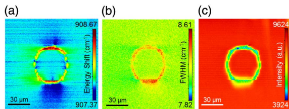
Fig. 2. Micro-Raman mapping of the facet cross section of the fs-DLW circular-cladding Tm:KLuW waveguide (W2) measuring the high gain 907 \text{cm}^{-1} phonon mode: (a) phonon energy shift, (b) full width at half-maximum, and (c) peak intensity.
