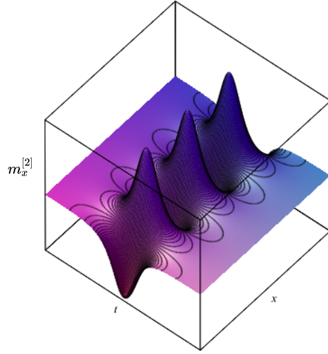
Figure 2.3: Akhmediev breather m_x^{[2]} for NLS system, with parameters h_0 = 1, A_1 = 4 .
