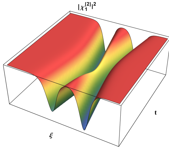
Figure 3.2: Two-soliton solution for the upper component \left|\chi_1^{[2]}\right|^2 . Parameters are g = 2 , \theta_0 = 0.5 , \theta_1 = 1 , \theta_2 = 1.2 , s = 1 , j_0 = 1 , and a_1 = a_2 = 1 .
