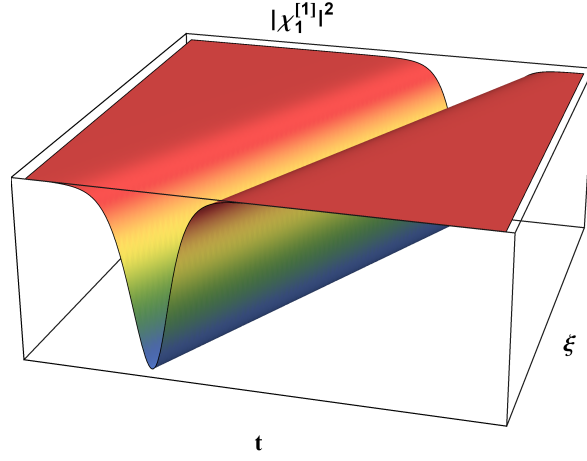
Figure 3.1: One-soliton solution for the upper component \left|\chi_1^{[1]}\right|^2 , with parameters g = 2 , \theta_0 = 0.5 , \theta_1 = 1 , s = 1 , j_0 = 1 , a_1 = 1 .
