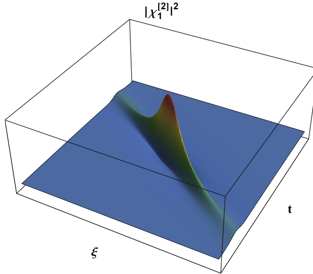
Figure 3.5: Generalization of the Peregrine soliton \left|\chi_1^{[2]}\right|^2 with parameters g = -2 , \theta_0 = 0.5 , \theta_1 = 0 , \theta_2 = \pi , s = 1 and h_0 = 1.5 .
