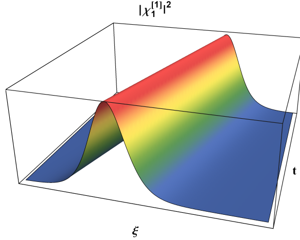
Figure 3.7: Generalization of the Davydov soliton |\chi_1|^2 with parameters g = -2 , \theta_0 = 0.5 , s = 1 and c = -\frac{1}{4} .
