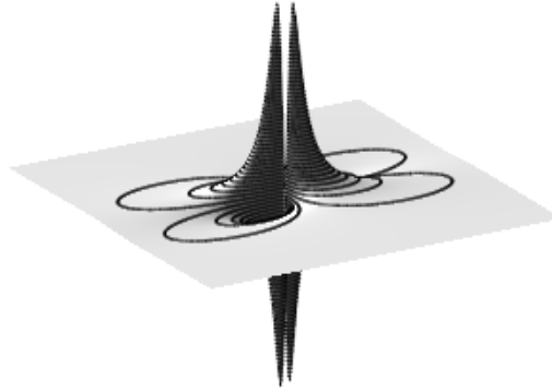
Figure 4.1: One-soliton solution of type 0+0 , m_y^{[2]} , with \beta_1 = 1, \beta_2 = 1 , a_1 = \frac{1}{2} , b_1 = \frac{1}{2} .
