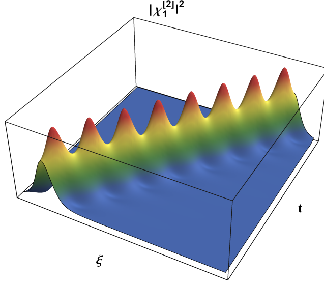
Figure 3.4: Generalization of the Kuznetsov-Ma breather \left|\chi_1^{[2]}\right|^2 with parameters g = -2 , \theta_0 = 5 , \hat{\theta}_1 = -2 , s = 1 , h_0 = 3 .
