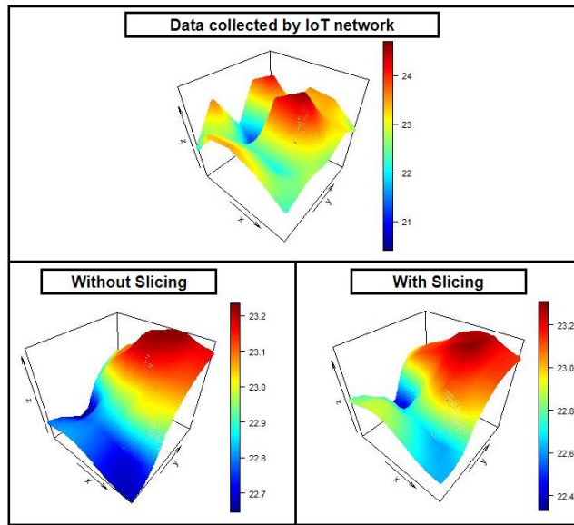
Figure 8: The results obtained by the data quality algorithm are compared using the technique proposed in this article and without using the technique.
