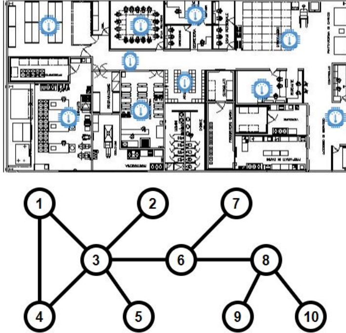
Figure 2: Illustrative example of the construction of a graph based on the position of the IoT nodes on a map.
