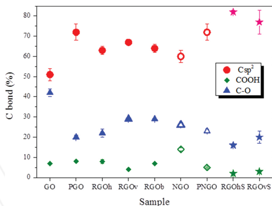
Figure 3. Chemical composition of graphene oxides determined by XPS measurements. Data were taken from references [17–19]. Solid symbols correspond to graphene oxides obtained from graphite and open symbols from GANF® nanofibers. Stars are results of surfactant-functionalized graphene oxides.
