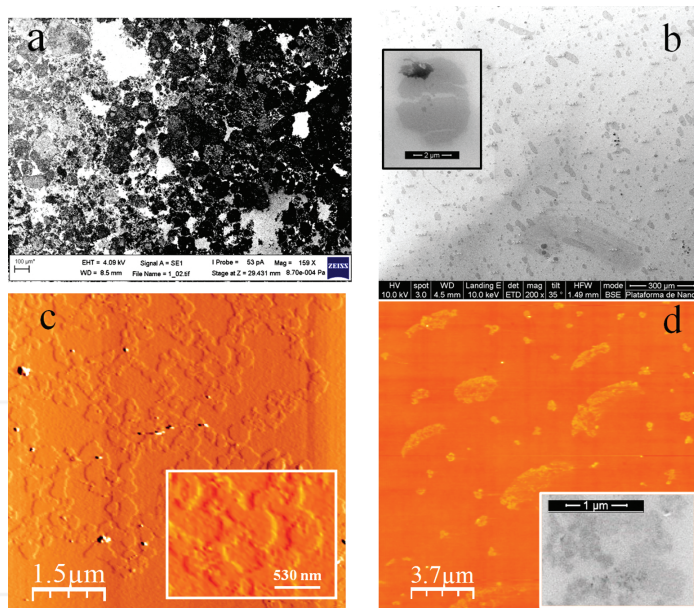
Figure 5. Representative images of different graphene oxides films: (a) SEM image of graphene oxide obtained by oxidation of graphite; (b) TEM image of graphene oxide reduced by vitamin C. The inset is a magnification to show the morphology of RGOv nanoplatelets; (c) graphene oxide functionalized with DDPS and reduced by hydrazine. The inset shows a magnification of the AFM image; (d) graphene oxide functionalized with DDPS and reduced by vitamin C. The inset is a TEM image to show details of the film morphology. Reduced graphene oxides were obtained using graphite as starting materials. The surface pressure of the Langmuir monolayer precursor of the LB film was 1 \text{ mN m}^{-1} .
