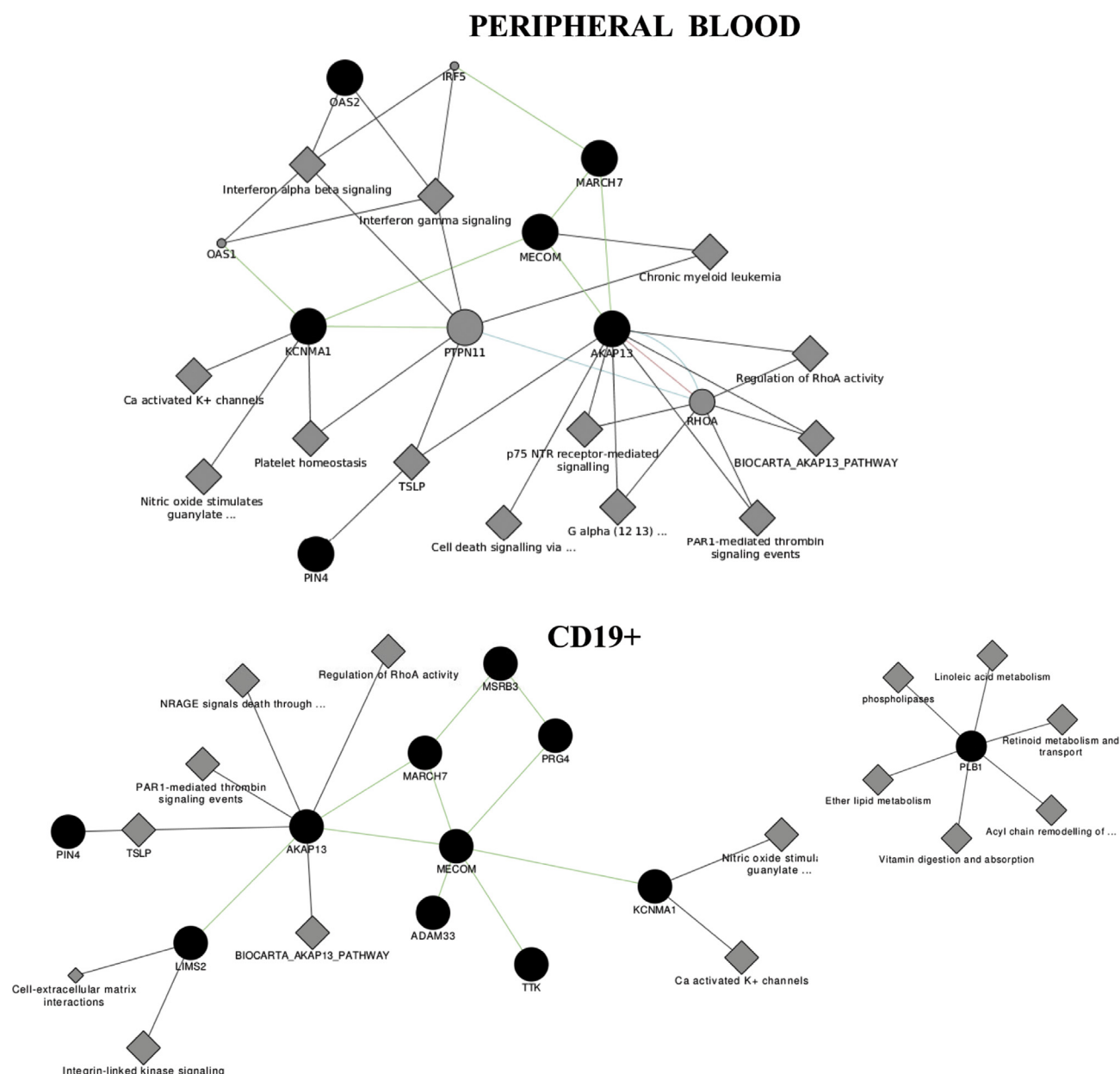
Fig. 4. Functional relations of Y.RNA.269-201 (ENSG00000201555) potential targets. GeneMANIA algorithm prediction. Black circles represent gene targets. Grey circles represent associated genes to network inference. Grey rhombuses represent pathways. The green edges represent genetics relationship. Pink and blue edges represent to protein-protein interaction.
