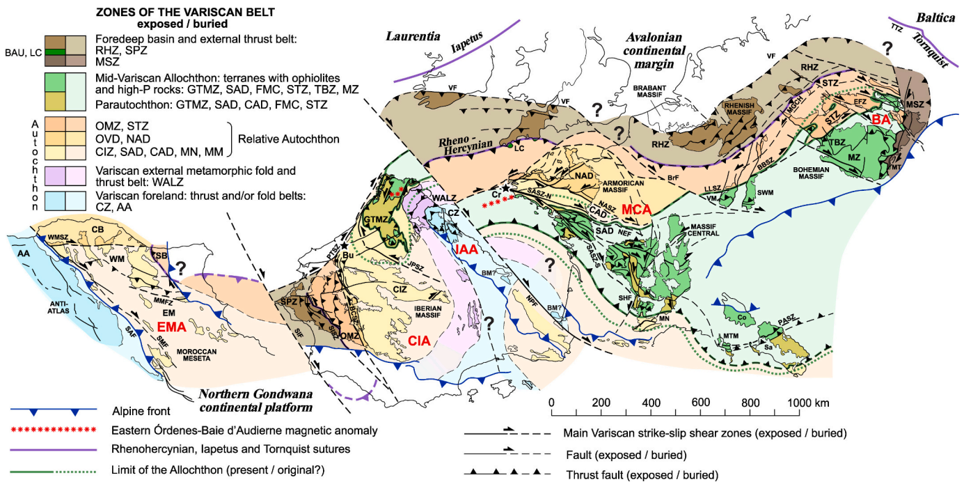
Fig. 1. Sketch of the Variscan belt in an early Permian reconstruction that postdates ductile and brittle transcurrent. Zones (Z): CZ, Cantabrian; CIZ, Central Iberian (OVD, Obejo-Valsequillo Domain); GTMZ, Galicia-Trás-os-Montes; MSZ, Moravo-Silesian; MZ, Moldanubian; OMZ, Ossa-Morena; RHZ, Rhenohercynian; SPZ, South Portuguese; STZ, Saxo-Thuringian; TBZ, Teplá-Barrandian; WALZ, West Asturian-Leonese. Armorican Domains (AD): CAD, Central; NAD, North; SAD, South; MM: Moroccan Meseta (AA, Anti-Atlas; CB, Coastal Block; EM, Eastern Meseta; SB, Sehouli Block; WM, Western Meseta). Shear zones (SZ), faults (F) and fault zones (FZ): BBSZ, Baden-Baden; BCSZ, Badajoz-Córdoba; BrF, Bray; EFZ, Elbe; JPSZ, Juzbado-Penalva; LLSZ, Lalaye-Lubine; MMFZ, Middle Meseta; MT, Moldanubian Thrust; NASZ, North Armorican; NEF, Nort-sur-Erdre; NPF, North Pyrenean; PASZ, Posada-Asinara; PTSZ, Porto-Tomar; SAF, South Atlas; SASZ, South Armorican (N and S, northern and southern branches); SHF, Sillon Houlier; SIF, South Iberia; SISZ, Southern Iberian; SMF, South Meseta; IAA, Ibero-Armorican; MCA, Massif Central. Other: BAU, Beja-Acebuches Unit; BM, Basque Massifs; Bu, Buçaco; Co, Corsica; Cr, Crozon. FMC, French Massif Central; LC, Lizard Complex; MTM, Maures-Tanneron Massif; MGCH, Mid-German Crystalline High; MN, Montagne Noire; Sa, Sardinia; SWM, Schwarzwald Massif; VM, Vosges Massif.
