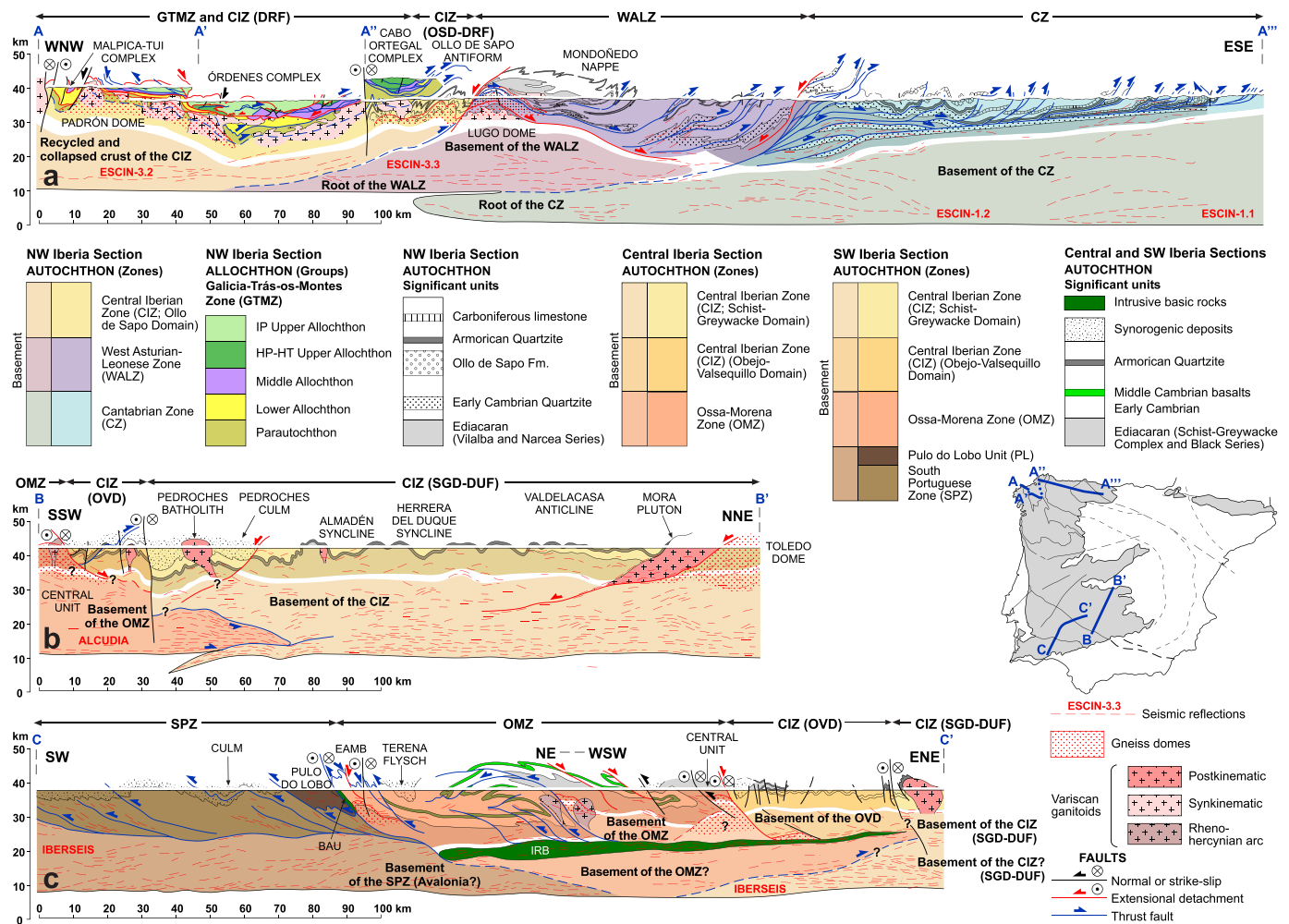
Fig. 3. Cross sections representative of the structure of the Iberian Massif including the Variscan sutures. (a) Northwest Iberian section A-A', modified from Martínez Catalán et al. (2014). (b) Central Iberian section B-B', based on Martínez Poyatos et al. (2012). (c) Southwest Iberian section C-C', based on Simancas et al. (2003) and partly on Rubio Pascual et al. (2013b). The sections are built from field geology and partly using deep seismic reflection profiles. For section A-A', these are ESCIN-1 (Pérez-Estaún et al., 1994, 1995), ESCIN-3.2 (Álvarez-Marrón, 1995, 1996) and ESCIN-3.3 (Martínez Catalán et al., 1995; Ayrza et al., 1998). The two latter were acquired offshore, while section A-A' derives from onshore geology. In the parts of section A-A' roughly corresponding to these two profiles, (GTMZ, CIZ and WALZ), the seismic reflections have been placed approximately. Section B-B' roughly follows the seismic line ALCUDIA (Martínez Poyatos et al., 2012). Section C-C' follows the seismic line IBERSEIS (Simancas et al., 2003). Whrench faults are continued at depth avoiding to cross low-dipping reflections. Colors corresponding to zones or groups are superposed to frames or grey shades indicating lithologies or units. Zones (Z): CZ, Cantabrian; CIZ, Central Iberian; GTMZ, Galicia-Trás-os-Montes; OMZ, Ossa-Morena; SPZ, South Portuguese; WALZ, West Asturian-Leonese. Domains of the CIZ (D): DRF, of Recumbent Folds; DUF, of Upright Folds; OSD, Olla de Sapo; OVD, Obejo-Valsequillo; SGD, Schist-Greywacke. Other units: BAU, Beja-Acebaches; EAMB, Évora-Aracena Metamorphic Belt; IRB, Iberian Reflective Body. Other: Upper Allochthon: IP, Intermediate-P; HP-HT, High-P/High-T. See Fig. 2 for location of the sections.
