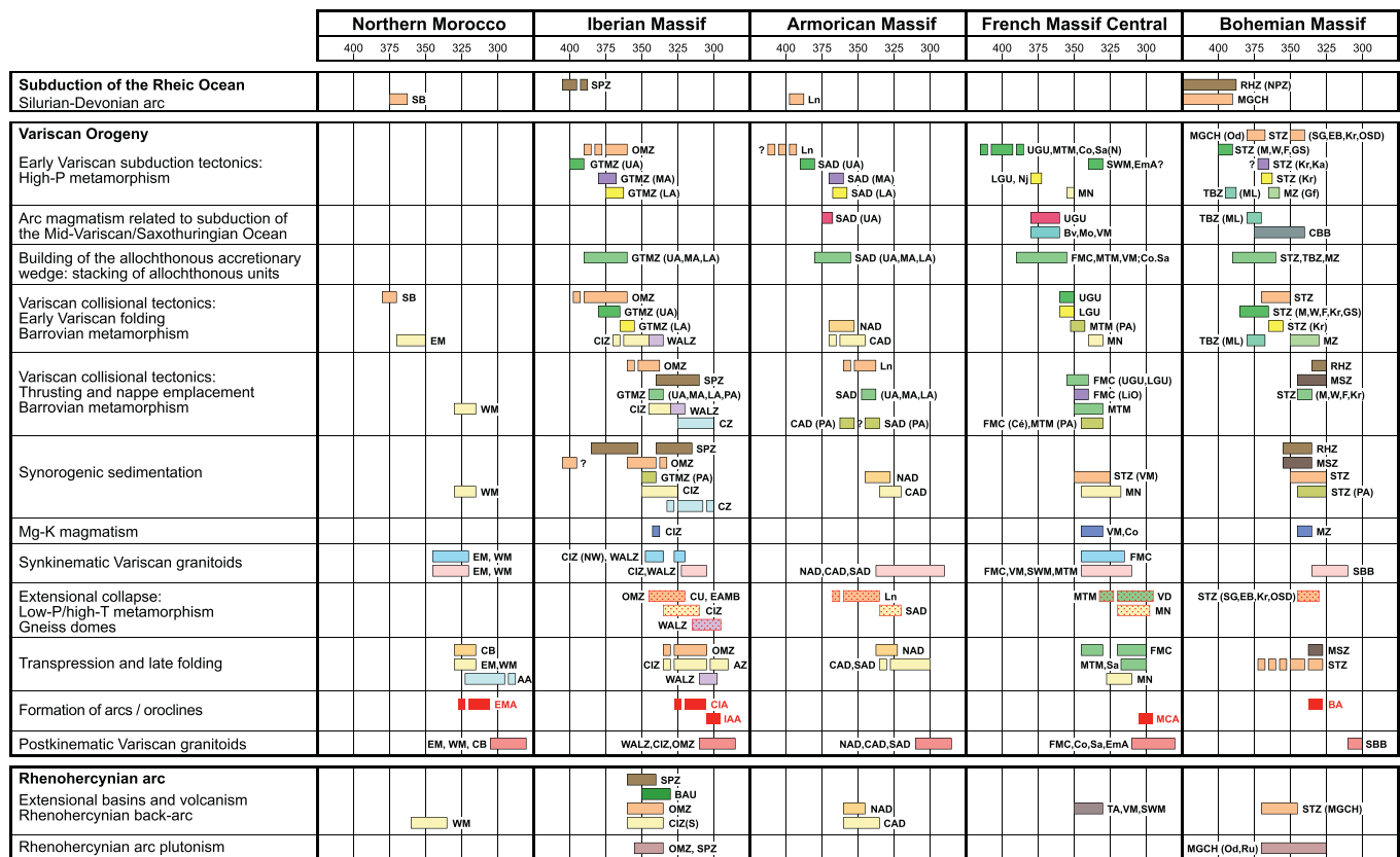
Fig. 10. Timing of early Variscan and Variscan events of the large massifs. The time interval spans 425–275 Ma. Small massifs are assumed to have similar evolutions as the massifs to which they are related in the text, and many of them are included in the figure. Bar colors and abbreviations are the same used in the maps, sections and text. The events related to subduction of the Rheic and Rhenohercynian oceans are given separated from those considered related with the building of the Mid-Variscan accretionary complex forming the Allochthon, their emplacement on the northern Gondwana Autochthon and the subsequent evolution of the ensemble.
