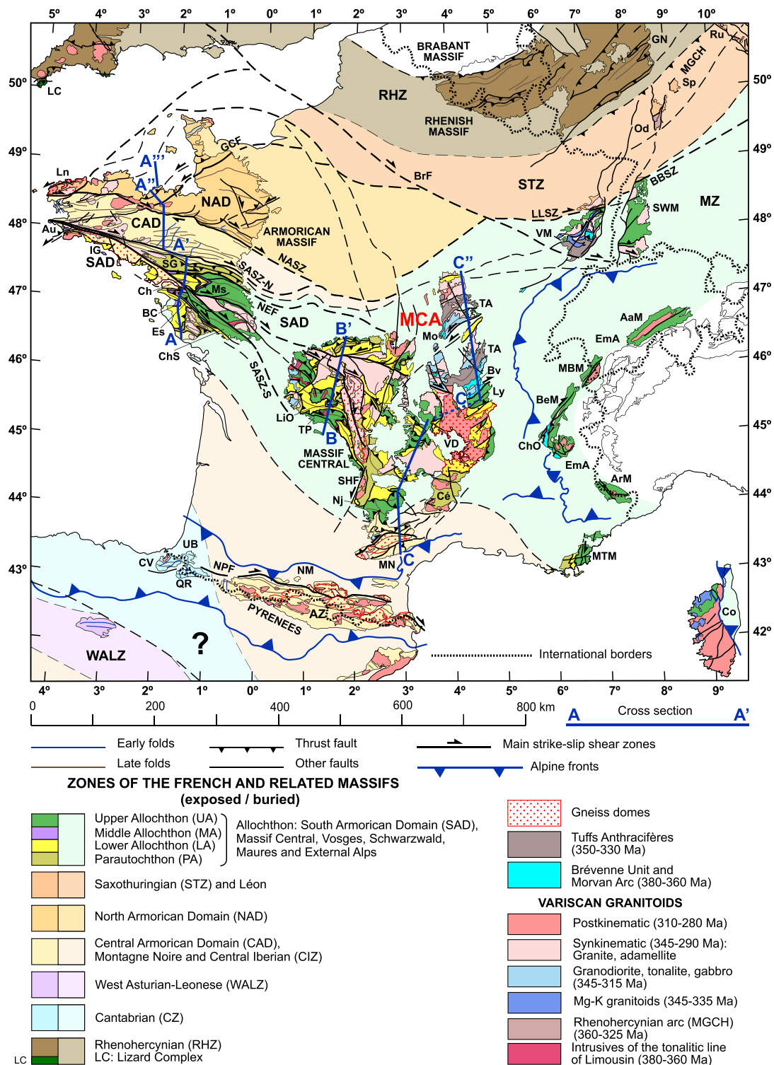
Fig. 4. Geological map of the French and related Variscan Massifs. Based on the Geological map of France to scale 1:1000000 (BRGM, 1996), and in Faure et al. (2009), Ballèvre et al. (2014), and Lardeaux et al. (2014). Zones (Z): MZ, Moldanubian; RHZ, Rhenohercynian; STZ, Saxothuringian; WALZ, West Asturian-Leonese; Armorian Domains (AD): CAD, Central; NAD, North; SAD, South. Shear zones (SZ) and faults (F): BBSZ, Baden-Baden; BrF, Bray; GCF, Granville-Cancalle; LLSZ, Lalaye-Lubine; NASZ, North Armorian; NEF, Nort-sur-Erdre; NPF, North Pyrenean; SASZ, South Armorian (N and S, northern and southern branches); SHF, Sillon Houiller. Arcs (A): MCA, Massif Central. Pyrenees: AZ, Axial zone; NM, Northern massifs; Basque Massifs: CV, Cinco Villas; QR, Quinto Real; UB, Ursuya-Baygura. Other: Au, Audierne Bay Complex; BC, Bois-de-Cené Unit; Bv, Brévenne Unit; Cé, Cévennes; Ch, Champtoceaux Complex; ChO, Chamrousse Ophiolite; ChS, Chantonay Syncline; Co, Corsica; EmA, External Massifs of the Alps (AaM, Aar; ArM, Argentera; BeM, Belledonne; MBM, Mont Blanc); Es, Essarts Unit; GN, Giessen Nappe; IG, Ile-de-Groix; LC, Lizard Complex; LiO, Limousin ophiolite; Ln, Léon; Ly, Lyonnais; MTM, Maures-Tanneron Massif; MGCH, Mid-German Crystalline High; MN, Montagne Noire; Mo, Morvan Arc; Ms, Mauges Unit; Nj, Najac Massif; Od, Odenwald Massif; Ru, Ruhla Massif; SG, St. Georges-sur-Loire Unit; Sp, Spessart Massif; SWM, Schwarzwald Massif; TA, Tuffs Anthracifères; TP, Thiviers-Payzac Unit; VD, Velay Dome; VM, Vosges Massif.
