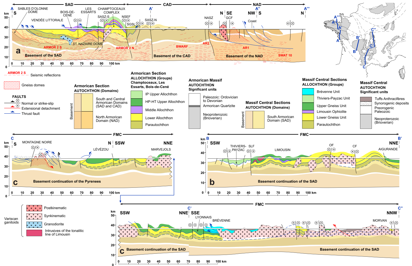
Fig. 5. Cross sections representative of the structure of the French Variscan massifs. (a) Armoric section A-A', including the Mid-Variscan suture in the southern part. (b) Western Massif Central section B-B'. (c) Eastern Massif Central section C-C'. The sections are built from field geology, based on the Geological map of France to scale 1:1000000 (BRGM, 1996), and on geological sections by Ledru et al. (1994b), Faure et al. (2009), Ballèvre et al. (2014), and Lardeaux et al. (2014). Section A-A' follows the trace of seismic reflection profiles ARMOR 2 South and 2 North (Bitri et al., 2003, 2010), AR2, AR1 and SWAT 10 (Bitri et al., 2001), whose interpretations have been included. For the Central Armoric Domain, reflections from the Brittany Wide Angle Refection Profile (BWARF; Matte and Hirn, 1988) separated c. 100 km to the east, have been projected into the section. Whence faults are continued at depth avoiding to cross low-dipping reflections. Colors corresponding to zones or groups are superposed to frames or grey shades indicating lithologies or units. Armoric Domains (AD): CAD, Central; NAD, North; SAD, South. Shear zones (SZ) and faults (F): CF, Combrailles; GCF, Granville-Cancale; NASZ, North Armoric; NEF, Nort-sur-Erdre; OF, Ouzilly; SASZ, South Armoric (N and S, northern and southern branches); SLF, South Limousin. Other: FMC, French Massif Central; MN, Montagne Noire. Upper Allochthon: IP, Intermediate-P; HP-HT, High-P/High-T. See Fig. 4 for location of the sections.
