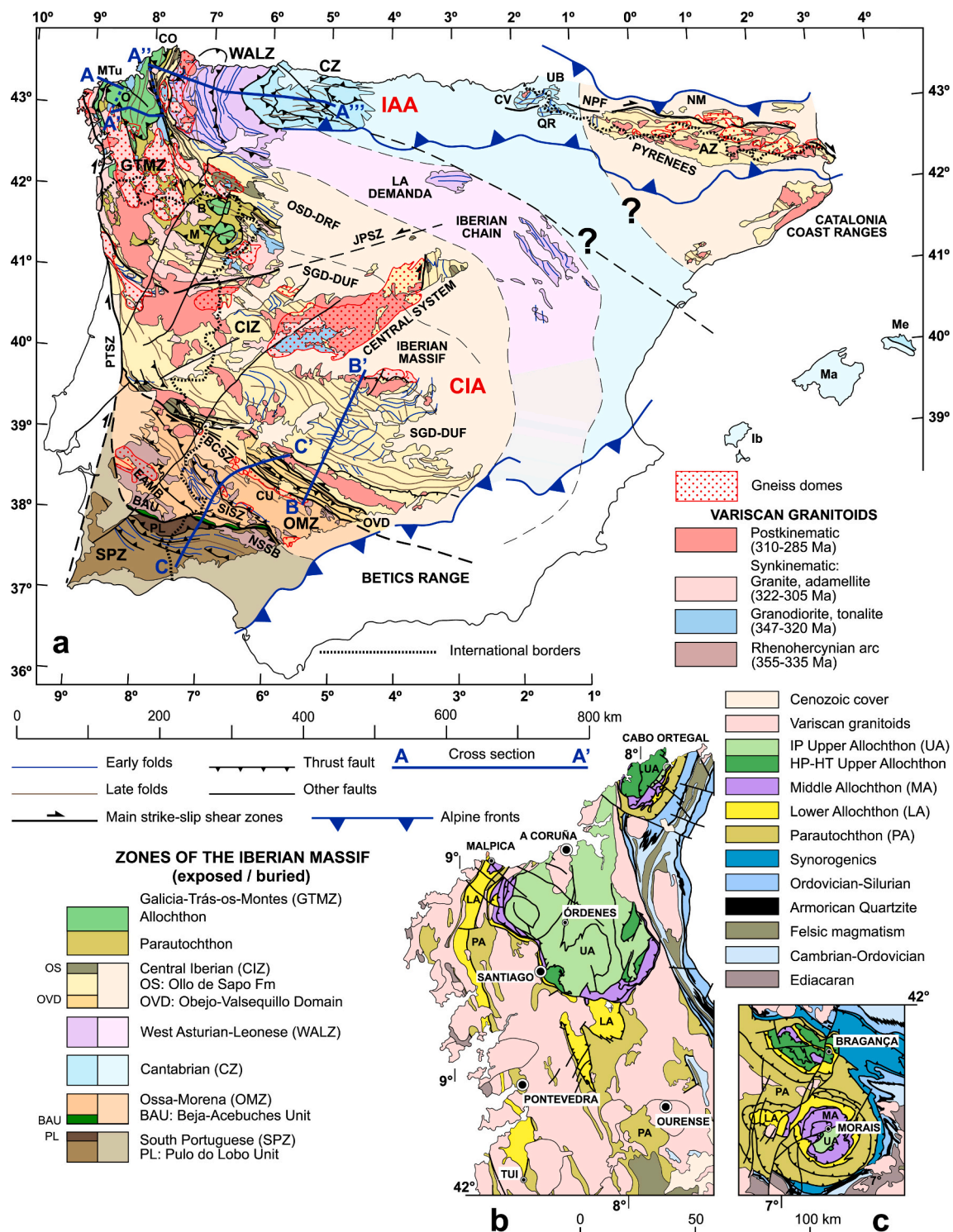
Fig. 2. (a) Geological map of the Iberian Peninsula showing the Variscan massifs and the zones of the Iberian Massif, continued into the Pyrenees, Iberian Chain and Catalonia Coast Ranges. Based on the Geological map of Spain and Portugal to scale 1:1000 000 (IGME-LNEG, 2015) and in Martínez Catalán (2012). The most important structures are shown, including early and late folds, thrust faults, and the main ductile strike-slip shear zones. (b) Detail of the geology of the Galicia allochthonous complexes showing the distribution of the three Allochthons and the Parautochthon. (c) Detail of the geology of the Portuguese allochthonous complexes. Zones (Z): CZ, Cantabrian; CIZ, Central Iberian; GTMZ, Galicia-Trás-os-Montes; OMZ, Ossa-Morena; SPZ, South Portuguese; WALZ, West Asturian-Leonese. Domains of the CIZ (D): DRF, of Recumbent Folds; DUF, of Upright Folds; OSD, Olla de Sapo; OVD, Obejo-Valsequillo Domain. Allochthonous complexes: B, Bragança; CO, Cabo Ortegal; M, Morais; MT, Malpica-Tui; O, Órdenes. Other units: BAU, Beja-Acebuches; CU, Central Unit; EAMB, Évora-Aracena Metamorphic Belt; NSSB, Northern Sierra de Sevilla Batholith; PL, Pulo do Lobo Unit. Shear zones (SZ) and faults (F): BCSZ, Badajoz-Córdoba; JPSZ, Juzbado-Penalva; NPF, North Pyrenean; PTSZ, Porto-Tomar; SISZ, Southern Iberian. Arcs (A): CIA, Central Iberian; IAA, Ibero-Armorican. Pyrenees: AZ, Axial Zone; NM, Northern Massifs; Basque Massifs: CV, Cinco Villas; QR, Quinto Real; UB, Ursuya-Baygura. Balearic Islands: Ma, Majorca; Me, Menorca; Ib, Ibiza. Allochthonous groups: LA, Lower Allochthon; MA, Middle Allochthon; PA, Parautochthon; UA, Upper Allochthon (IP, Intermediate-P; HP-HT, High-P/High-T).
