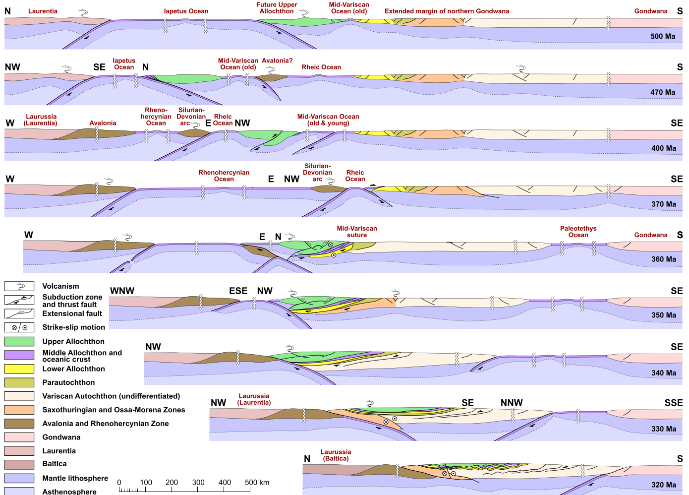
Fig. 13. Proposed plate dynamics of the Variscan Belt depicted using cross-sections, the location of which is indicated by continuous blue lines in Fig. 12. The sections vary for each time frame. They are located to cut across the Mid-Variscan Allochthon except at 370 Ma, designed to highlight the role of the Silurian-Devonian arc. The late Variscan evolution related with transcurrent dextral shearing is not shown. In this figure, the three allochthons and the Parautochthon are depicted with the colors used in previous figures (maps, sections and correlations) to shown their progressive incorporation to the accretionary wedge and its thrusting onto the Autochthon during Variscan collision.
