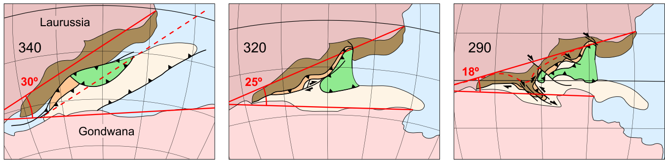
Fig. 14. Late evolution of the Variscan Belt shown in three steps in relation with the relative position of Laurussia and Gondwana using the reconstruction of Matthews et al. (2016). The geographic grid is drawn every 15°, with a thicker line for the Equator. The Variscan Belt became progressively squeezed between the two major plates, as shown by the angle formed by two reference red lines. This angle decreases between 340 and 290 Ma imposing an internal deformation in the triangular area in between, comparable to the trishear kinematic model (Erslev, 1991). The dashed line at 340 Ma approximately represents the position of the parallel continuous line 20 Ma later if only translation had occurred. The curved dashed line at 290 Ma represents a realistic trace of the continuous straight line drawn in Laurussia at 340 Ma. Legend as in Fig. 12.
