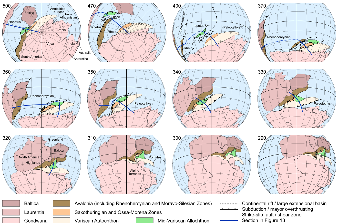
Fig. 12. Evolution of the Variscan Belt in the context of Paleozoic plate dynamics. The main continental masses and the elements forming the Variscan Belt are shown in orthographic projection for different ages. Northern and eastern territories (Siberia, China, Indonesia) are omitted. For the late Cambrian and Lower Ordovician, a projection centered in the South Pole has been used. The geographic grid is drawn every 15^\circ , with a thicker line for the Equator, and is fixed for the 500–470 and 400–290 Ma intervals. This figure was built using animations 500.A97 and 470.A97 of GMap2015, the reconstruction geometries of Domeier and Torsvik (2014) for GPlates, and the partial retrodeformation carried out in this work (Fig. 11). Blue lines indicate the location of sections in Fig. 13 (dotted parts not shown). Note that the Mid-Variscan Allochthon represents the future Upper Allochthon until 400 Ma. Between 390 and 360 Ma it progressively incorporated the Middle and Lower Allochthons and by 340 Ma also the Parautochthon.
