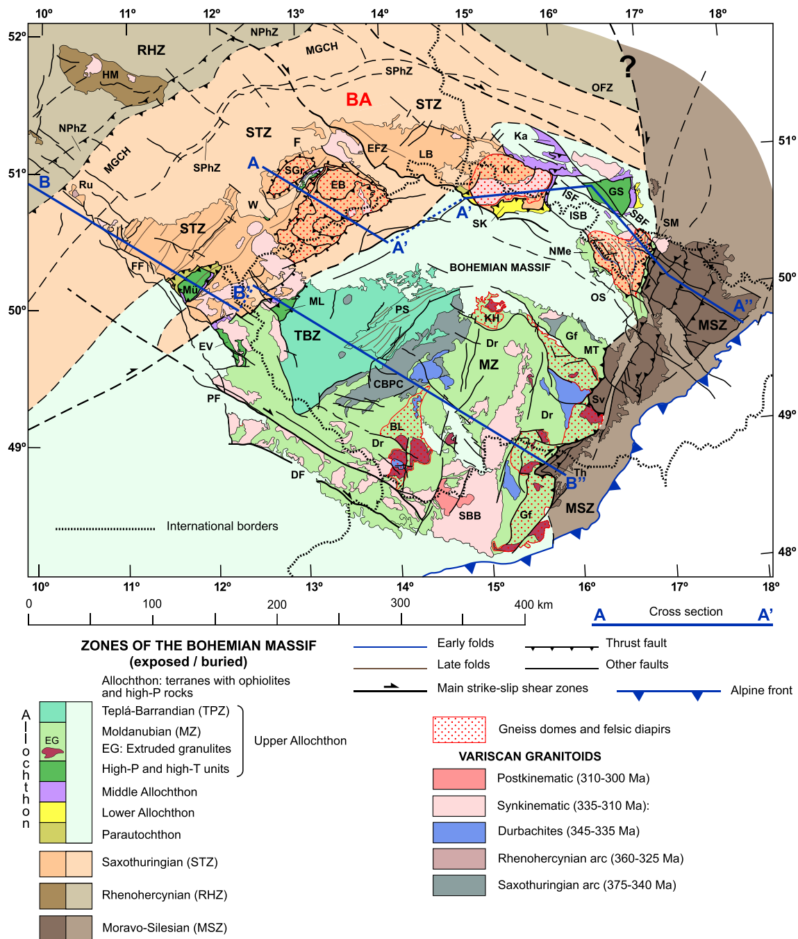
Fig. 6. Geological map of the Bohemian Massif. Based on the Geological maps of Germany to scale 1:1000000 (BGR, 1993), and the Czech Republic to scale 1:500000 (Czech Geological Survey, 2007), and in Mazur and Aleksandrowski (2001), Franke and Żelaźniewicz (2000, 2002), Schulmann et al. (2009, 2014), Zeh and Will (2010), Mazur et al. (2015) and Martínez Catalán et al. (2020). Zones (Z): MZ, Moldanubian; MSZ, Moravo-Silesian; NPhZ, Northern Phyllite; RHZ, Rhenohercynian; SPhZ, Southern Phyllite; STZ, Saxothuringian; TBZ, Teplá-Barrandian. Shear zones (SZ), faults (F) and fault zones (FZ): DF, Danube; EFZ, Elbe; FF, Franconian; ISF, Intra-Sudetic; MT, Moldanubian Thrust; OFZ, Odra; PF, Pfahle; SBF, Sudetic Boundary. Arches (A): BA, Bohemian. Massifs and units: BL, Blanský les; Dr., Drosendorf; EB, Erzgebirge; EV, Erbendorf-Vohenstrauß; F, Frankenberg; Gf, Gföhl; GS, Góry Sowie; HM, Harz Mountains; Ka, Kaczawa Complex; KH, Kutna Hora; Kr, Krkonoše; LB, Lausitz Block; Mü, Münchberg; ML, Mariánské Lázně; NMe, Nové Město; OS, Orlica-Šneznik Dome; PS, Praha Syncline; SG, Saxonian Granulitebirge; SK, South Krkonoše; SM, Staré Město; W, Wildenfels. Other: CBPC, Central Bohemian Plutonic Complex; ISB, Intra-Sudetic Basin; MGCH, Mid-German Crystalline High; Ru, Ruhla; SBB, South Bohemian Batholith; Sv, Svratka window; Th, Thaya window.
