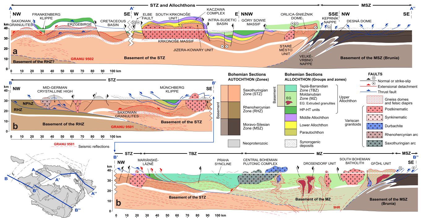
Fig. 7. Representative sections across the Bohemian Massif showing the crustal structure. (a) Northern section A-A', based on Krawczyk et al. (2000), Schulmann and Gayer (2000), Chopin et al. (2012) and Tomek et al. (2019). (b) Southern section B-B'', based on Franke (2000), Schulmann et al. (2005) and Guy et al. (2011). The sections are partly based on deep seismic reflection profiles GRANU 9501 and 9502 (DEKORP and Orogenic Processes Working Groups, 1999; Krawczyk et al., 2000), and 9HR (Chlupáčová and Švancara, 1994). The seismic profiles are more or less close to, but do not coincide with the geological sections, and the reflections have been projected approximately on them. Colors corresponding to zones or groups are superposed to frames or grey shades indicating lithologies or units. Zones (Z): MZ, Moldanubian; MSZ, Moravo-Silesian; NPhZ, Northern Phyllite; RHZ, Rhenohercynian; STZ, Saxothuringian; TBZ, Teplá-Barrandian. See Fig. 6 for location of the sections.
