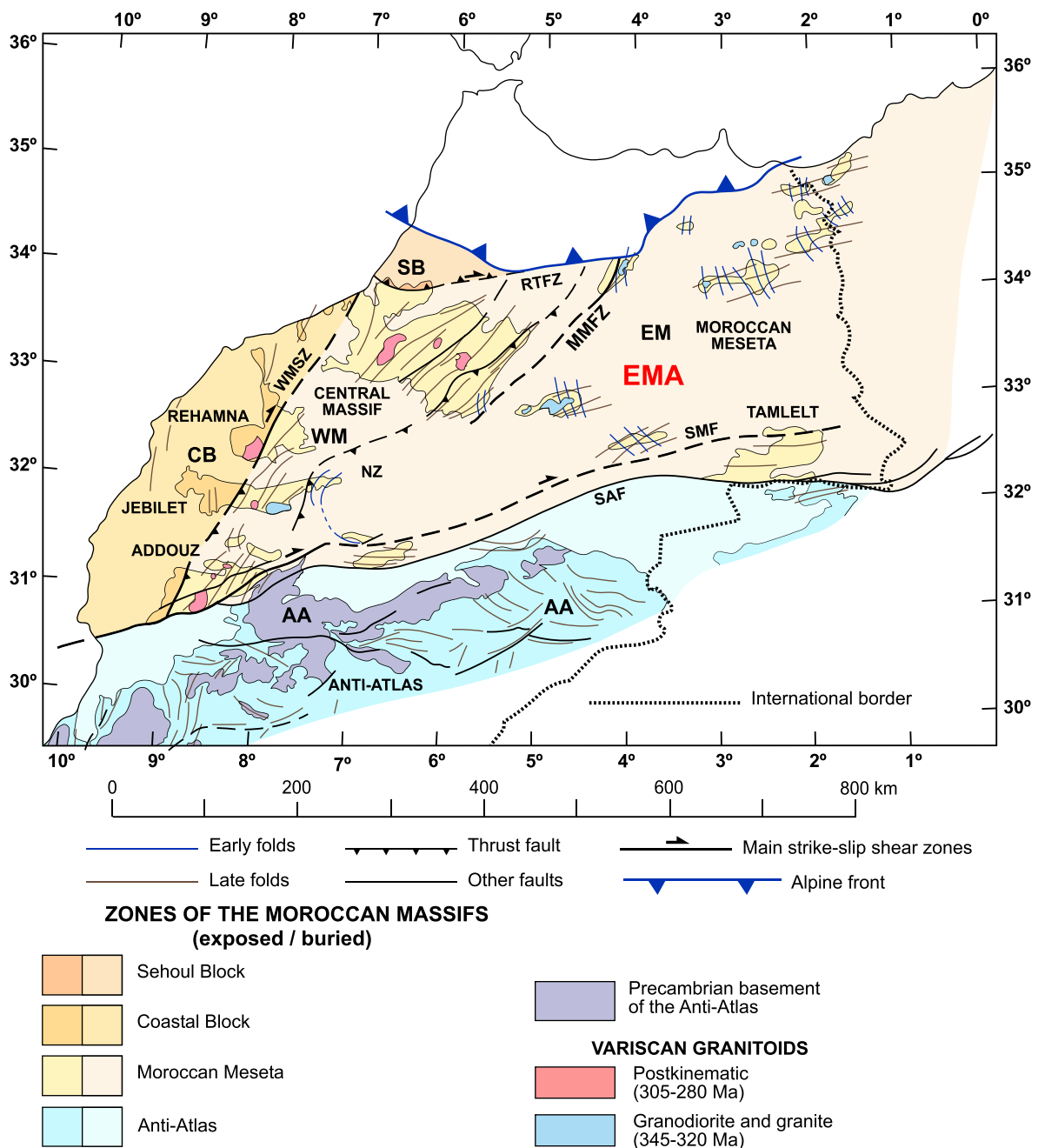
Fig. 8. Geological map of Variscan Morocco. Based on the Geological map of Europe and Adjacent Areas to scale 1:5000000 (BGR, 2005), Michard et al. (2010a) and Ouanaimi et al. (2016). Zones (Z): AA, Anti-Atlas; CB, Coastal Block; EM, Eastern Meseta; SB, Sehoul Block; WM, Western Meseta. Shear zones (SZ), faults (F) and fault zones (FZ): MMFZ, Middle Meseta; RTFZ, Rabat-Tiflet; SAF, South Atlas; SMF, South Meseta; WMSZ, Western Meseta. Arcs (A): EMA, Eastern Meseta. Other: NZ, Nappe Zone; SMFr, South Meseta Front.
