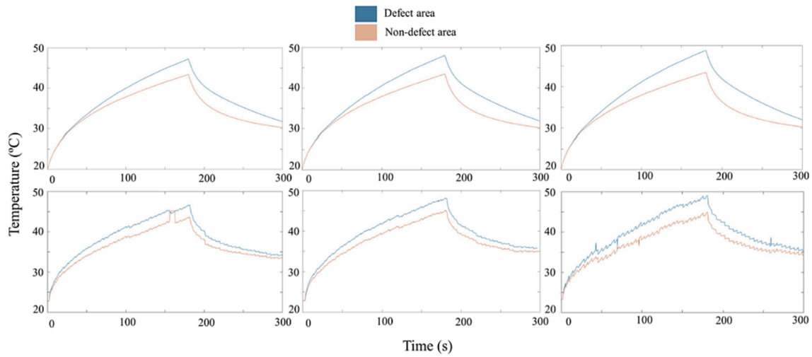
Fig. 7. Differences in the heating and cooling curves between the defect (blue) and non-defect (brown) zone for 10 mm defect length and PLA: results from FEM simulation (up) and from the experimental test (in raw) (down). The X-axis represents the time and the Y-axis the temperature for all plots. (For interpretation of the references to colour in this figure legend, the reader is referred to the web version of this article.)
