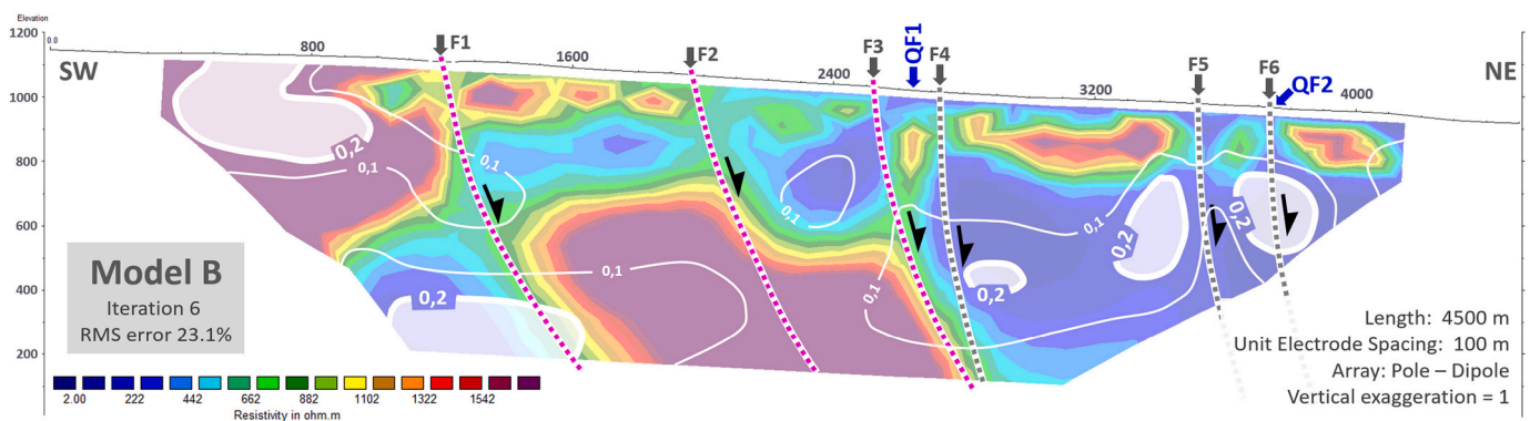
Fig. 10. Depth of Investigation Index (DOI) of the resistivity model. Cells with DOI index greater than 0.2 are considered less reliable. This figure shows how the obtained DOI index do not affect the structural interpretation of the model (Fig. 8).
