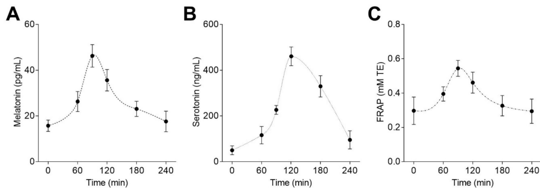
Figure 3. Plasma concentration-time profiles of melatonin (A), serotonin (B), and antioxidant capacity measured by the FRAP method (C) after the administration of lentil sprouts (equivalent to 50 \mu\text{g/kg} melatonin). Each point represents the mean \pm SD ( n = 8 ).
