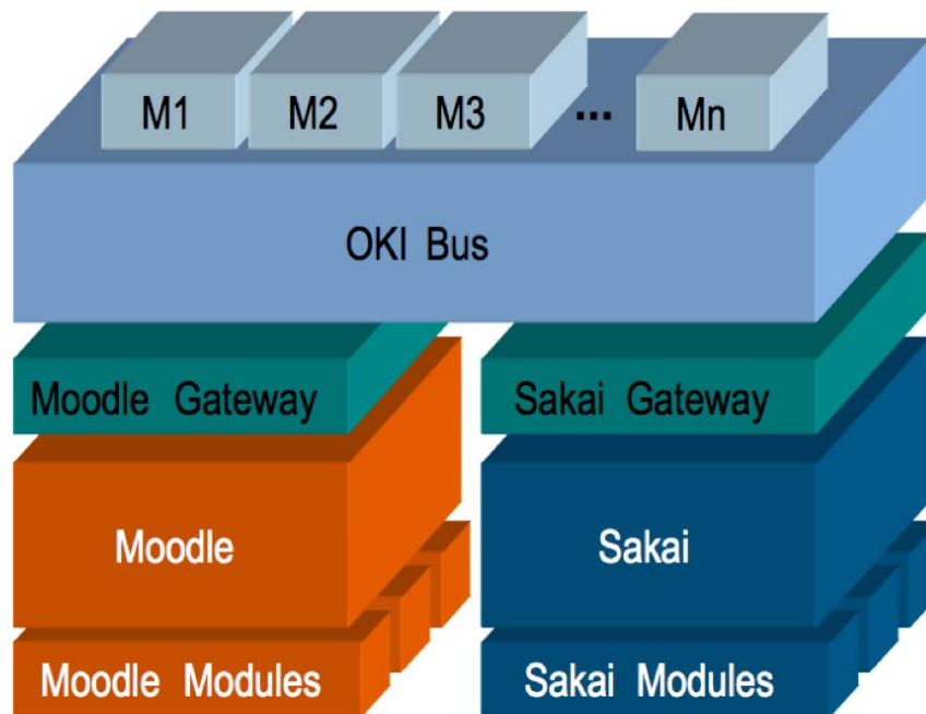
Figure 2: The Campus project architecture [Santanach et al. 07a]
