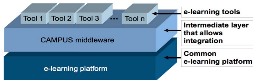
Figure 1: Campus project architecture [Santanach et al. 07a]
