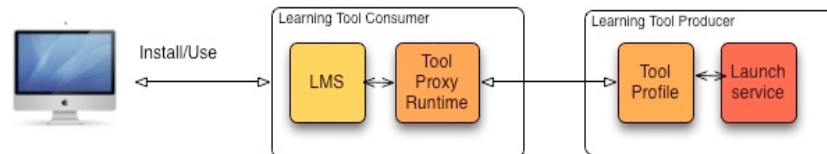
Figure 3: Learning Tool inside the LMS: Installation process
