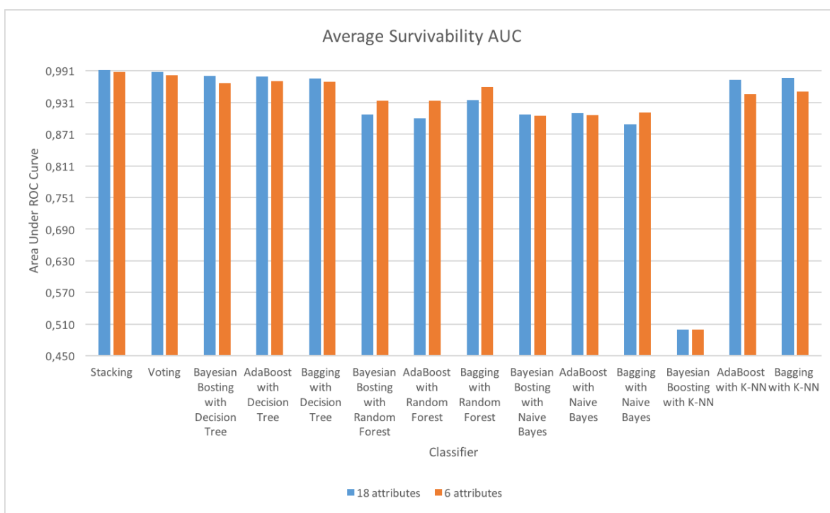
Figure 3: Average survivability AUC: comparison of the 18-attribute models with the 6-attribute models.
