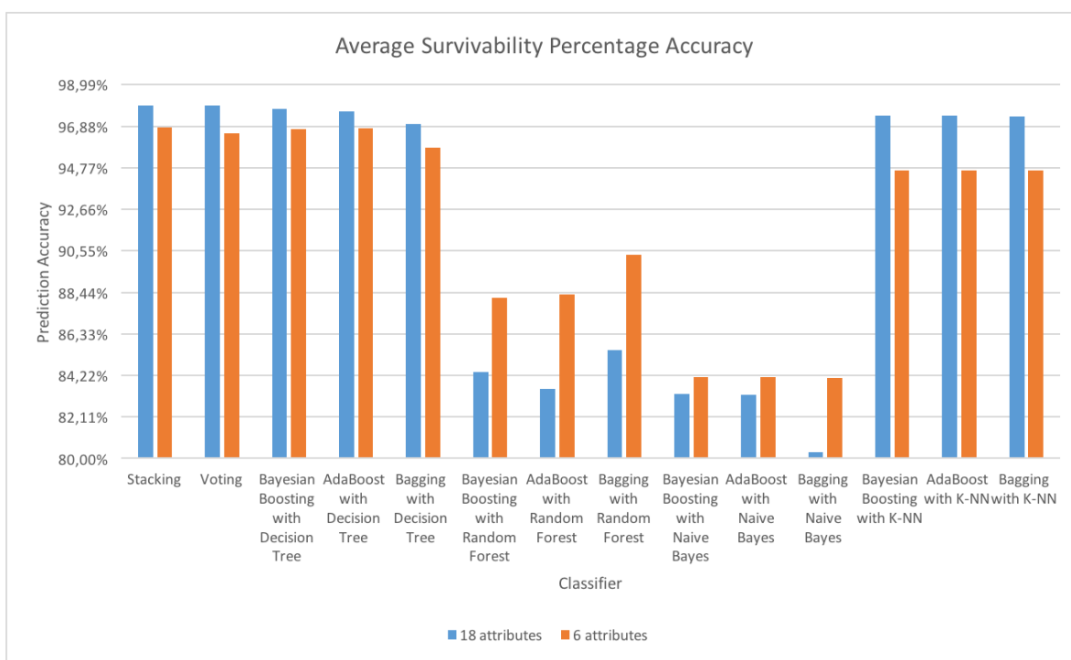
Figure 2: Average survivability percentage accuracy: comparison of the 18-attribute models with the 6-attribute models.
