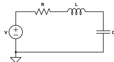
Fig. 2. RLC circuit
