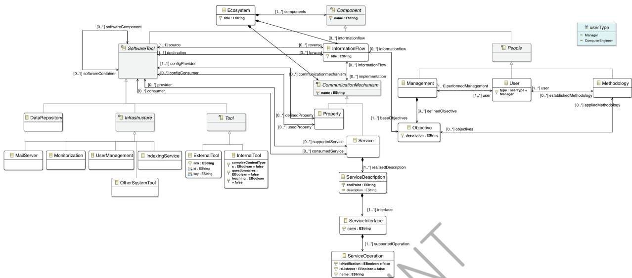
Figure 4. Learning ecosystem metamodel in Ecore
