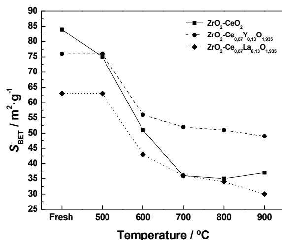
Figure 8. Evolution of S_{BET} with the maximum temperature of the last reduction treatment for the undoped and Ln-doped ZrO 2 -CeO 2 samples during the application of the successive thermochemical ageing treatments.
