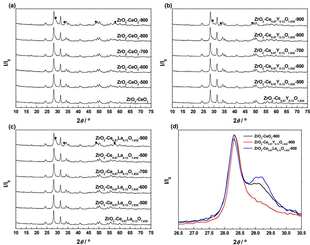
Figure 9. “(a–c) XRD patterns recorded for the undoped and Ln-doped \text{ZrO}_2\text{-CeO}_2 samples, subjected to successive thermochemical ageing treatments at increasing reduction temperatures from 500 to 900 °C. (d) Enlargement of the (111) diffraction peak of monoclinic \text{ZrO}_2 for the undoped and Ln-doped \text{ZrO}_2\text{-CeO}_2 samples subjected to the whole series of reduction treatments up to 900 °C. Caption: ■ \text{Ce}_x\text{Zr}_{1-x}\text{O}_{2-\delta} phases.
