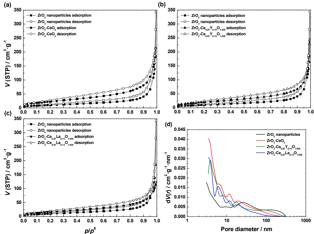
Figure 4. (a–c) Nitrogen adsorption-desorption isotherms at -196^\circ\text{C} and (d) BJH pore size distributions for the commercial ZrO 2 nanoparticles and the fresh undoped and Ln-doped ZrO 2 -CeO 2 samples.
