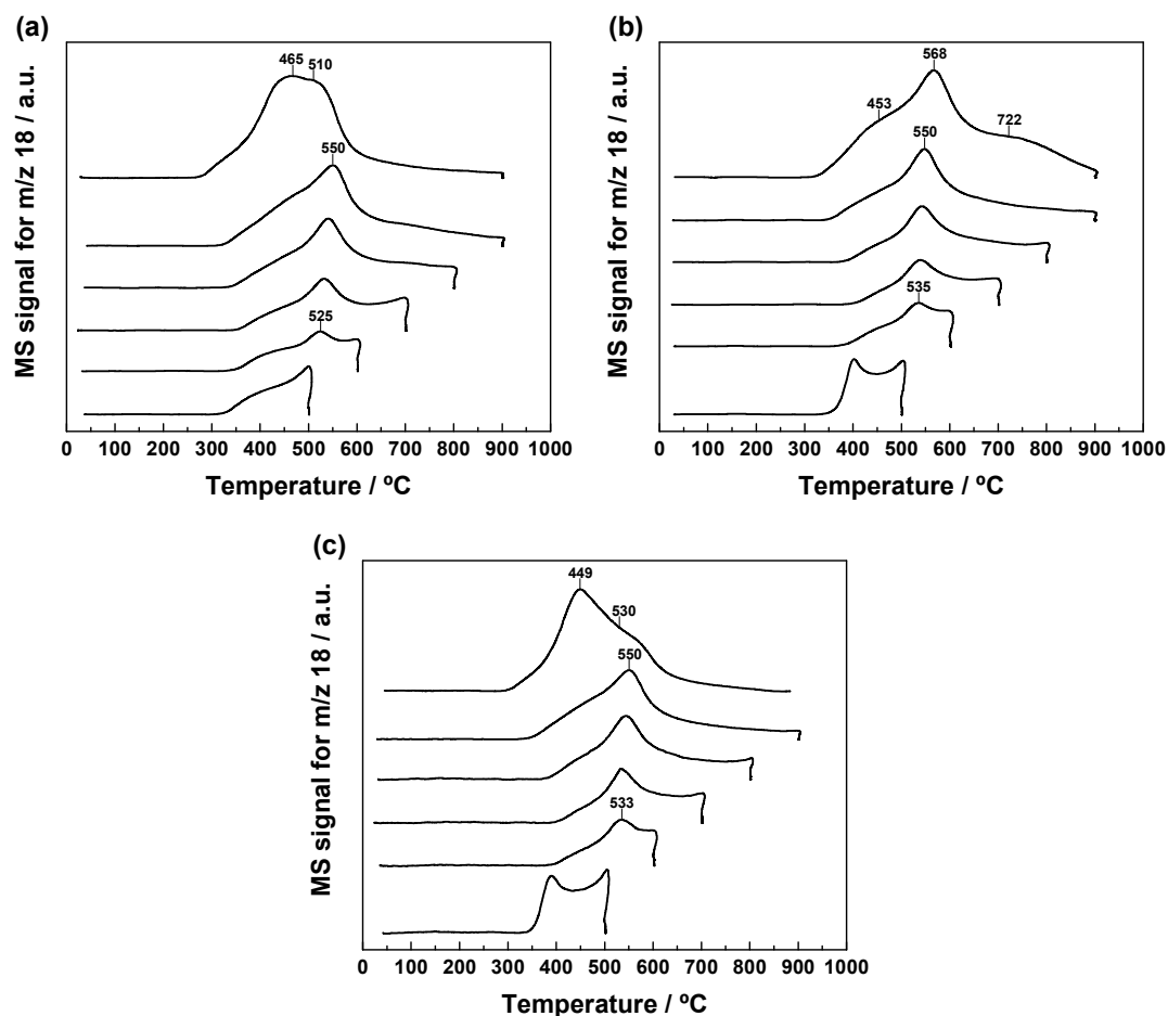
Figure 10. Temperature-programmed reduction (TPR) profiles registered for the undoped and Ln-doped \text{ZrO}_2\text{-CeO}_2 samples during the application of the successive reduction treatments, at increasing temperatures from 500 to 900 °C: (a) \text{ZrO}_2\text{-CeO}_2 , (b) \text{ZrO}_2\text{-Ce}_{0.87}\text{Y}_{0.13}\text{O}_{1.935} , and (c) \text{ZrO}_2\text{-Ce}_{0.87}\text{La}_{0.13}\text{O}_{1.935} .
