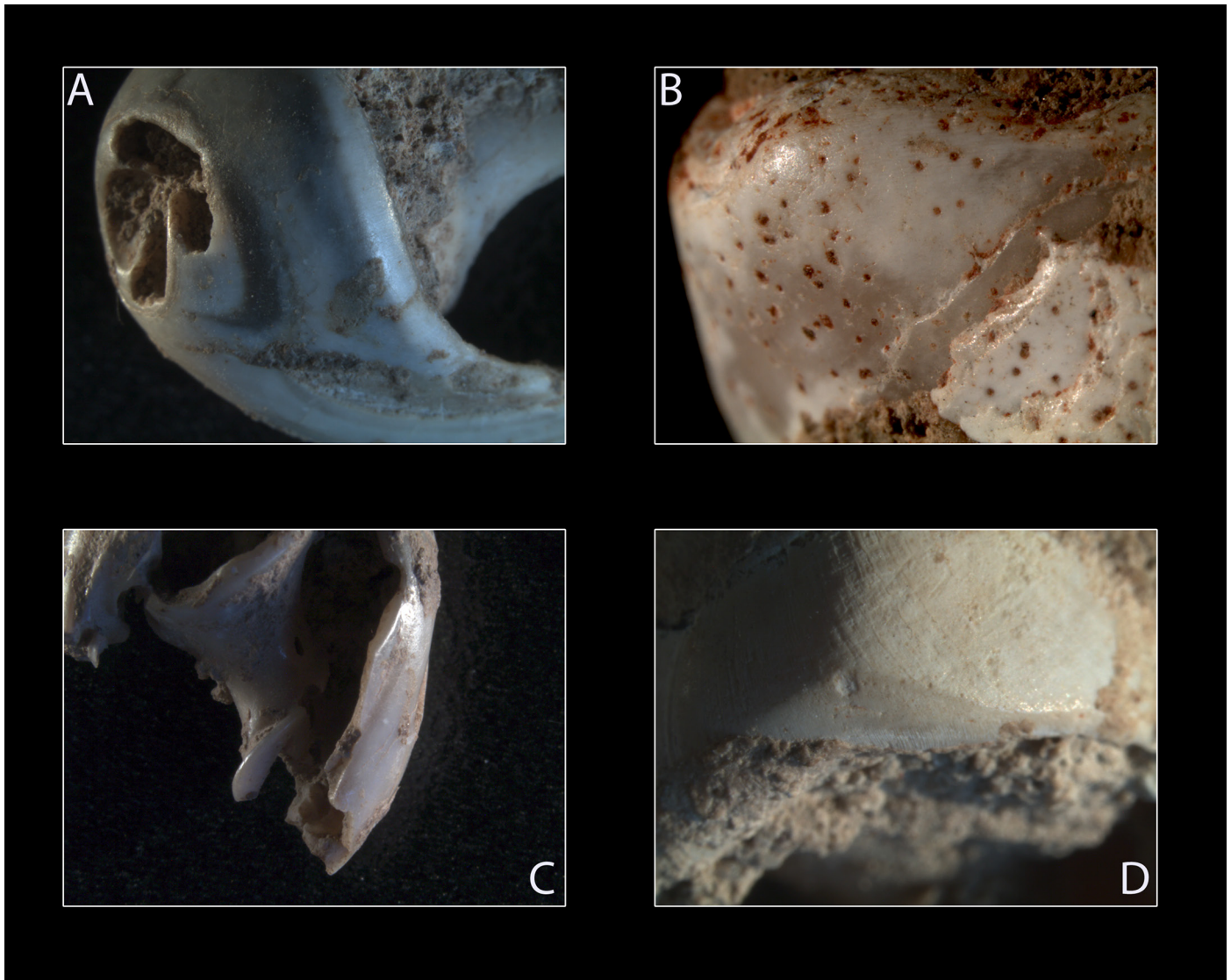
Figure 4. Examples of some of the taphonomic attributes identified on the Contrebandiers Aterian (Layer CEA-4) sample, illustrating A) shining or polish (I15-371; 10x magnification), B) red staining in pits created by bioeroders (I15-367; 12.5x magnification), C) shining or polish and breakage along the worn area of the shell (I14-198; 8x magnification), and D) abrasion (I15-324; 16x magnification). Images are courtesy of the Contrebandiers Project and A, B and D are from Dibble et al. (2012).
