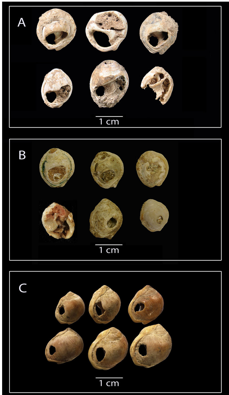
Figure 3. A comparison of a few examples of the shells discussed in the text. The specimens are from A) Contrebandiers Cave, Morocco, B) a fossil beach outcrop in Temara, Morocco (Chahid et al. 2016; Chakroun et al. 2017), and C) Blombos Cave, South Africa. Images A and B are courtesy of the Contrebandiers Project (from Dibble et al. 2012) and C is courtesy of Christopher Henshilwood, Francesco d'Errico, and Marian Vanhaeren (from Henshilwood et al. 2004).
