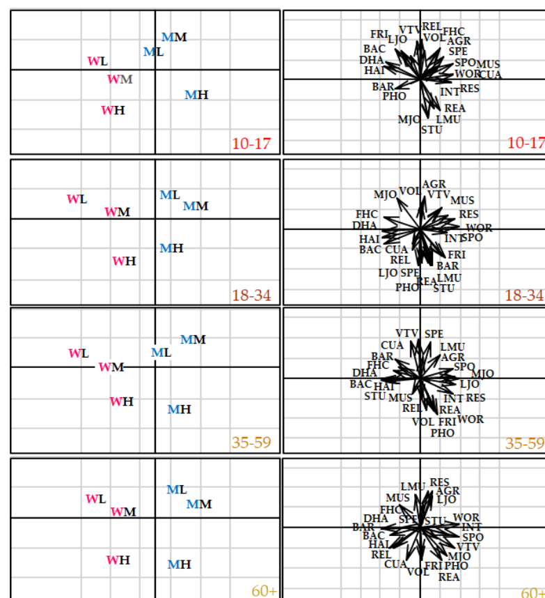
Figure 7. Compromise projections of gender-SES and age group in the year 2017.
