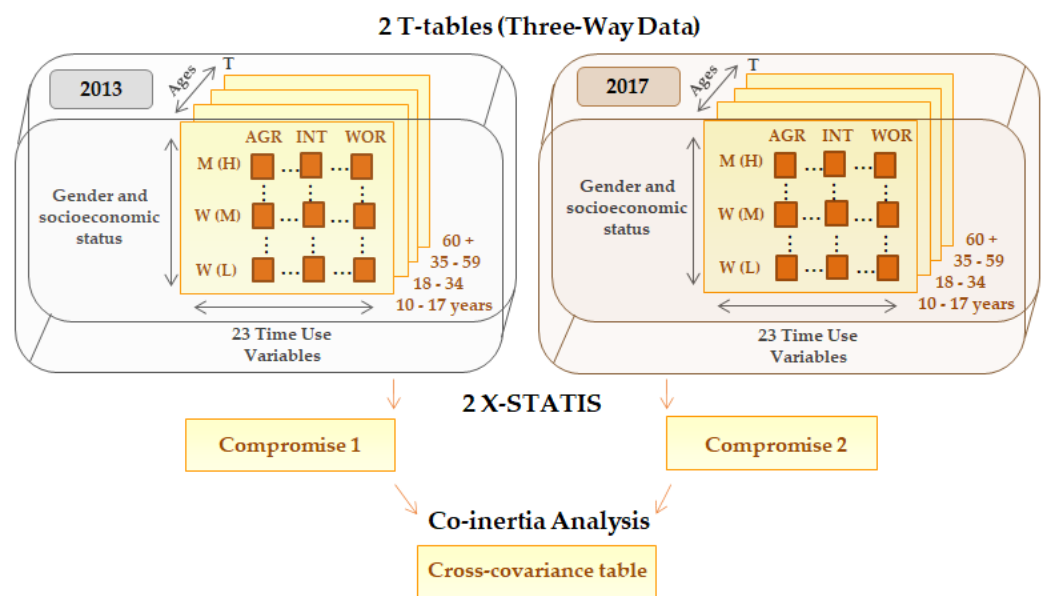
Figure 2. Data analysis scheme for the CO-STATIS technique.
