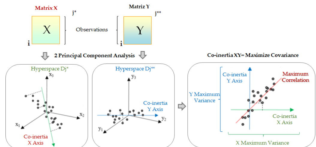
Figure 4. Co-inertia analysis scheme.
