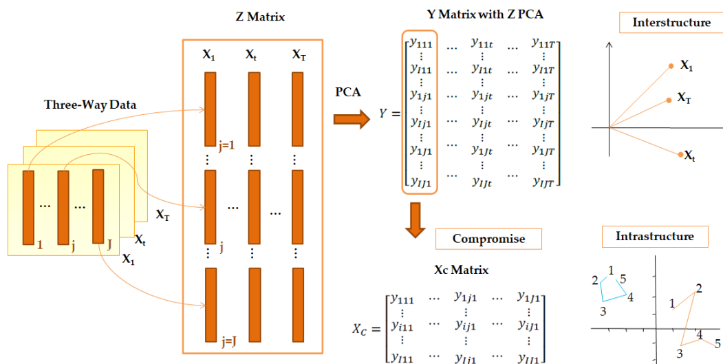
Figure 3. Data analysis scheme for the X-STATIS.
