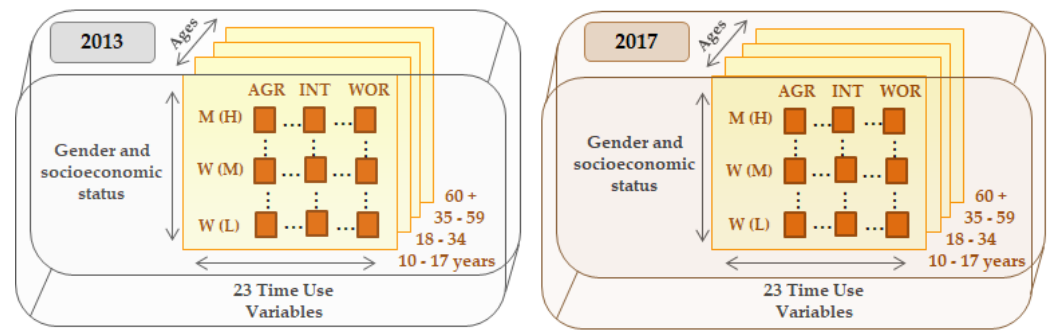
Figure 1. Structure of the data in analysis.
