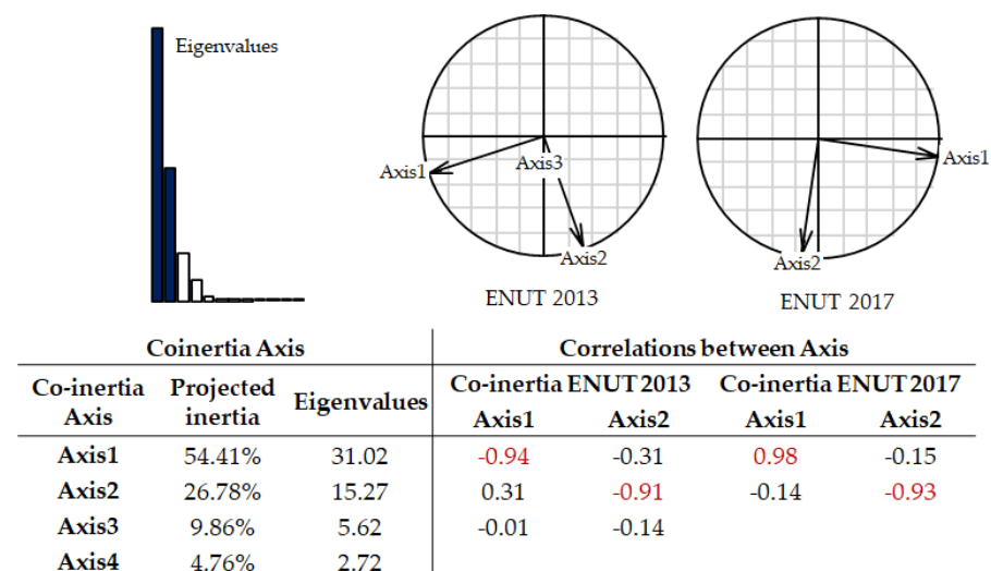
Figure 8. Co-inertia axes and correlations with axes of the principal component analysis.
