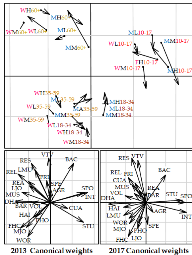
Figure 9. Co-structure graphs of the co-inertia between ENUT 2017 and 2013.
