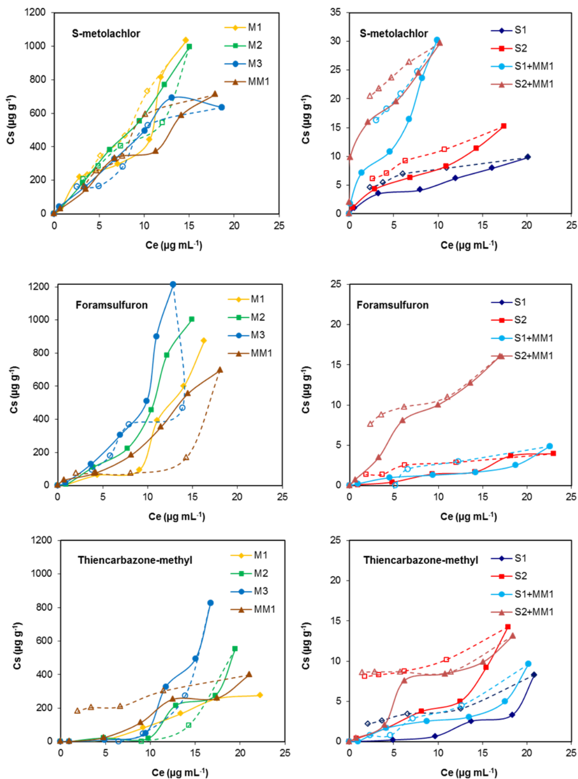
Figure 36. Adsorption-desorption isotherms of S-metolachlor, foramsulfuron, and thien carbazole-methyl for mulches (M1, M2, M3 and MM1), unamended (S1 and S2) and MM1-amended soils (S1 + MM1 and S2 + MM1). Closed symbols and continuous line correspond to adsorption, and open symbols and dashed line correspond to desorption.
