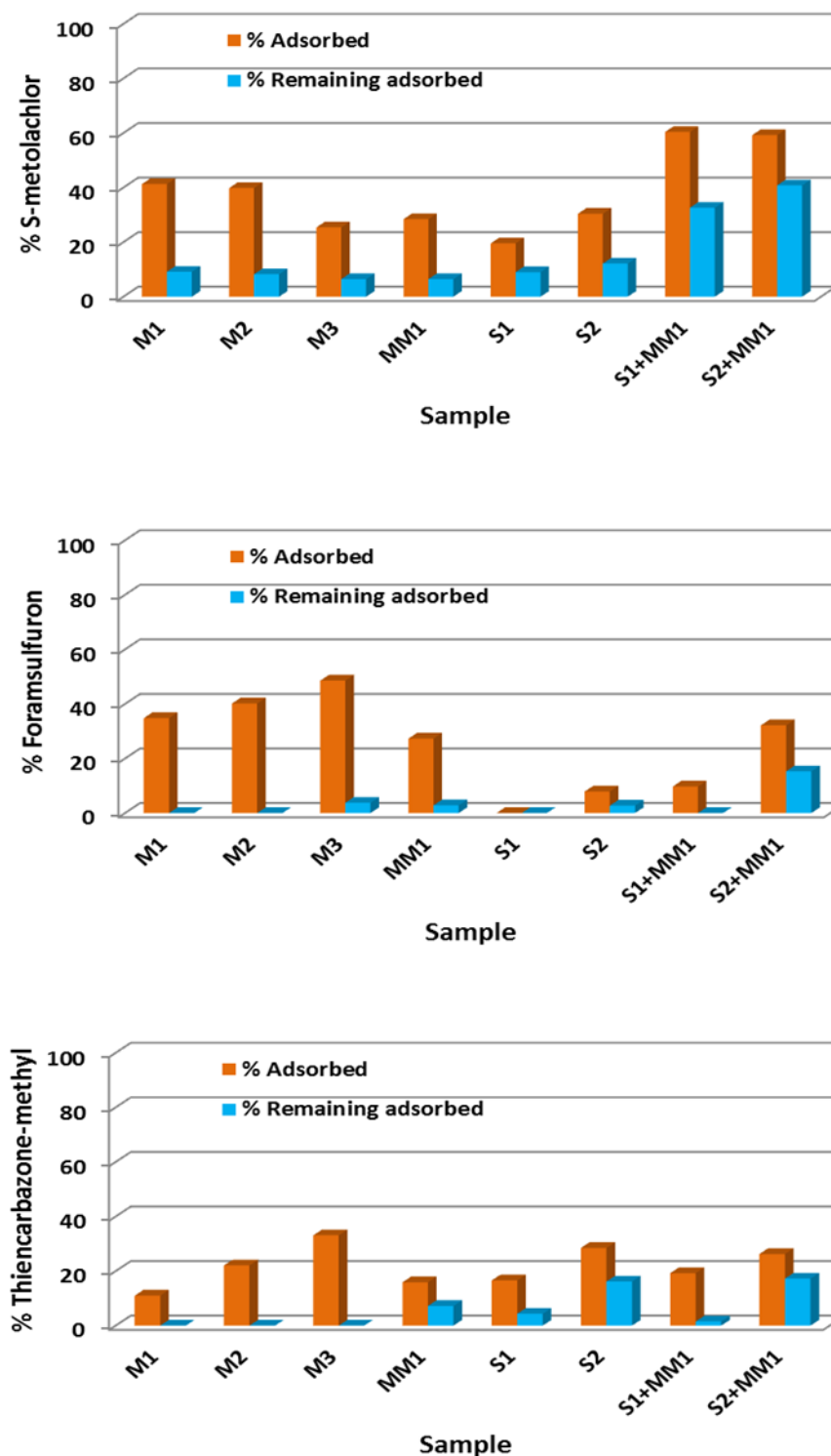
Figure 37. Adsorbed amounts expressed as percentages of herbicide (S-metolachlor, foramsulfuron or thien carbazon-methyl) in aqueous solution at an initial concentration of 25 \mu\text{g mL}^{-1} , and the residual amounts adsorbed after desorption (four steps) expressed as percentages of the herbicide adsorbed by the mulches (M1, M2, M3 and MM1), unamended (S1 and S2) and MM1-amended soils (S1 + MM1 and S2 + MM1).
