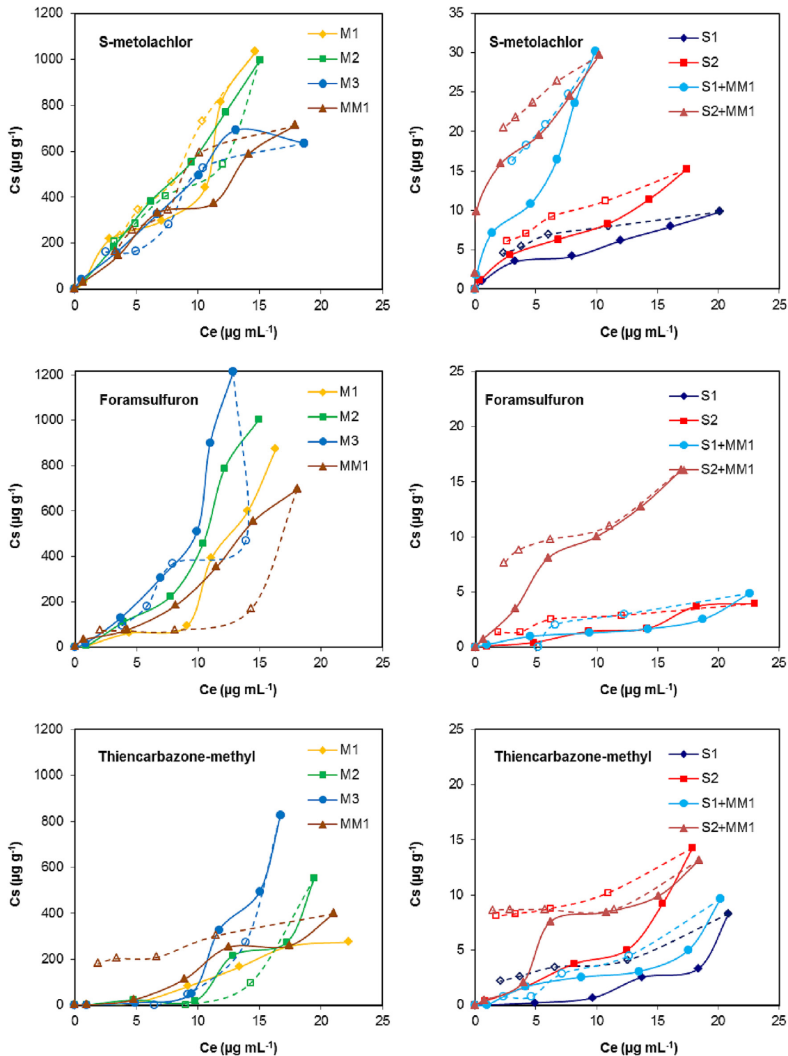
Fig. 1. Adsorption-desorption isotherms of S-metolachlor, foramsulfuron, and thien carbazon-methyl for mulches (M1, M2, M3 and MM1), unamended (S1 and S2) and MM1-amended soils (S1 + MM1 and S2 + MM1). Closed symbols and continuous line correspond to adsorption and open symbols and dashed line correspond to desorption.
