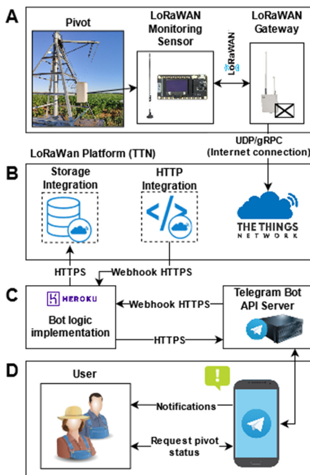
Fig. 2 – Telegram Bot system architecture.
