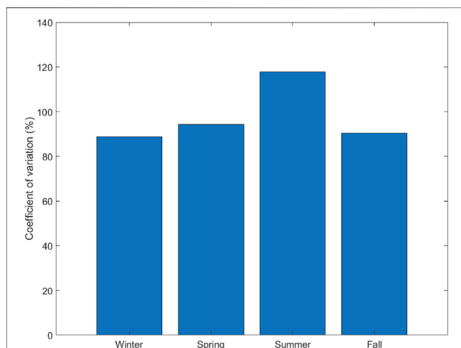
FIGURE 9 | Seasonal distribution of the coefficient of variation of the daily precipitation at the four weather stations located in the REMEDHUS area.
