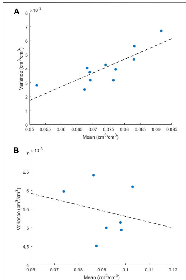
FIGURE 8 | Relationship between the average daily mean soil moisture and variance in the summer months (JJA) when precipitation is lower (A) or above the average (B).
