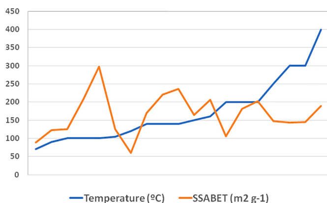
Fig. 3. SSA values and temperatures of outgassing from the data recorded in Table 2, plotted from the lowest to the highest temperature used for out-gassing.
