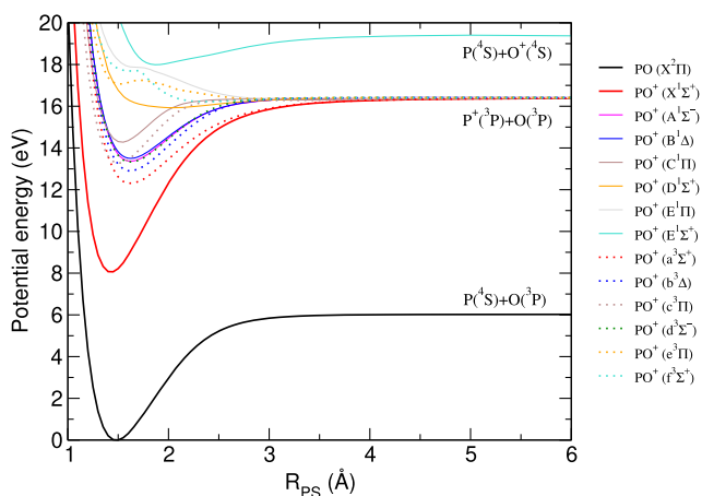
FIGURE 6 | MRCI+Q/V5Z potential energy curves (PECs) of PO ground electronic state and all the singlet and triplet electronic states of PO + correlating to P + ( 3 P) + O( 3 P) and P( 4 S) + O + ( 4 S). For clarity, the triplet states are represented with dashed lines.
