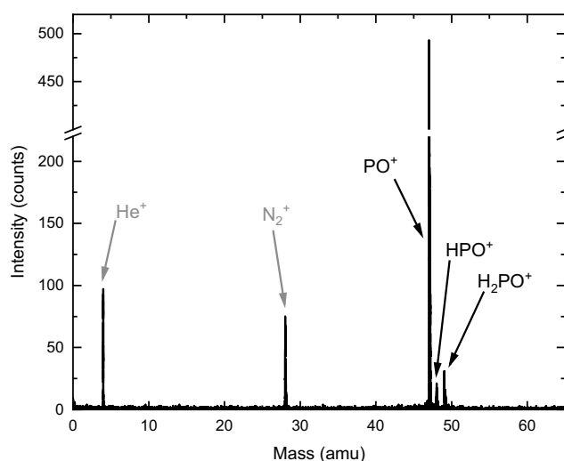
FIGURE 4 | TOFMS obtained from the integration of the photoionization in the 8.0–8.9 eV photon energy range using the \text{PH}_3 + \text{O} mixture. \text{PO}^+ , \text{HPO}^+ and \text{H}_2\text{PO}^+ are visible at m/z=47 , 48 and 49, respectively. The peaks at m/z=4 and 28, correspond to \text{He}^+ and \text{N}_2^+ , respectively, used as carrier gases in the experiments.
