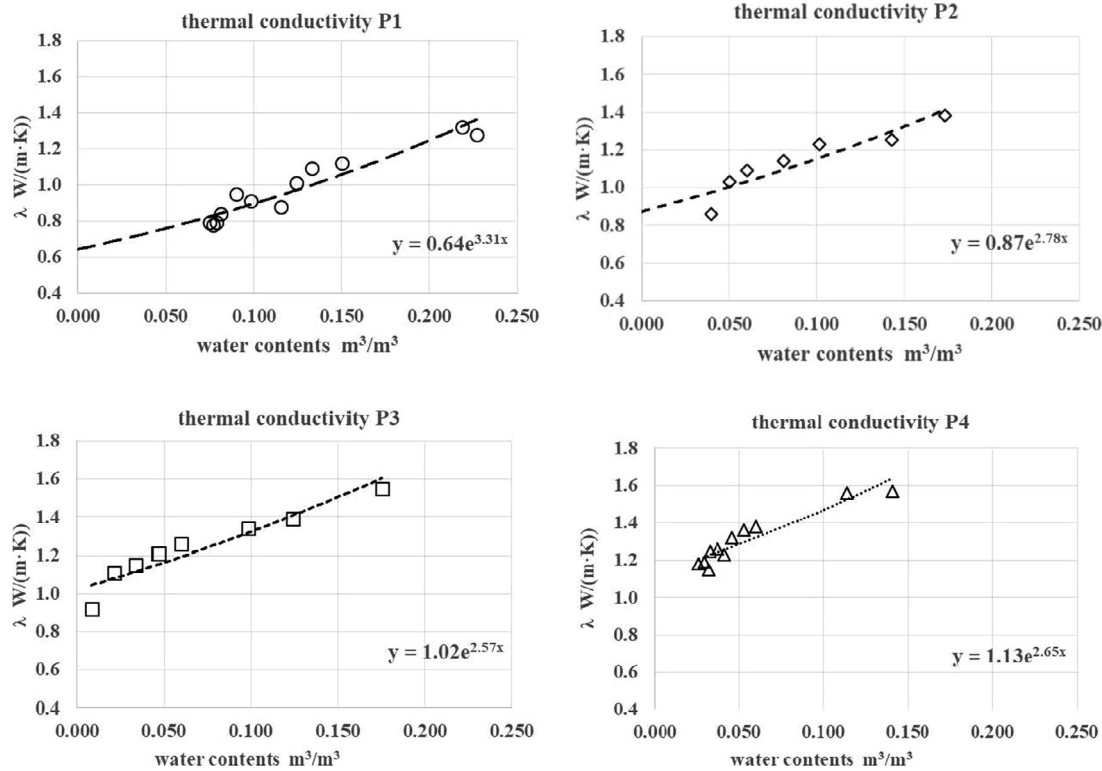
Fig. 7. Graph showing the result of the heat flow test: the thermal conductivity of the specimens in relation to the water content in m³/m³.
