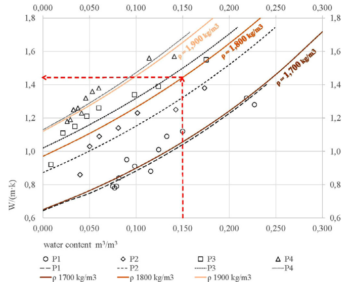
Fig. 8. Abacus with the result of the heat flow test, the thermal conductivity of the specimens in relation to the water content in m³/m³.
