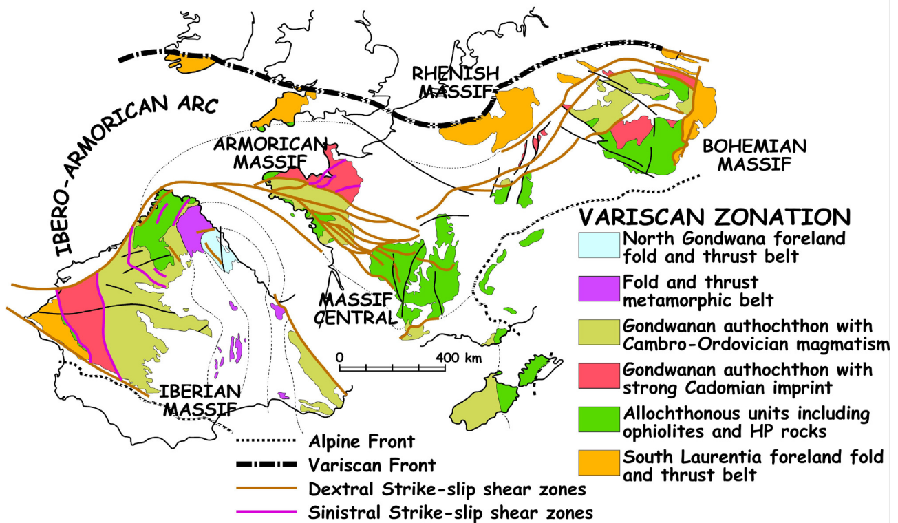
FIGURE 1. The Western European Variscan Belt showing geological zones or domains. The hairpin shaped Iberian Orocline, a major bend affecting the Variscan orogen. After Martínez Catalán et al. , 2007.
