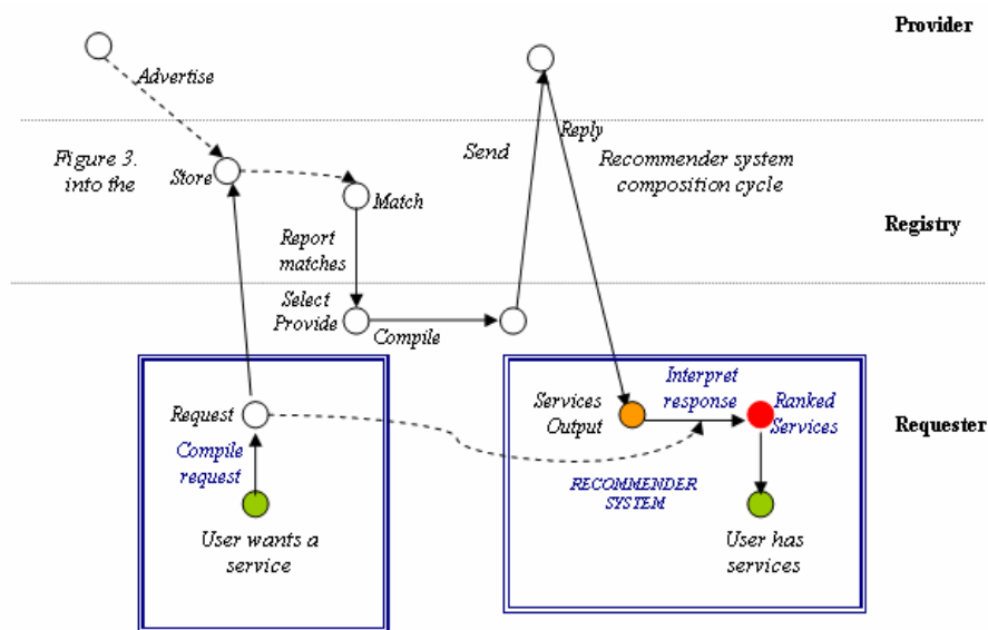
Figure 3: Recommender system in the composition cycle
