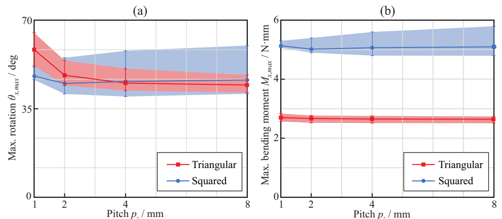
Figure 7. Bending analysis: effect of the pitch on the maximum rotation (a) and maximum applied torque (b) when the end of the martensitic elastic regime is reached.
