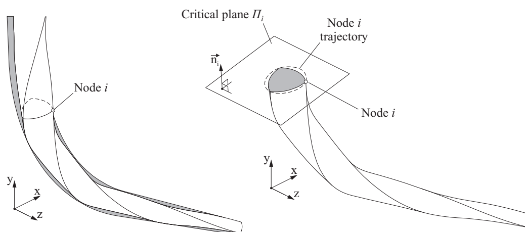
Figure 7. Determination of the critical plane and bending strain for node i .
