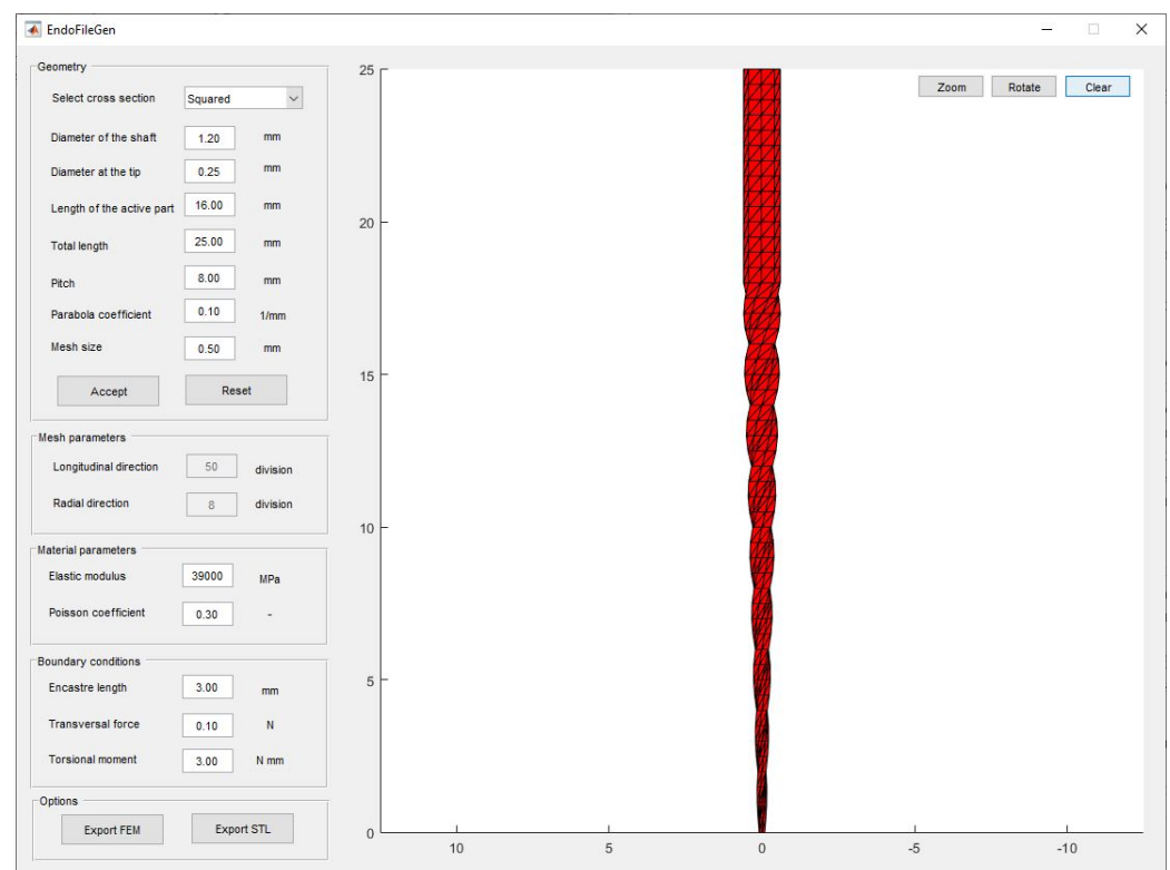
Figure 5. Graphical interface for the developed computer program.
