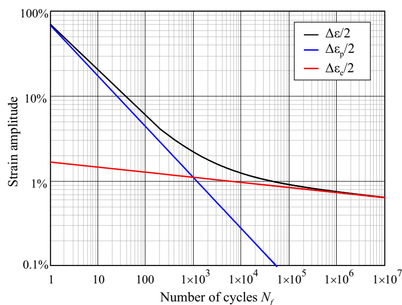
Figure 6. Coffin–Manson relation between strain amplitude and number of cycles to failure (NCF). Parameters for NiTi from [25]: \varepsilon'_F = 0.68 , \sigma'_F = 705 MPa, E = 42.5 GPa, c = -0.6 , b = -0.06 .
