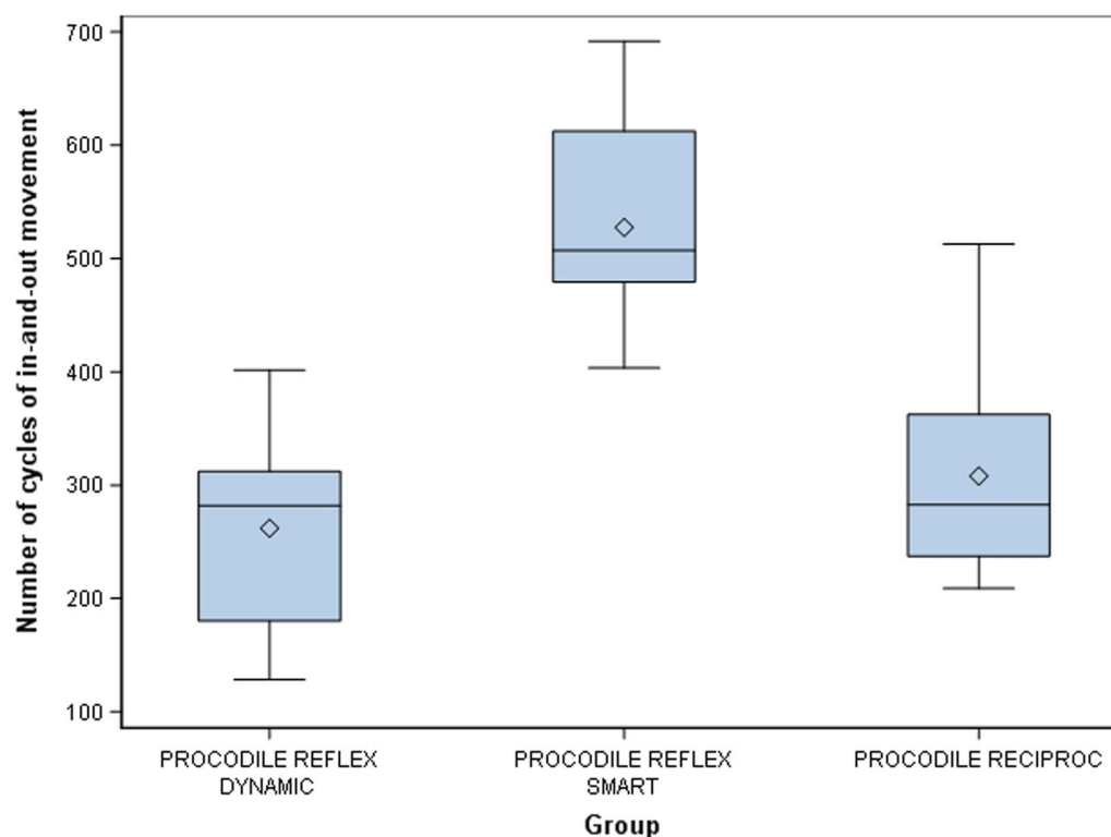
Fig. 4 Box plots of number of cycles of in-and-out movement of experimental groups. Horizontal line in each box represents median value
