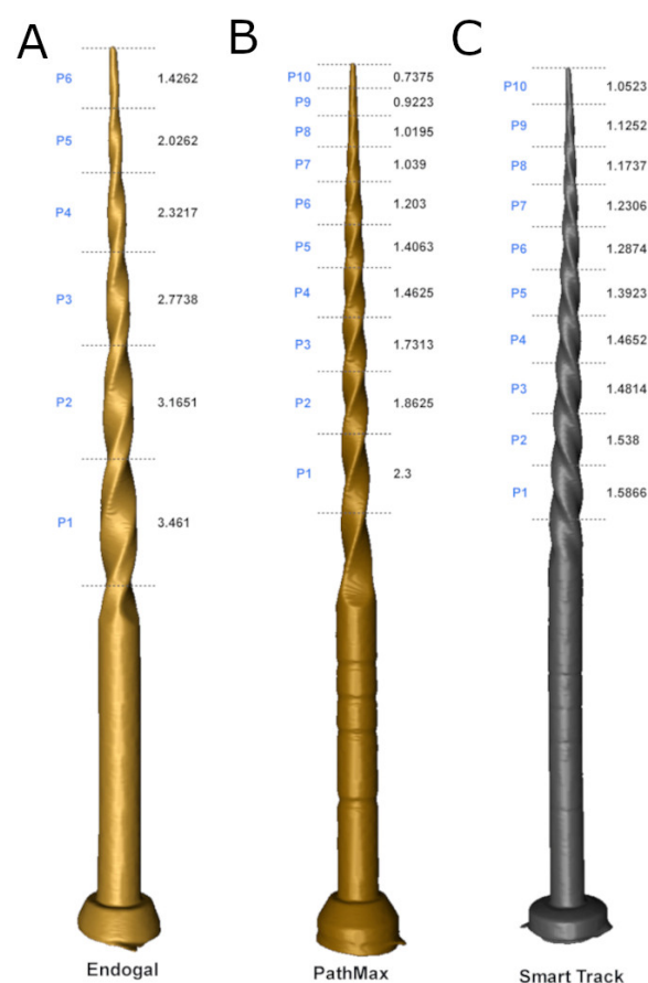
Figure 5. (A) STL digital files of EDG NiTi alloy endodontic rotary file, (B) PMP heat-treated NiTi alloy endodontic rotary file, and (C) ST heat-treated NiTi alloy endodontic reciprocating file.
