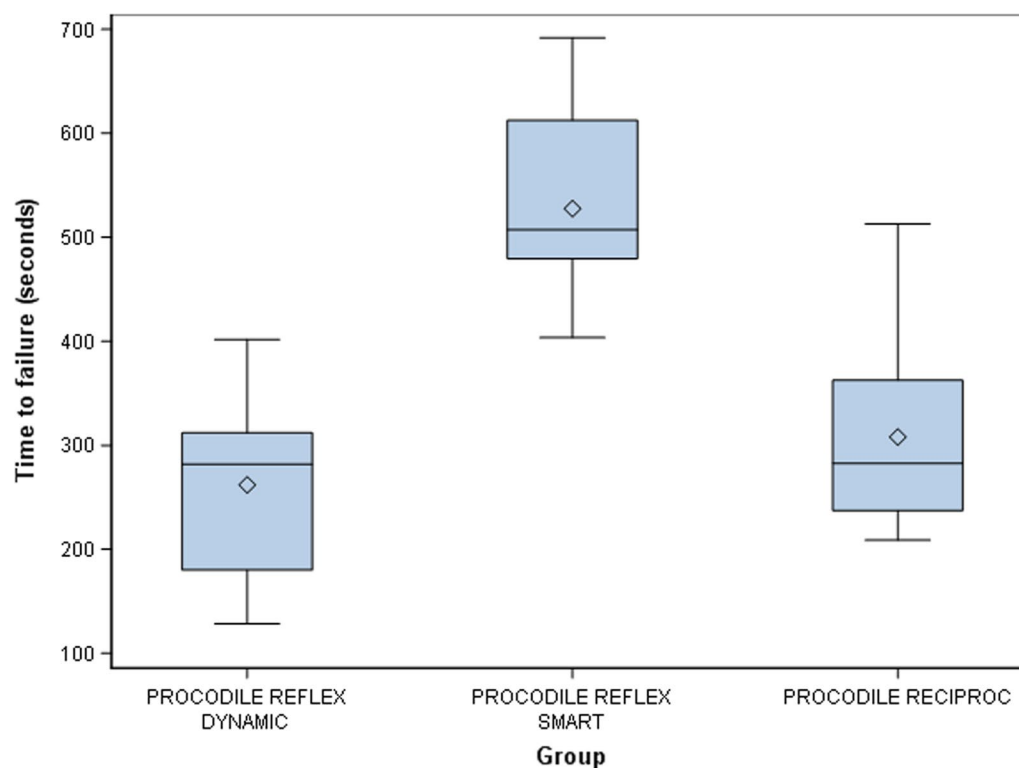
Fig. 2 Box plots of time to failure of experimental groups. Horizontal line in each box represents median value
