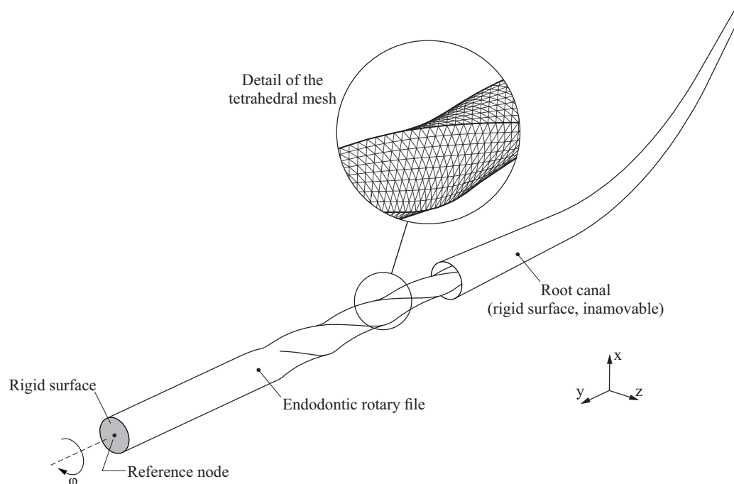
Figure 4. Definition of the finite element model.
