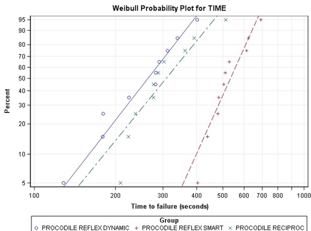
Fig. 3 Weibull probability plot of time to failure
