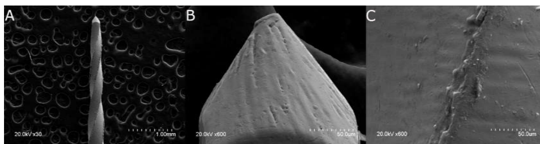
Figure 2. (A) SEM images of the full-length NiTi alloy endodontic rotary files (Ref.: IRE 02506, D, Endogal, Galician Endodontics Company, Lugo, Spain) at \times 30 , (B) and specifically of the end of the file at \times 600 and (C) the surface of the file at \times 600 .
