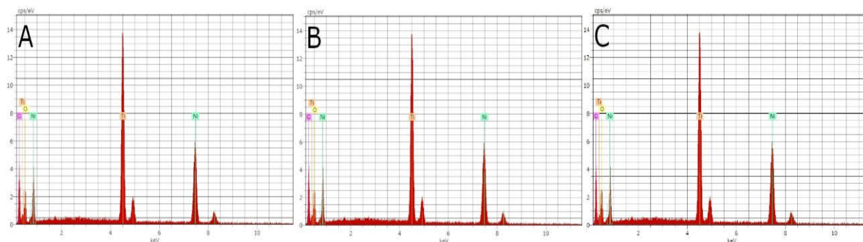
Figure 3. EDX micro-analysis of the NiTi alloy endodontic rotary files at locations (A) 1, (B) 2, and (C) 3.
