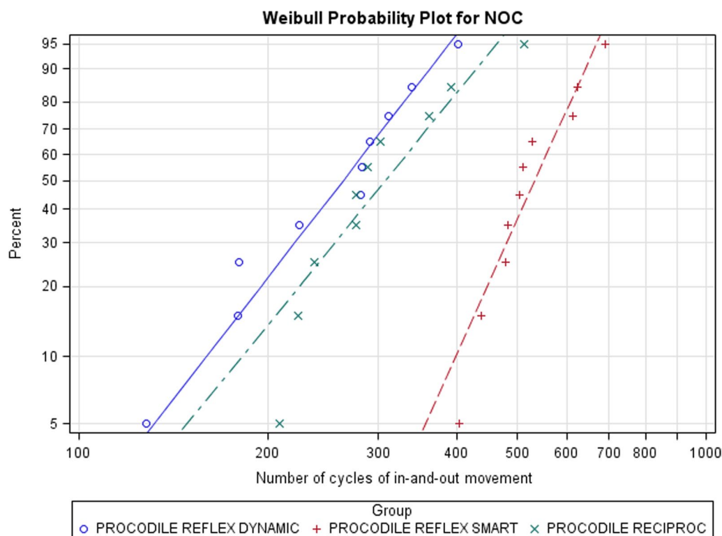
Fig. 5 Weibull probability plot of number of cycles to failure (NOC)
