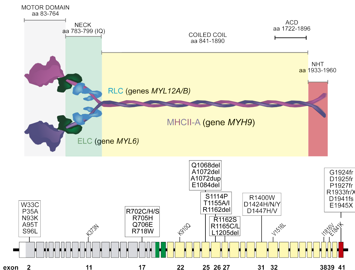
Figure 7: Schematic representation of MYH9 mutations. Top, Color-coded organization of an extended NMII-A hexamer, including the domain organization of MHCII-A, and their binding to ELC (in dark green) and RLC (blue). ACD, assembly-competent domain. NHT, non-helical tailpiece. Bottom, exon organization of the MYH9 gene and position of the most prevalent mutations found in MYH9 -RD patients. Exon organization is color-coded: grey, motor domain; green, neck; yellow, coiled coil; red, NHT. Figure and footnote modified from (Asensio-Juárez et al., 2020).
