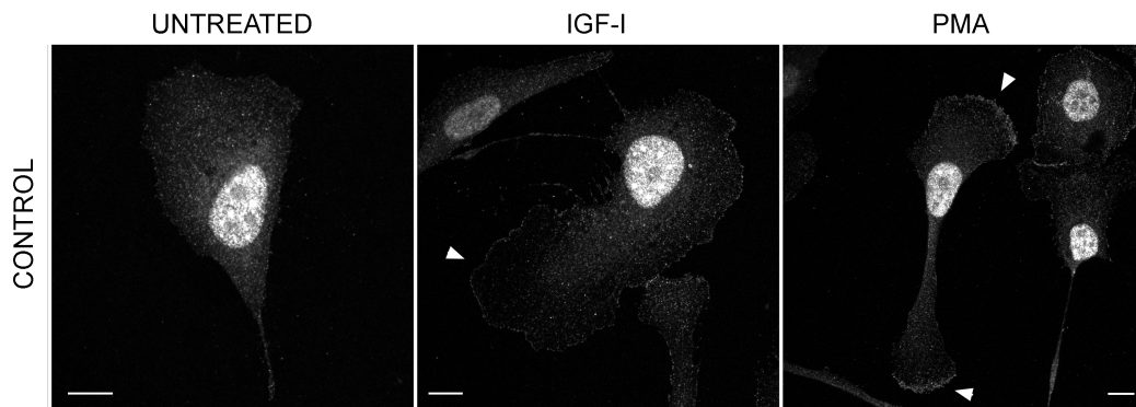
Figure 19: Y155-phosphorylated RLC and the phospho-mimetic mutant Y155E preferentially localizes to the leading edge of polarized cells. Representative confocal images of CHO.K1 cells spread on fibronectin, serum-starved for 16h, then treated with IGF-I (100 ng/ml) or PMA (20 ng/ml) for 10 min, fixed and stained with the pY155 antibody. Bars=10 \mu m.
