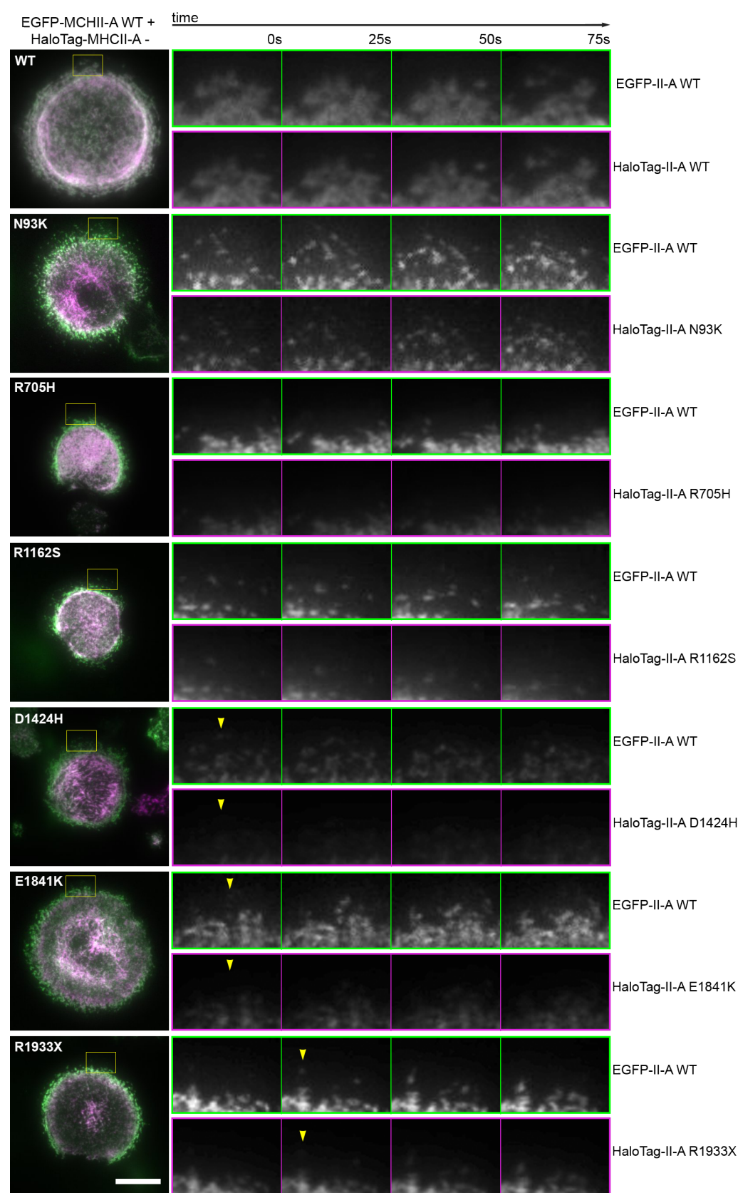
Figure 31: Nucleation of NMII-A and MYH9 mutants in post lamellipodial regions. (See caption next page).
