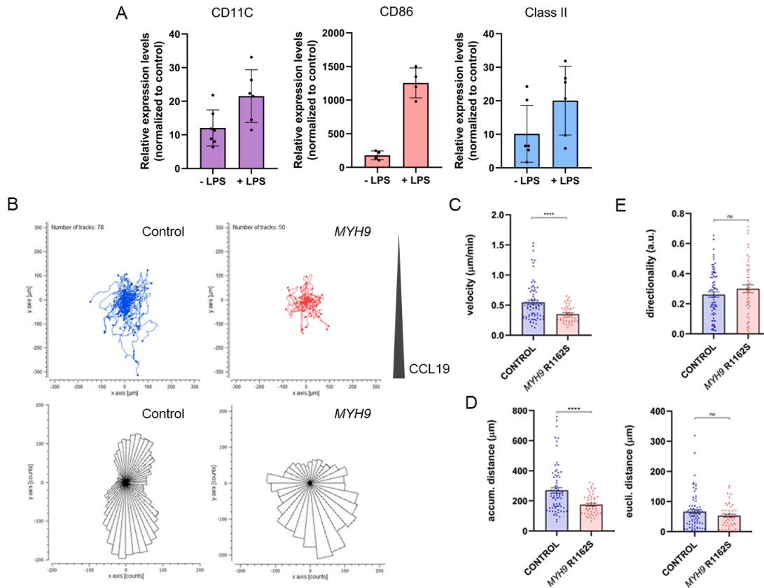
Figure 38: MYH9-R1162S decreases dendritic cell migration speed in 3D collagen gels. (A) Relative surface expression levels of class marker CD11c and maturation markers CD86 and Class II in control mDCs with or without LPS stimulation. Quantification of four independent experiments. (B) Top, data represent the indicated number of tracks and cells' trajectories from each condition. Bottom, rose-plot diagrams of mDCs migration on a CCL19 gradient. N= 78 cells (control) and 50 cells (MYH9) (C) Average migratory velocity, (D) accumulated distance (left panel) and Euclidean distance (right panel), and (E) directionality were calculated using Ibidi's Chemotaxis and Migration Tool from the migratory tracks. Data are the mean \pm SEM. Both mDCs migrate towards CCL19, but MYH9 R1162S mDCs migrate slower, and slightly more persistently. Nonparametric Mann-Whitney U test was used to evaluate statistical significance of control vs MYH9 R1162S-mDCs. **** p < 0.0001 ; n.s., not significant.
