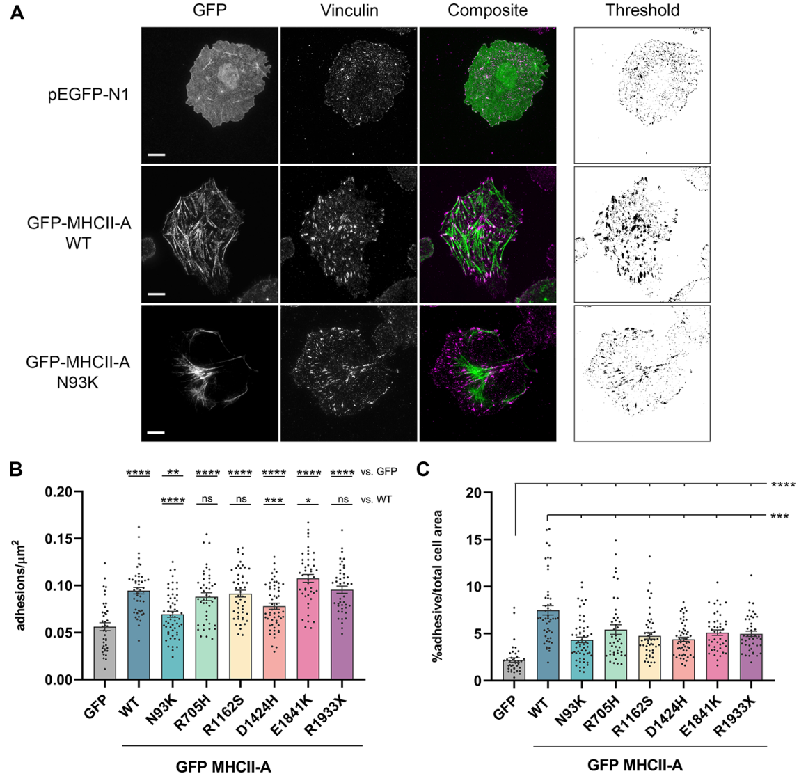
Figure 27: Most NMII-A mutants support adhesion assembly but do not enable efficient adhesion growth. (A) Representative TIRF images of COS-7 cells transfected with EGFP alone, EGFP-MHCII-A WT or the mutants, only N93K mutant is depicted here for illustration. 48h post-transfection, cells were allowed to adhere on fibronectin substrates (3 \mu\text{g}/\text{ml} ) for 150 minutes, fixed and stained for vinculin. Right column shows an example of the threshold used to calculate adhesive area. Scale bar= 10 \mu\text{m} . (B) Quantification of the number of adhesions per \mu\text{m}^2 and (C) the adhesive area of COS-7 cells transfected as in (A). Data are the mean \pm SEM of approximately 40 cells/condition from three independent experiments. Statistical significance of EGFP-MHCII-A vs. EGFP and EGFP-MHCII-A WT vs EGFP-MHCII-A mutants was addressed with unpaired t test for the adhesion/ \mu\text{m}^2 data, and Mann-Whitney U test for the adhesive area. * p < 0.05 ; ** p < 0.01 ; *** p < 0.001 , **** p < 0.0001 , n.s., not significant.
