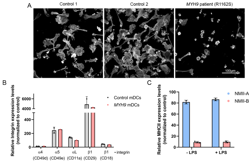
Figure 36: MYH9-R1162S dendritic cells exhibit deficient adhesion on fibronectin. (A) Representative fluorescent images of mDCs allowed to adhere for 40 mins on fibronectin-coated coverslips, fixed, and stained with phalloidin. mDCs carrying R1162S variant adhered less to fibronectin than control mDCs. Bar = 100 \mu m. (B) Relative surface expression levels of the indicated integrins by flow cytometry. Fluorescence levels were normalized to the fluorescent levels of unstained control samples. (C) Relative expression levels of MHCII-A (blue) and MHCII-B (red) in immature and mature mDCs. MHCII fluorescence levels were normalized using the fluorescent levels of control samples incubated only with secondary antibody. Quantification of at least two independent experiments.
