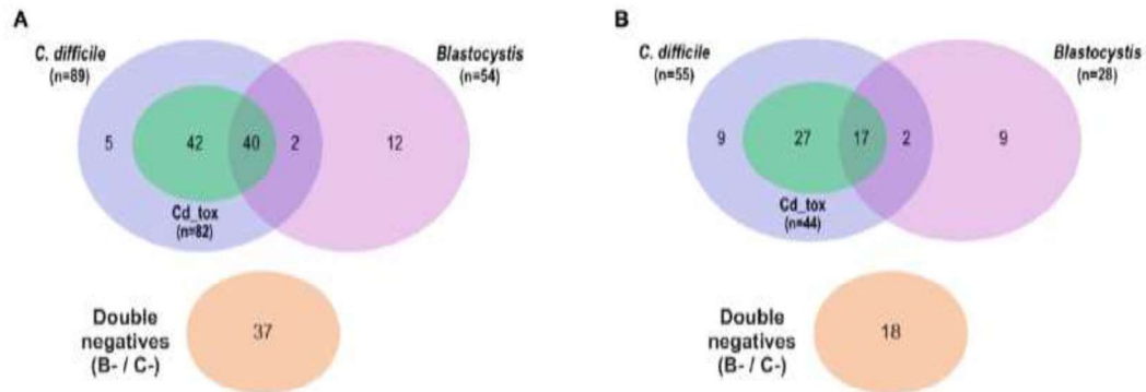
Figure 1. Infection frequencies by Blastocystis and C. difficile within onset groups: (A) Number of community-onset (CO) patients with C. difficile infection (CDI), positive toxigenic C. difficile (Cd_tox), and presence of Blastocystis and patients negative for both microorganisms. (B) Number of healthcare facility-onset (HCFO) patients with C. difficile infection (CDI), positive toxigenic C. difficile (Cd_tox), and presence of Blastocystis and patients negative for both microorganisms.
