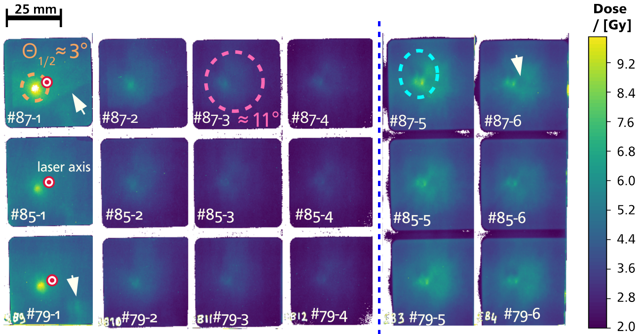
FIGURE 6.25: Overview on RCF results for shots #79, #85 and #87 with a respective transverse nozzle displacement of 0\text{ }\mu\text{m} , -50\text{ }\mu\text{m} and +50\text{ }\mu\text{m} as 2D dose maps. For display purpose, data is averaged over the three colour channels. RCF layers are numbered in ascending order in direction of particle propagation. The laser axis is indicated with a white dotted marker, its size represents the alignment uncertainty to the laser axis in air pressure. The unlaminated EBT-3 films used for both last layers were likely exposed to conditions, after their calibration and prior to the experiment, that changed their response to dose-deposition with respect to the calibrated response. This is clear from their detection of dose in the area blinded by the detector casing, which is blank on the first layers. Image taken from [75].
