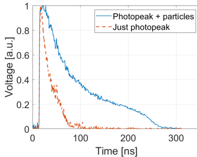
FIGURE 6.16: Comparison between the detector raw signal comprising the extended photopeak and all accelerated particle species (blue full line) and a signal with the extended photopeak only (orange dashed line). Data taken from [75].
