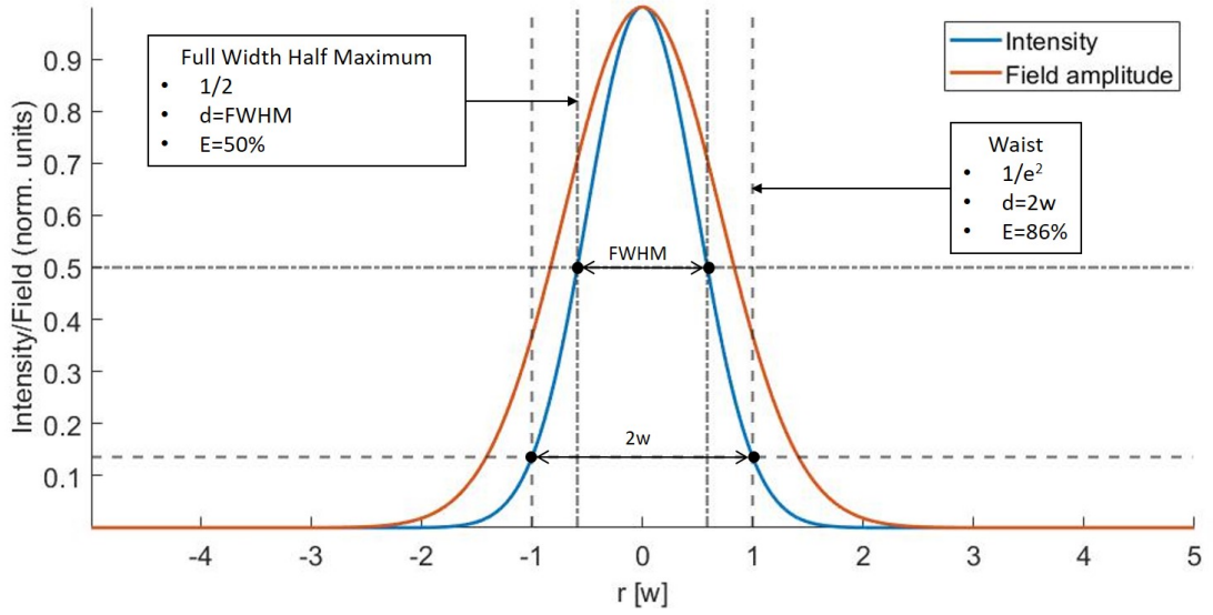
FIGURE 3.5: Gaussian beam field amplitude and intensity profiles. Widths definitions for 1/e^2 and FWHM.
