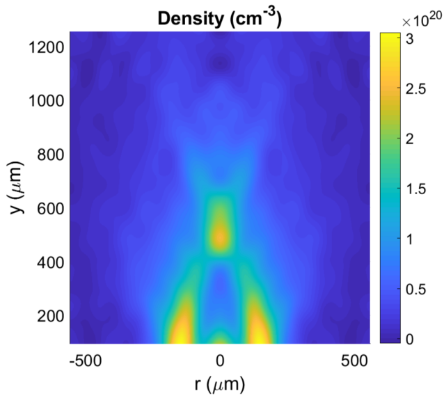
(A) Molecular density map retrieved from the interferogram in figure 6.5. y = 0 corresponds to the nozzle edge.
