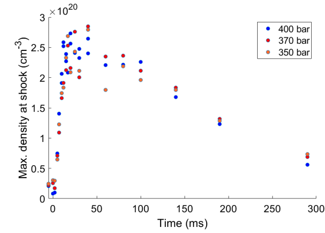
(A) Time evolution of the molecular density of the shock point density for TUCAN nozzle for different backing pressures of Nitrogen.
