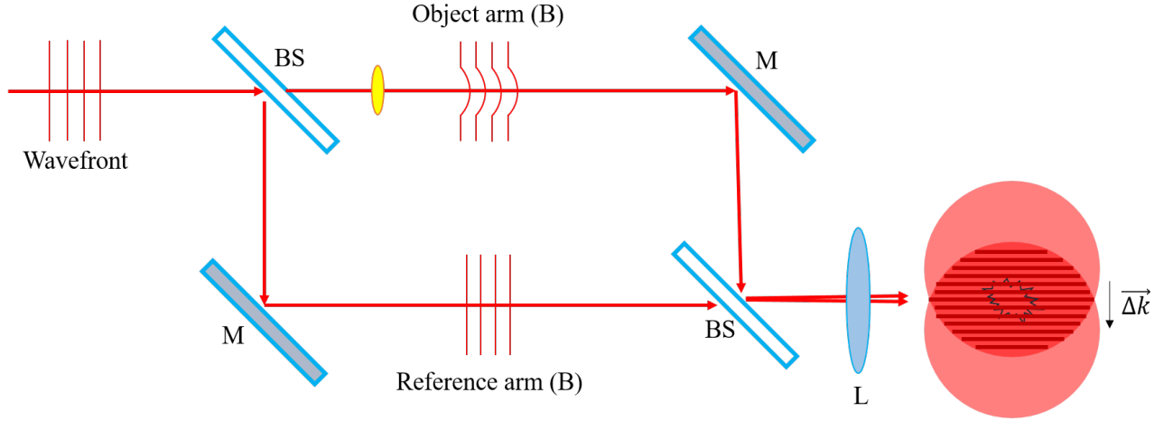
FIGURE 4.4: Basic Mach-Zehnder interferometer operation. M stands for mirrors, meanwhile BS for beams-plitters and L for an imaging lens.
