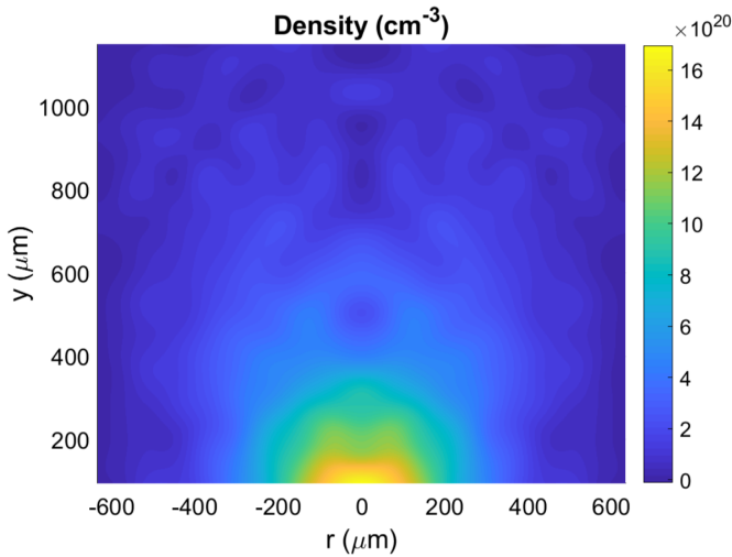
(A) Density map retrieved from interferometric technique of nozzle LOLA.
