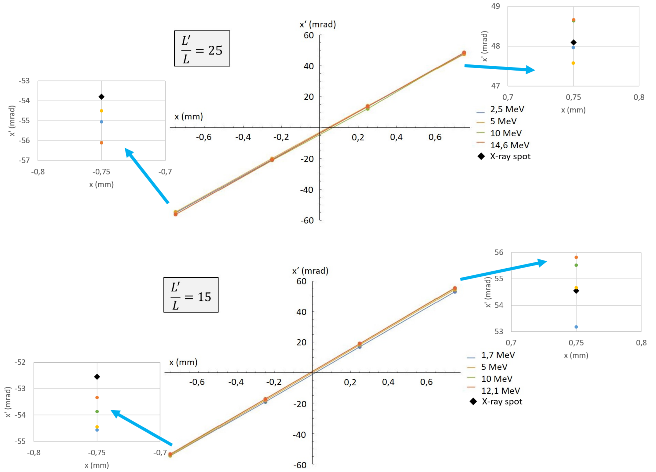
FIGURE 7.19: Representation of the mean divergence values of each beamlet lineout \langle x'_i \rangle (i.e. the trace centroids) in the trace space for both experimental configurations (upper plot: dataset with L'/L = 25 , bottom plot: dataset with L'/L = 15 ). Insets detail the centroids value for the extreme beamlets.
