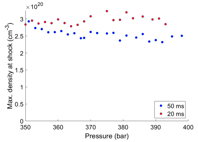
(B) Dependence with pressure of the shock point molecular density for TUCAN fed with Nitrogen, measured at different times after the valve opening.
