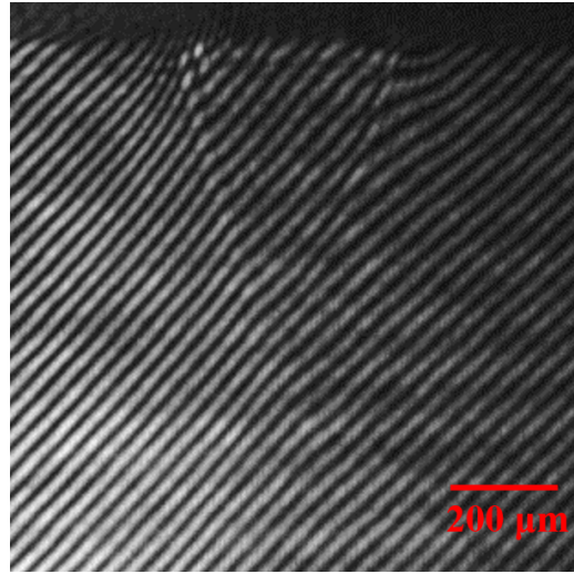
FIGURE 6.5: Typical Nomarsky interferometric picture of a fully developed shock jet (TUCAN, outer orifice diameter 400\text{ }\mu\text{m} ), backed with 400 bars of nitrogen, measured 12 ms after the valve opening.
