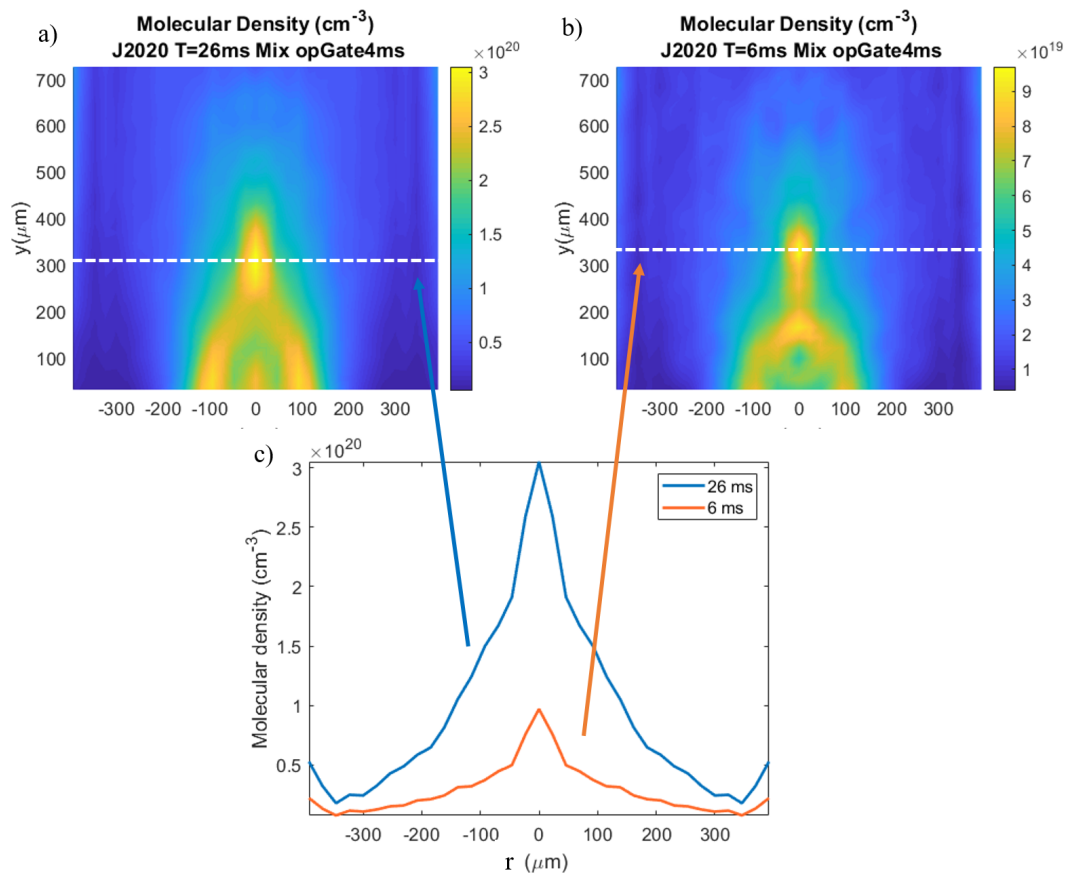
FIGURE 6.32: Density maps comparison of (a) a fully-developed J2020 jet ( \sim 410 bar of 9:1 \text{N}_2 :He mix, valve opening time 4 ms), measured 26 ms after valve trigger and (b) the same jet at early formation stages (6 ms after valve opening). (c) compares both radial density lineouts from (a) and (b).
