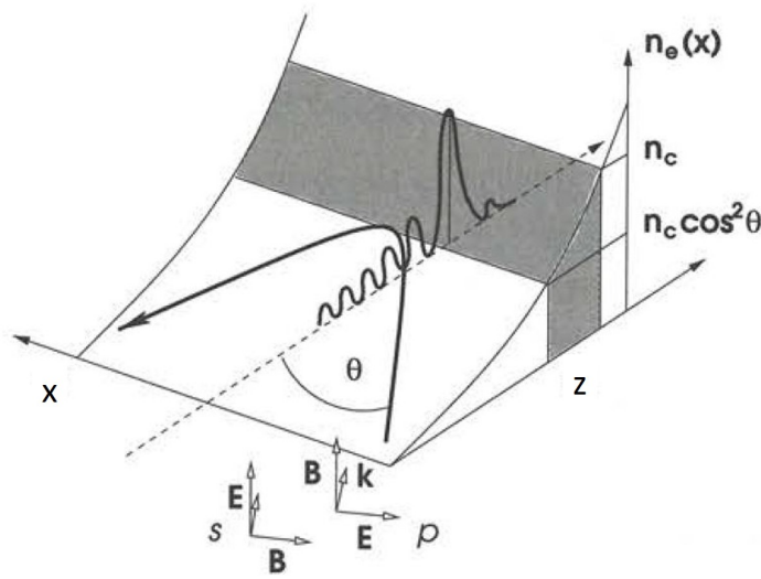
FIGURE 3.22: Geometrical sketch of for p(s)-polarized EM wave, with angle of incidence \theta into a preplasma gradient density from an initially overdense target. Figure adapted from [69].
