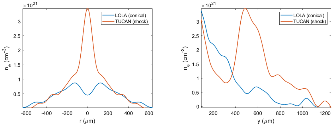
(A) Transversal lineouts of the expected electron density at shock height for TUCAN (shock, orange) and LOLA (conical, blue).
