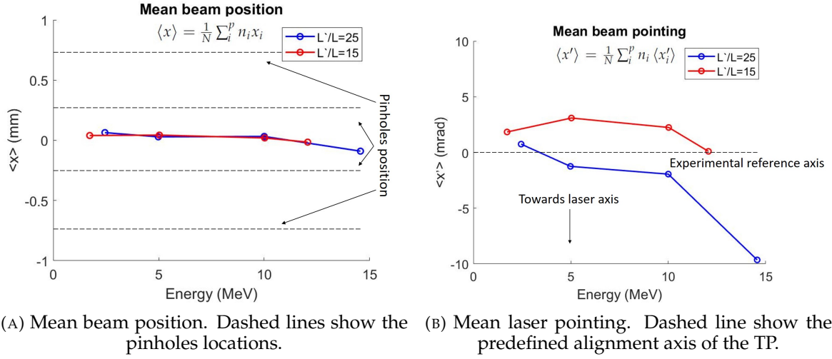
FIGURE 7.17: Energy resolved mean beam position and pointing estimated from trace-space measurement. Insets show the formulae of each term. Their definition is explained in equation 4.26. Blue lines: dataset with L'/L = 25 . Red lines: dataset with L'/L = 15 .
