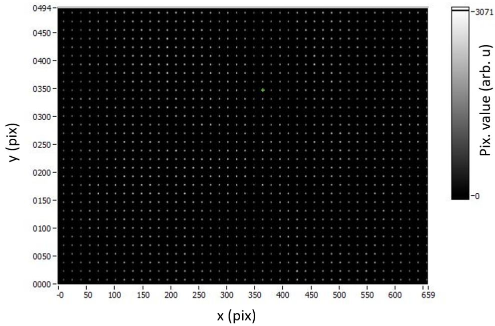
FIGURE 4.16: Typical raw signal from SH wavefront detector. The multiple foci generated by the micro-lenses array can be appreciated. Data taken with HASO4 detector, back-illuminated with a expanded He-Ne laser.
