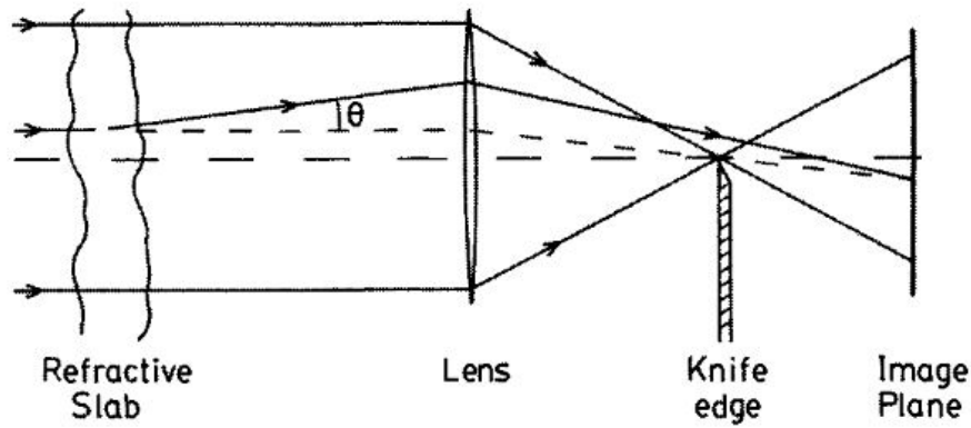
FIGURE 4.18: Working principle of Schlieren imaging. Image taken from [63].
