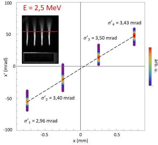
(A) Trace space for the mean energy 2.5 MeV.
