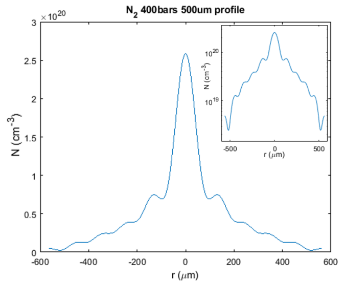
(B) Density lineout at shock height ( 500\text{ }\mu\text{m} ) taken from 6.6a. Inset shows the same lineout in logarithmic scale.
