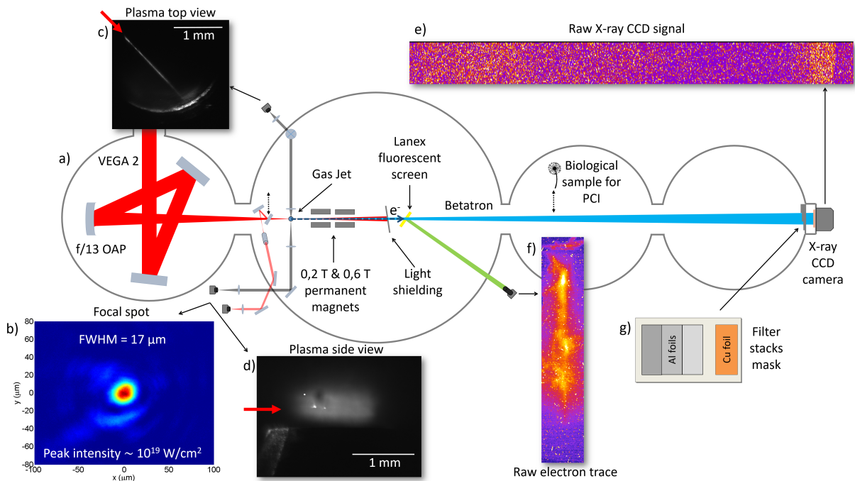
FIGURE 5.12: a) General setup of the LWFA commissioning experiment at VEGA 2. b) Laser focal spot. c) Zenithal plasma image (red arrow points the laser direction). d) Lateral plasma image (red arrow points the laser direction). e) Raw X-ray CCD signal of the Betatron radiation. f) Electron spectral trace measured on Lanex screen. g) Step-filter configuration for Betatron characterization.
