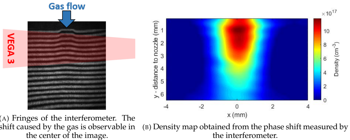
FIGURE 5.16: Typical raw interferometric signal and density map of the rectangular gas jet with 50 bar of Argon.
