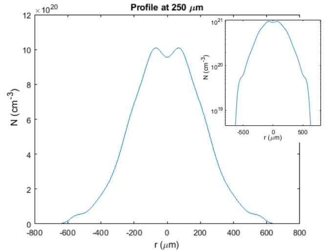
(B) Density lineout at 250 \mu\text{m} from nozzle end taken from 6.8a. Inset shows the same lineout in logarithmic scale.
