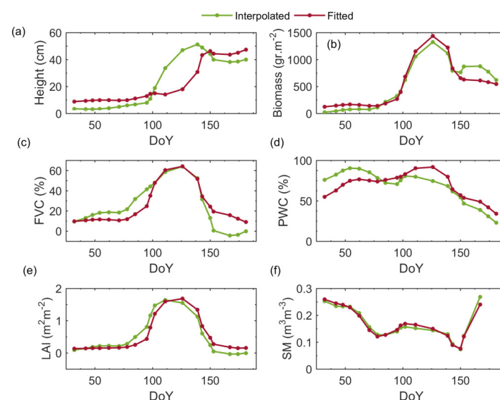
Figure 10. Interpolated real data versus cointegration—adjusted for biophysical variables of M9 plot. (a) Height, (b) Biomass, (c) FVC, (d) PWC, (e) LAI, (f) SM.
