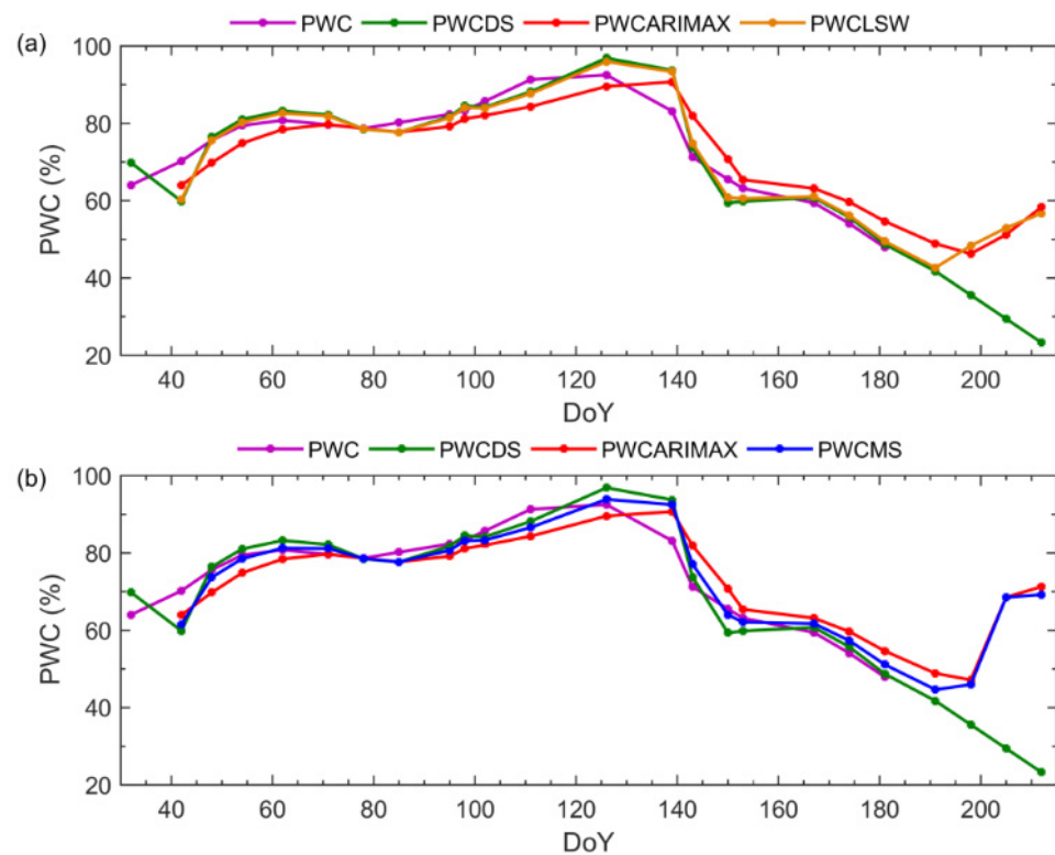
Figure 6. Combination prediction for PWC: (a) weighted least squares; (b) mean squared. PWC: interpolated data; PWCDS: double smoothing; PWCARIMAX: ARIMAX; PWCLSW: weighted least squares; PWCMS: mean squared.
