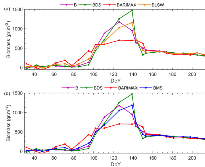
Figure 4. Combination prediction for biomass: (a) weighted least squares; (b) mean squared. B: interpolated data; BDS: double smoothing; BARIMAX: ARIMAX; BLSW: weighted least squares; BMS: mean squared.
