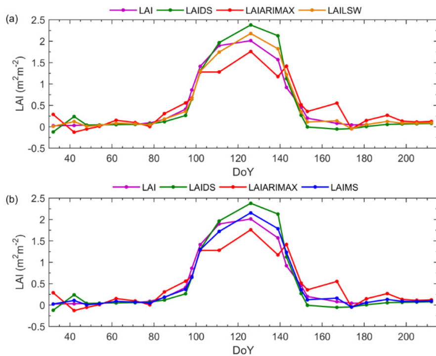
Figure 7. Combination prediction for LAI: (a) weighted least squares; (b) mean squared. LAI: interpolated data; LAIDS: double smoothing; LAIARIMAX: ARIMAX; LAILSW: weighted least squares; LAIMS: mean squared.
