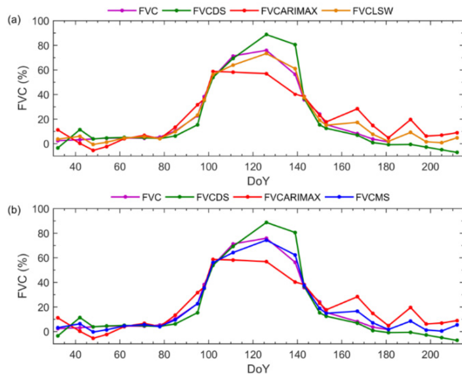
Figure 5. Combination prediction for FVC: (a) weighted least squares; (b) mean squared. FVC: interpolated data; FVCDS: double smoothing; FVCARIMAX: ARIMAX; FVCLSW: weighted least squares; FVCMS: mean squared.
