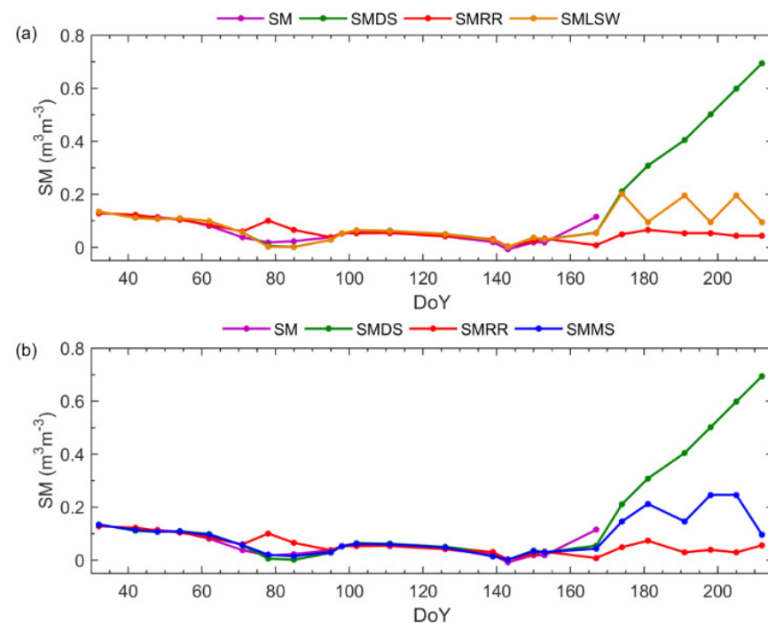
Figure 8. Combination prediction for soil moisture: (a) weighted least squares; (b) mean squared. SM: interpolated data; SMDS: double smoothing; SMRR: robust regression SMLSW: weighted least squares; SMMS: mean squared.
