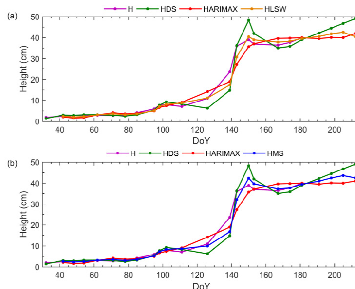
Figure 3. Combination prediction for height: (a) weighted least squares; (b) mean squared. H: interpolated data; HDS: double smoothing; HARIMAX: ARIMAX; HLSW: weighted least squares; HMS: mean squared.
