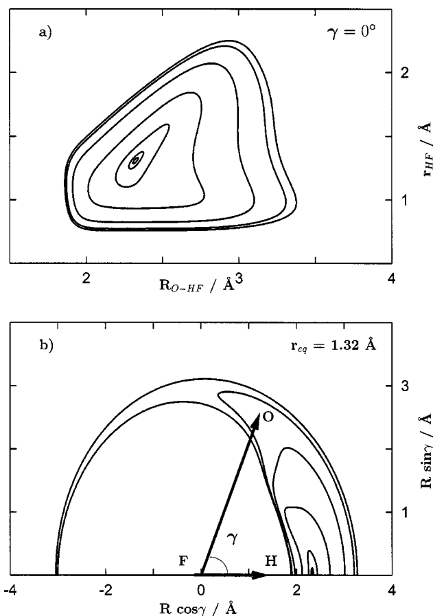
FIG. 2. Contour plots of the local OHF - ( 2 A') PES in product Jacobi coordinates for (a) \gamma=0 , (b) r=1.32 Å, with x=R \cos \gamma and y=R \sin \gamma . The contours correspond to 0.002, 0.01, 0.1, 1, 5, 10, and 12 eV.
