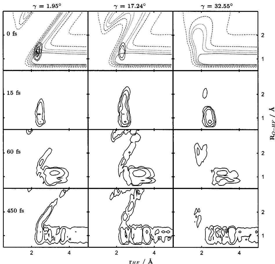
FIG. 4. Contour plots of the wave packet density for different times and angles in the product Jacobi coordinates. The propagation is performed on the OHF( ^3A'' ) PES to simulate the J'=1 \leftarrow J=0 . The contours of the potential correspond to 3.5, 1.5, 0.5, 0, -0.5 eV with respect to OH( v=0 ) + F.
