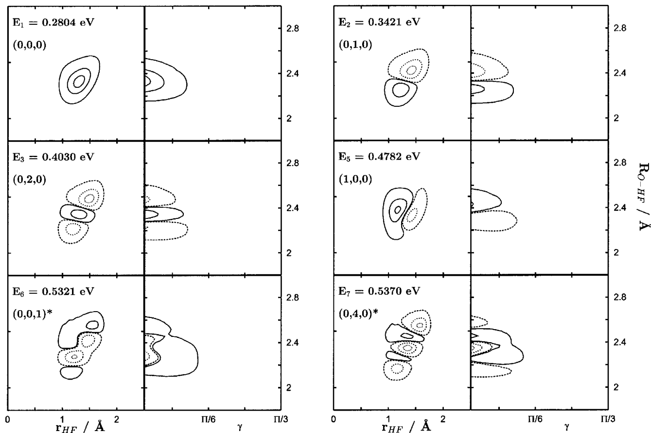
FIG. 3. Contour plots of the wave function amplitude for several vibrational bound states of \text{OHF}^-(^2A') in product Jacobi coordinates for \gamma=0 (left panels) and for r=1.32 Å (right panels). The energies, E_k of the k level are in eV, and the approximate (v,n,b) quantum numbers are given. Solid (dashed) lines correspond to positive (negative) amplitudes. The levels marked with an asterisk interact strongly.
