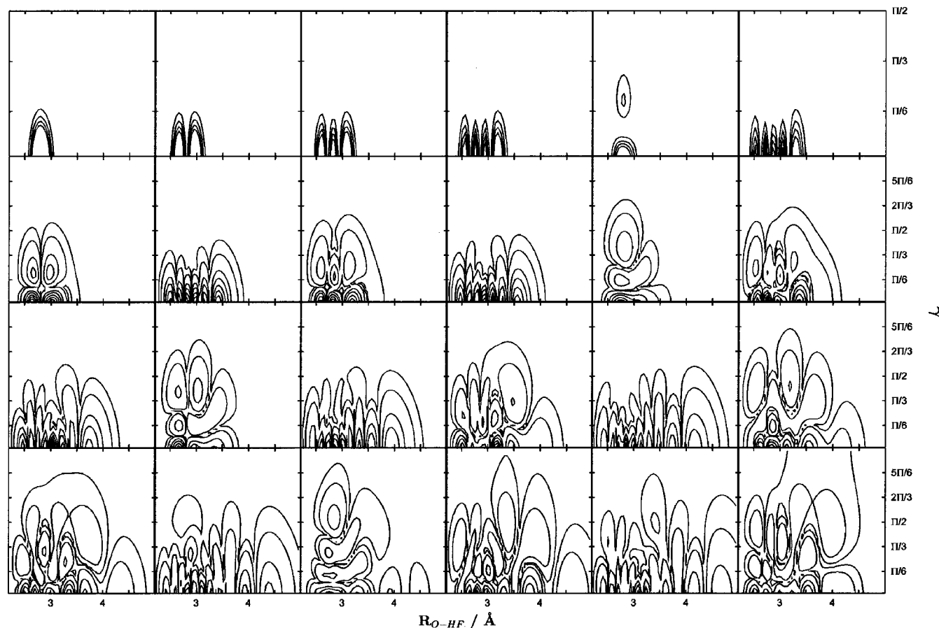
FIG. 9. Contour plots of the amplitude density of the quasibound states, for r frozen at the HF equilibrium distance, obtained for O-HF( v=1 ).
