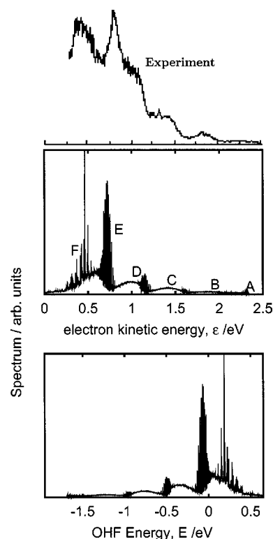
FIG. 5. Spectrum obtained for the J'=1 \leftarrow J=0 transition. Bottom panel, as a function of the OHF energy. Central panel, as a function of the electron kinetic energy, using \epsilon = 0.65 - E in eV. The factor 0.65 has been fitted, since the dissociation energy of the OHF ^- was not calculated. Top panel, experimental spectrum from Ref. 21.
