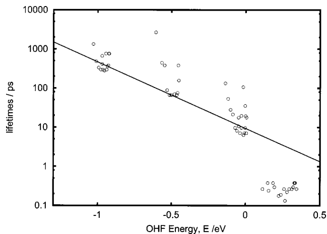
FIG. 11. Resonance lifetimes (in ps) as a function of energy (in eV), as obtained by doing individual fits to a Lorentzian function in the vicinity of the rather well isolated resonances of the spectrum calculated with the TICC in rather fine energy grid.
