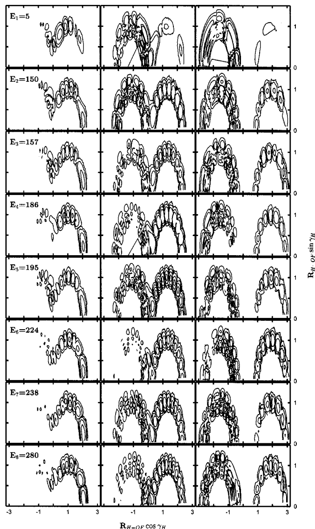
FIG. 14. Contour plots of the density probability of several HLH resonances. The energy of the resonances are in meV, distances are in Å, and three contours are chosen with an order of magnitude of density probability difference, to distinguish the wave functions structures. Left panels for r_{\text{OF}} = 1.965 Å, middle panels for r_{\text{OF}} = 2.4 Å, and right panels for r_{\text{OF}} = 3.5 Å.
