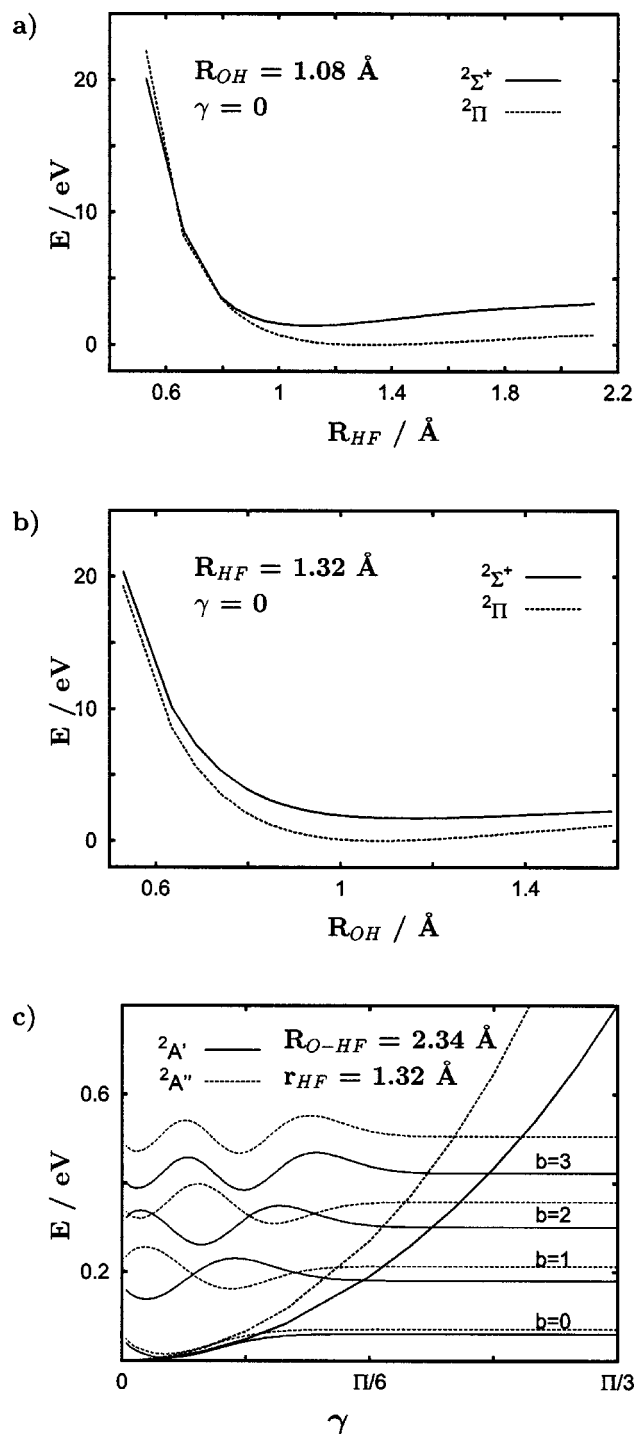
FIG. 1. Calculated ab initio energy points for several electronic states of the OHF - anion. On each panel fixed geometric parameters are equilibrium values. On panel (c) the two potential curves, of 2 A' (solid line) and 2 A'' (dashed line) states, are plotted together with their corresponding monodimensional bending levels, b .
