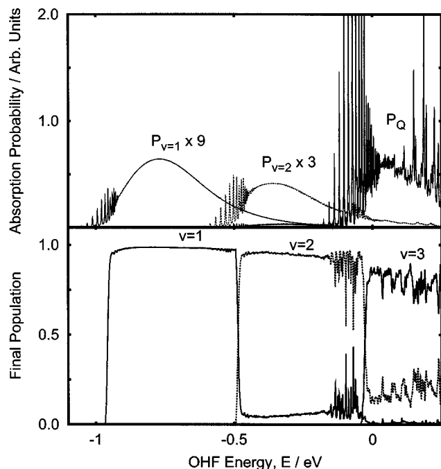
FIG. 6. Top panel, absorption probabilities obtained for the different portions of the wave packets applying the projection operators of Eq. (7). Bottom panel final \text{HF}(v) vibrational distribution. Energy scale, in eV, is referred to the \text{F} + \text{OH}(v=0) threshold.
