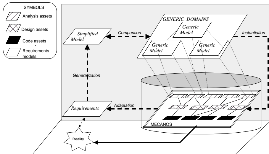
Fig. 5. Generic requirements as the key to mecano reuse
