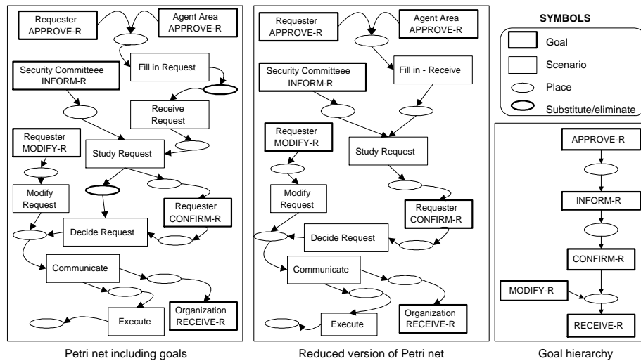
Fig. 6. Reduction of the Petri net of a request processing system
