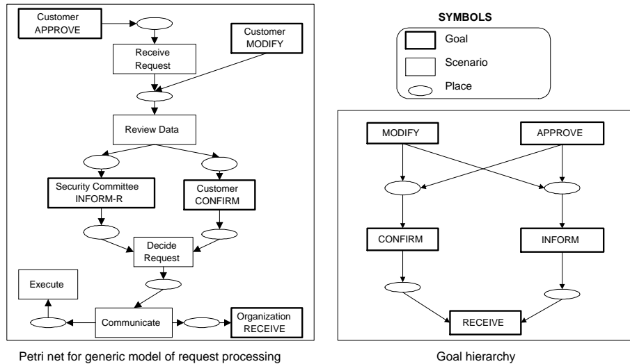
Fig. 7. A generic model for the domain of request processing
