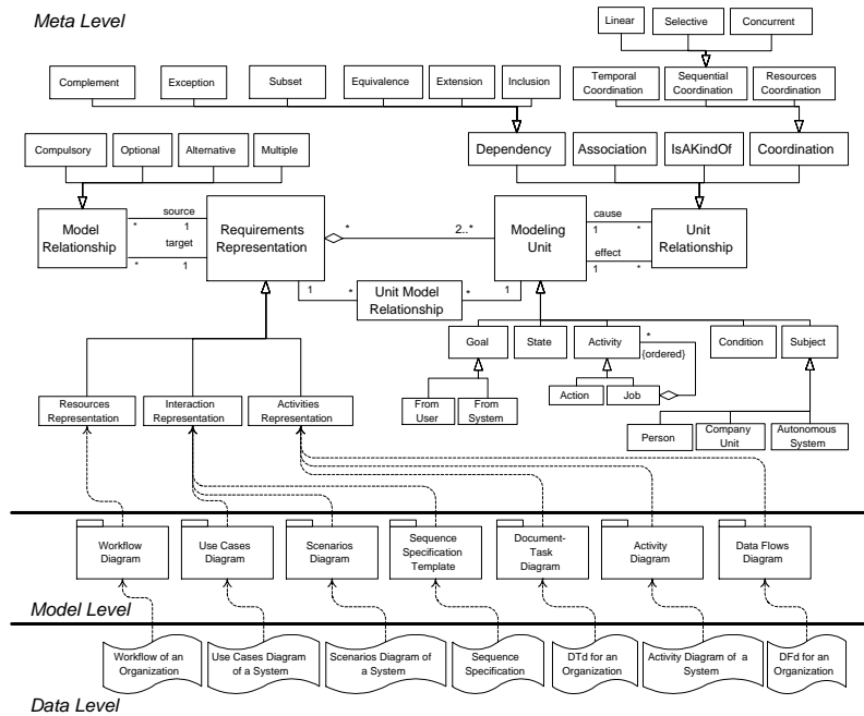
Fig. 3. Metamodel of Software Requirements Representations, expressed in UML. The requirements are represented by Modeling Units related to each other and with Requirements Representations that are also related to each other.
