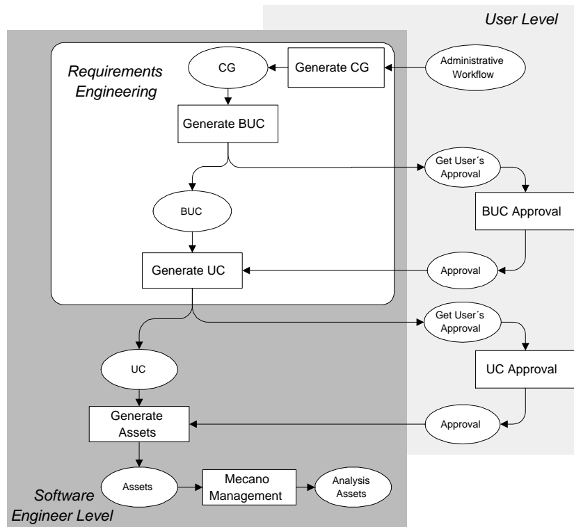
Fig. 2. General framework for the standardization of user requirements capture
