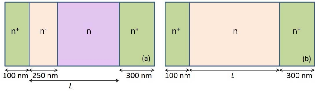
FIGURE 1. Geometry of the studied structures with physical dimensions. (a) Diode with a 250 nm-length notch placed next to the cathode and (b) diode without notch. The lengths of n^+ contact regions are 100 nm and 300 nm at the cathode and anode, respectively, in both structures. n^+=2\times 10^{18} \text{ cm}^{-3} , DS1: n=1\times 10^{17} \text{ cm}^{-3} and n=2\times 10^{16} \text{ cm}^{-3} and DS2: n=5\times 10^{17} \text{ cm}^{-3} and n=1\times 10^{17} \text{ cm}^{-3} . Four different lengths, L=1500, 1200, 900 and 750 nm have been simulated.
