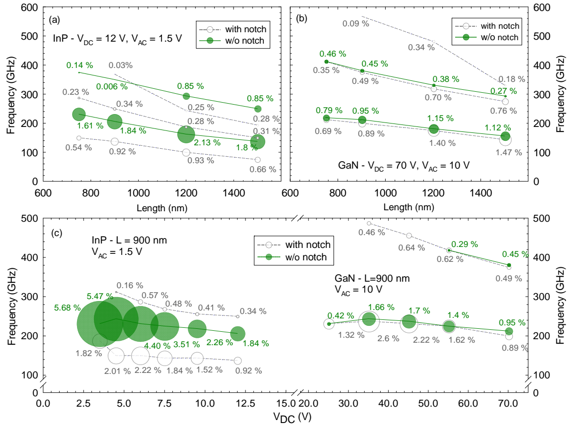
FIGURE 6. FME and corresponding efficiency of the different generation bands found in diodes with the DS1 with and without notch. The size of the bubbles scales with the maximum of the DC to AC conversion efficiency, \eta , indicated for the different generation bands. The dependence on the length of the active region is shown for (a) InP diodes using V_{DC}=12 V and V_{AC}=1.5 V and (b) GaN diodes using V_{DC}=70 V and V_{AC}=10 V. (c) Dependence on the DC bias for L=900 nm and using and AC excitation of V_{AC}=1.5 V for InP and V_{AC}=10 V for GaN.
