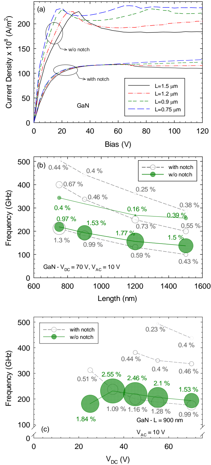
FIGURE 8. Results in a GaN diode (with and without notch) when the DS2 is considered. (a) I-V curves for different lengths of the active region: L=1500 \text{ nm} , 1200 \text{ nm} , 900 \text{ nm} and 750 \text{ nm} . Dependence of the FME and corresponding efficiency of the different generation bands on the (b) length of the active region ( V_{DC}=70 \text{ V} and V_{AC}=10 \text{ V} ) and (c) DC bias for L=900 \text{ nm} and using V_{AC}=10 \text{ V} . The size of the bubbles scales with the maximum of the DC to AC conversion efficiency, \eta , and is indicated for the corresponding generation band.
