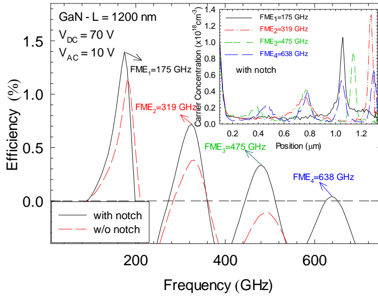
FIGURE 7. DC to AC conversion efficiency vs. frequency for GaN-based diodes (with and without notch) with L=1200 nm and for the DS1. Single-tone excitation with V_{DC}=70 V and V_{AC}=10 V. The inset shows the profile of carrier concentration along the diode corresponding to a given time within one period of the AC signal for frequencies at the maximum of the emission bands to be FME=175, 318.7, 475 and 637.5 GHz.
