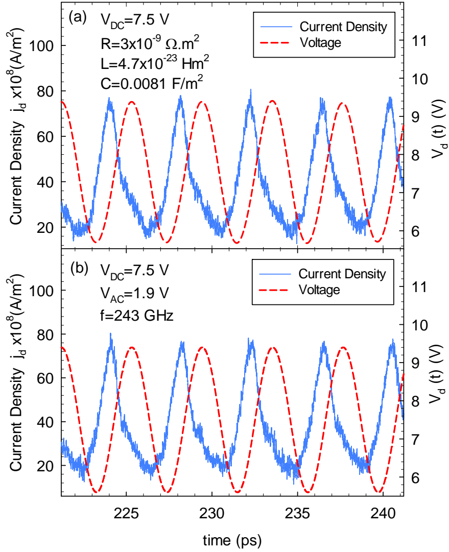
FIGURE 3. Time-sequences of current density j_d and applied voltage V_d(t) in a InP n^+nn^+ diode using the DS1 and V_{DC}=7.5 V. (a) Resonant RLC circuit in series with the diode ( R=3 \times 10^{-9} \Omega \text{m}^2 , L=4.7 \times 10^{-23} Hm 2 , and C=0.0081 F/m 2 ) and (b) excitation by means of a single-tone of frequency 243 GHz and V_{AC}=1.9 V [Eq. 3].
