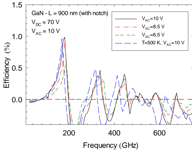
FIGURE 9. DC to AC conversion efficiency vs. frequency for a GaN-based diode with notch with L=900 nm and for the DS2 and with V_{DC}=70 V. The AC excitation used are V_{AC}=10 V, 8.5 V and 6.5 V. Also results T=500 K are presents ( V_{AC}=10 V).
