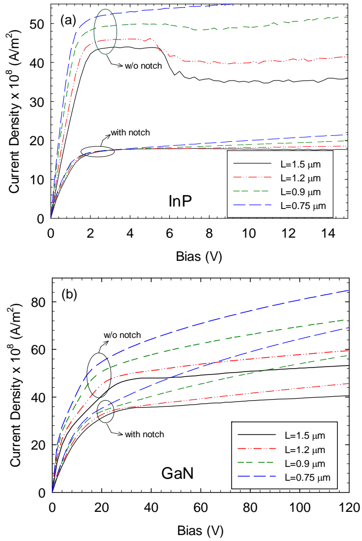
FIGURE 4. I - V curves for the two types of diodes, with and without notch, and for different lengths of the active region: L=1500 nm, 1200 nm, 900 nm and 750 nm for the DS1 and for (a) InP and (b) GaN.
