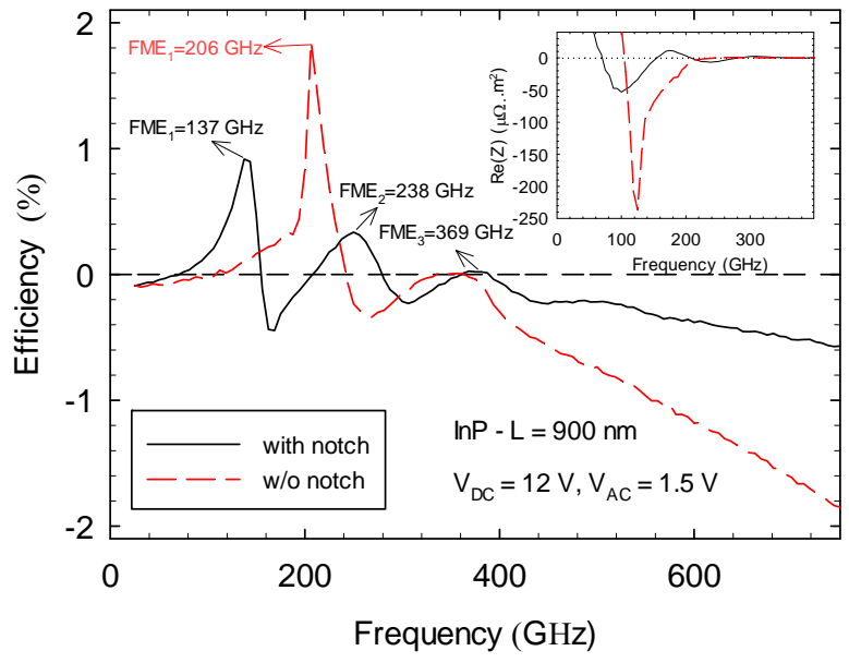
FIGURE 5. DC to AC conversion efficiency vs. frequency for InP-based diodes (with and without notch) with L=900 nm and for the DS1. Single-tone excitation with V_{DC}=12 V and V_{AC}=1.5 V. The inset shows the real part of the impedance.
