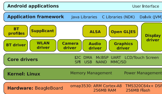
Figure 17: Android architecture over Beagleboard
