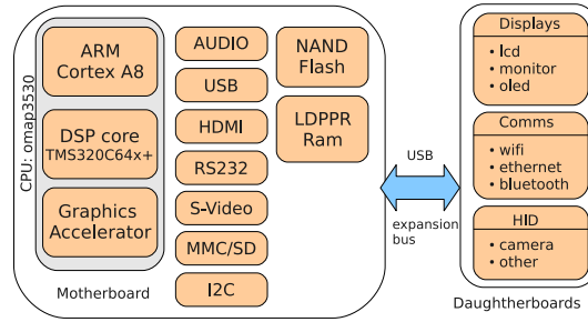
Figure 16: Hardware of Beagleboard
