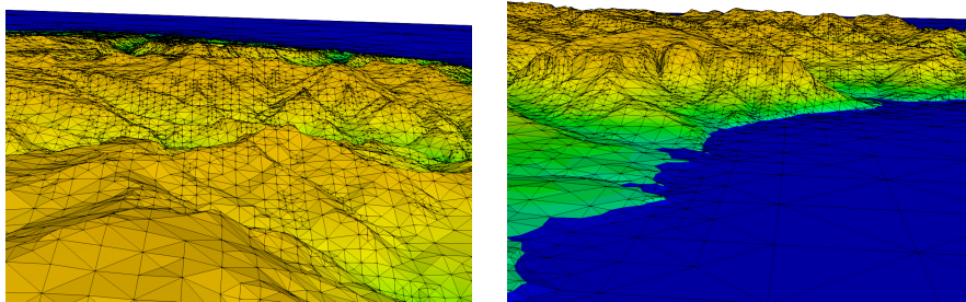
Figure 9: Surface of the final mesh of Gran Canaria Island, for \varepsilon = 50m. , and several details
