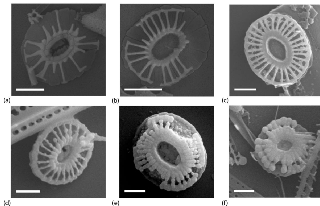
Plate 1. SEM photos showcasing the different morphologies of Emiliana huxleyi morphotype B/C coccoliths found in the sediment traps of the 61° S site. Scale bars = 1 \mu m.
