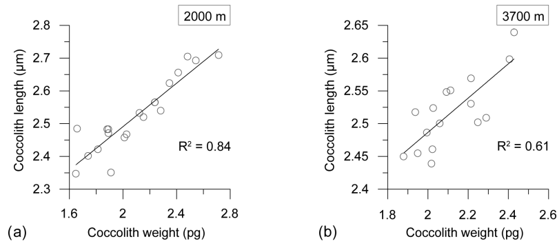
Figure 7. Regression plots between E. huxleyi coccolith mass (pg) and length (µm) at the 2000 m (a) and 3700 m (b) sediment traps.
