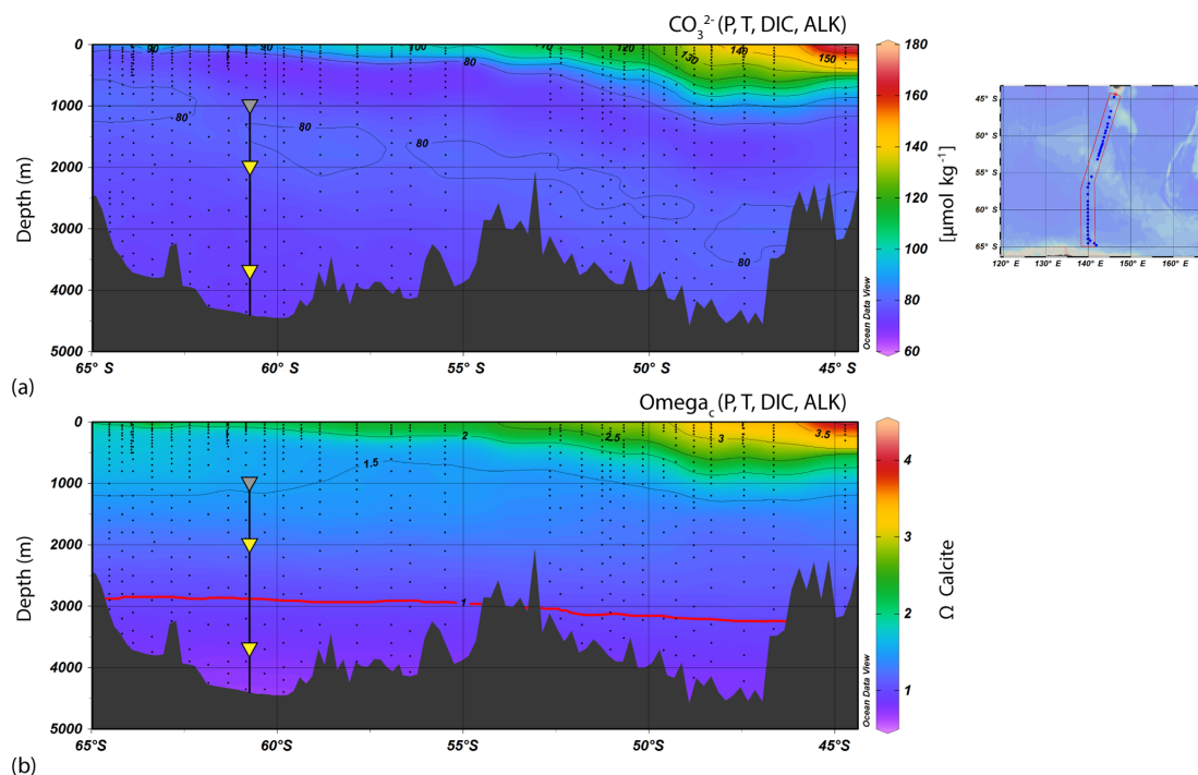
Figure 3. Cross section of the mooring location in comparison to regional sea-floor bathymetry, carbonate concentrations [ \text{CO}_3^{2-} ] and calcite saturation ( \Omega_{\text{calcite}} ) for WOCE transect SR03 2001 from Bostock et al. (2011), who calculated them from the dissolved inorganic carbon (DIC) and alkalinity in the CARINA database (CARINA group, 2011). The location of the transects is shown on the map on the right top. The \Omega_{\text{calcite}} = 1 contour is highlighted with a red line to show the approximate depth of the CSH across the transect.
