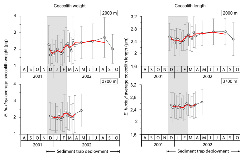
Figure 6. Mean and standard deviation of coccolith weight and length over the sediment trap deployment period at 2000 and 3700 m at the 61° S site. The solid red line represents a three-point running average. Grey strips represent summer.
