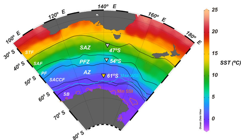
Figure 1. Annual mean sea surface temperature map (World Ocean Atlas; Locarnini et al., 2013) of the Australian sector of the Southern Ocean, showing the position of the main frontal and zonal systems (adapted from Orsi et al., 1995) and the location of the 61, 54 and 47° S sediment trap stations (inverted triangles). Abbreviations: STF – subtropical front, SAZ – Subantarctic zone, SAF – Subantarctic Front, PFZ – Polar Frontal Zone, PF – Polar Front, AZ – Antarctic zone, SACCFC – Southern Antarctic Circumpolar Current Front, SB – southern boundary, Max WSI – maximum winter sea ice extent (August 2001) and Min SSI – minimum summer sea ice extent (February 2002; Fetterer et al., 2017).
