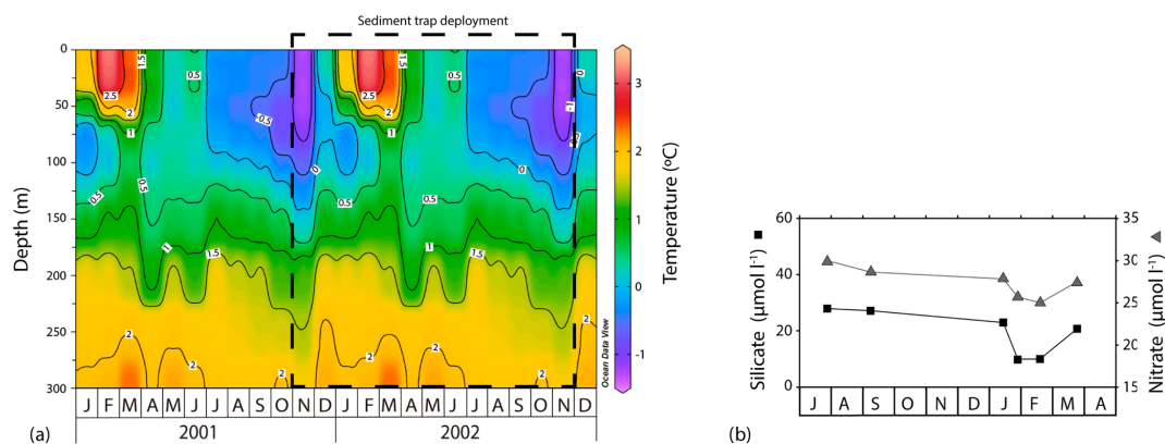
Figure 2. (a) Seasonal variation in the vertical structure of temperature ( ^{\circ}\text{C} ) between January 2001 and December 2002 for the 61^{\circ}\text{S} site from the World Ocean Atlas 2009 (Locarnini et al., 2010). (b) Summary of seasonal evolution of macronutrient concentrations (silicate and nitrate) in the mixed layer at the 61^{\circ}\text{S} site taken from the WOCE SR3 transects between 1993 and 1996 (modified from Trull et al., 2001b).
