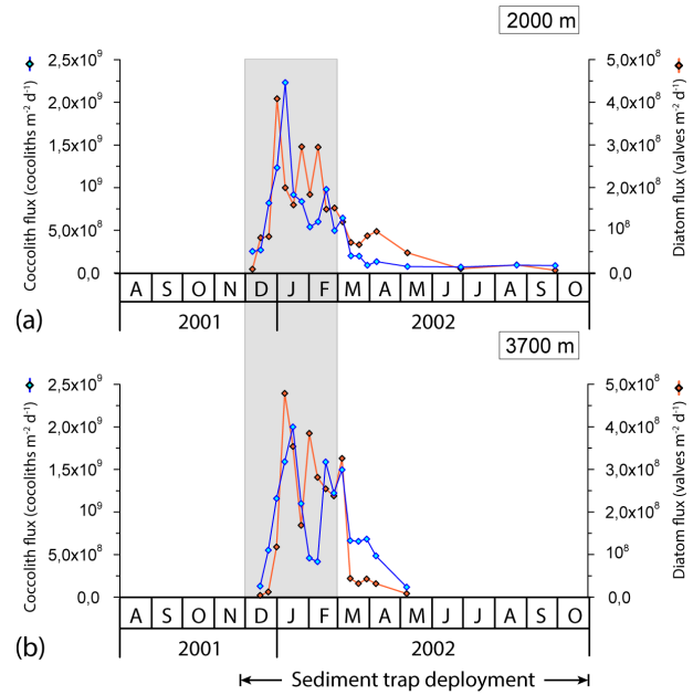
Figure 5. Seasonal variation in total coccolith and diatom valve flux at the 2000 and 3700 m sediment traps at the 61° S site. Grey strips represent summer.
