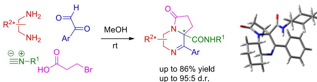
Fig. 1: Synthesis of Enantiopure Pyrroloperazines
