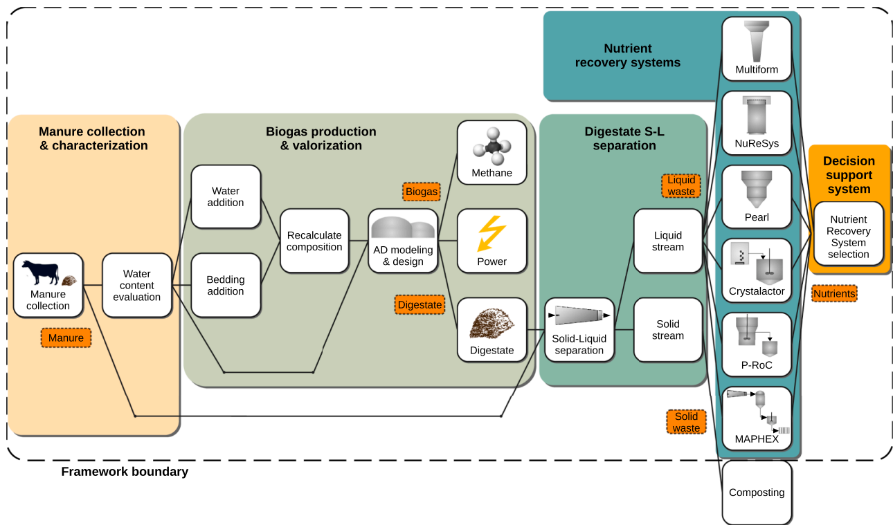
Fig. 2. Process flowsheet for manure management and phosphorus recovery stages included in COW2NUTRIENT.
