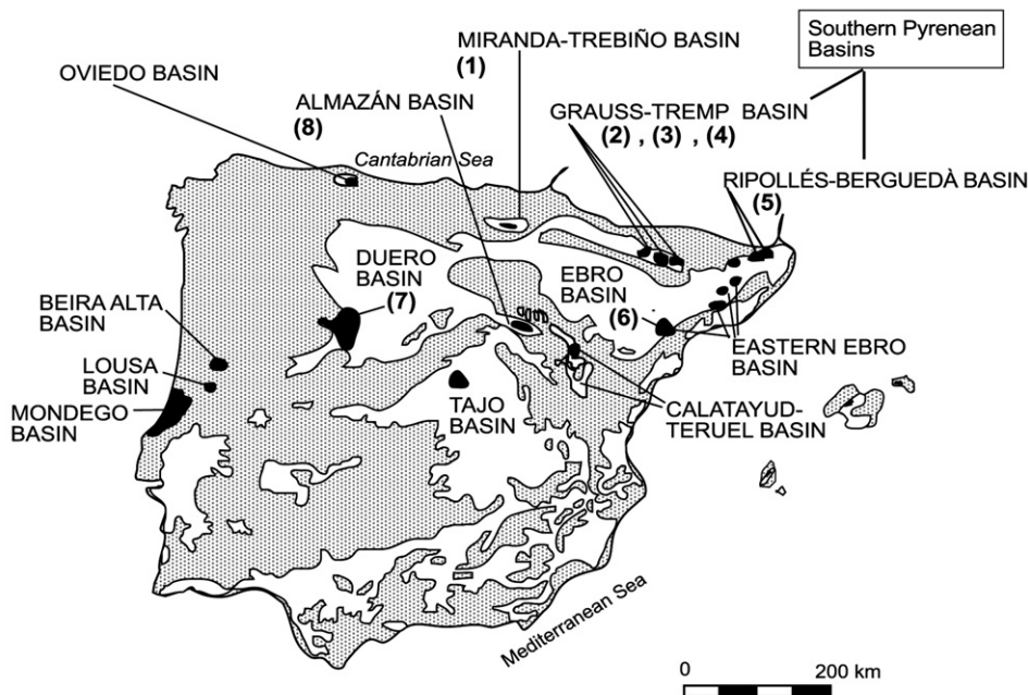
Iberian Tertiary basins with ■ Eocene mammal sites
