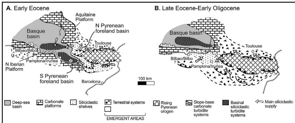
FIGURE 5 Paleogeography of the Pyrenean and Basque-Cantabrian region during the Early Eocene (A) and Late Eocene-Early Oligocene (B). Modified from Alonso-Zarza et al., 2002 after Plaziat, 1981.
